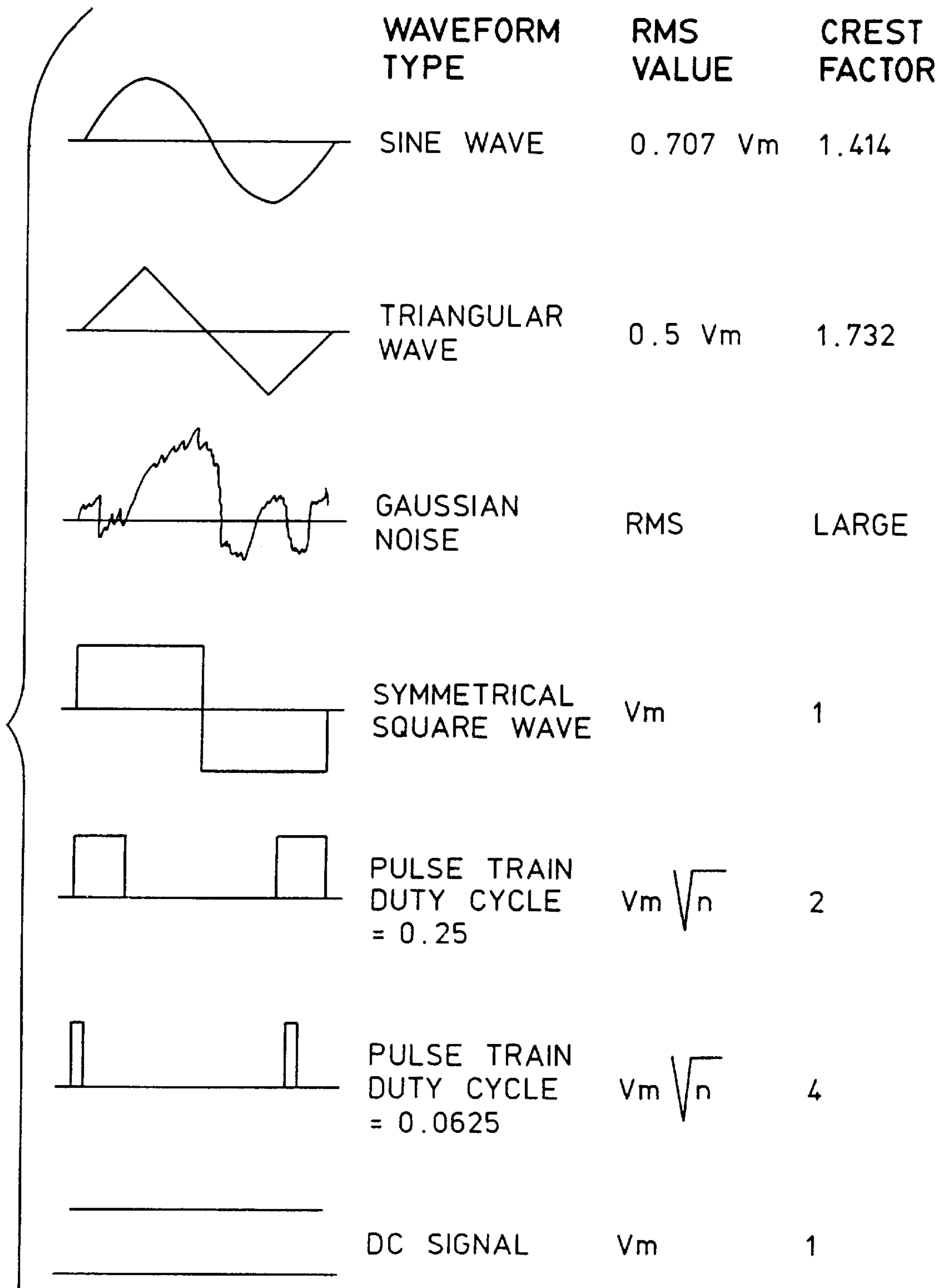
RMS AND CREST FACTOR CHART
