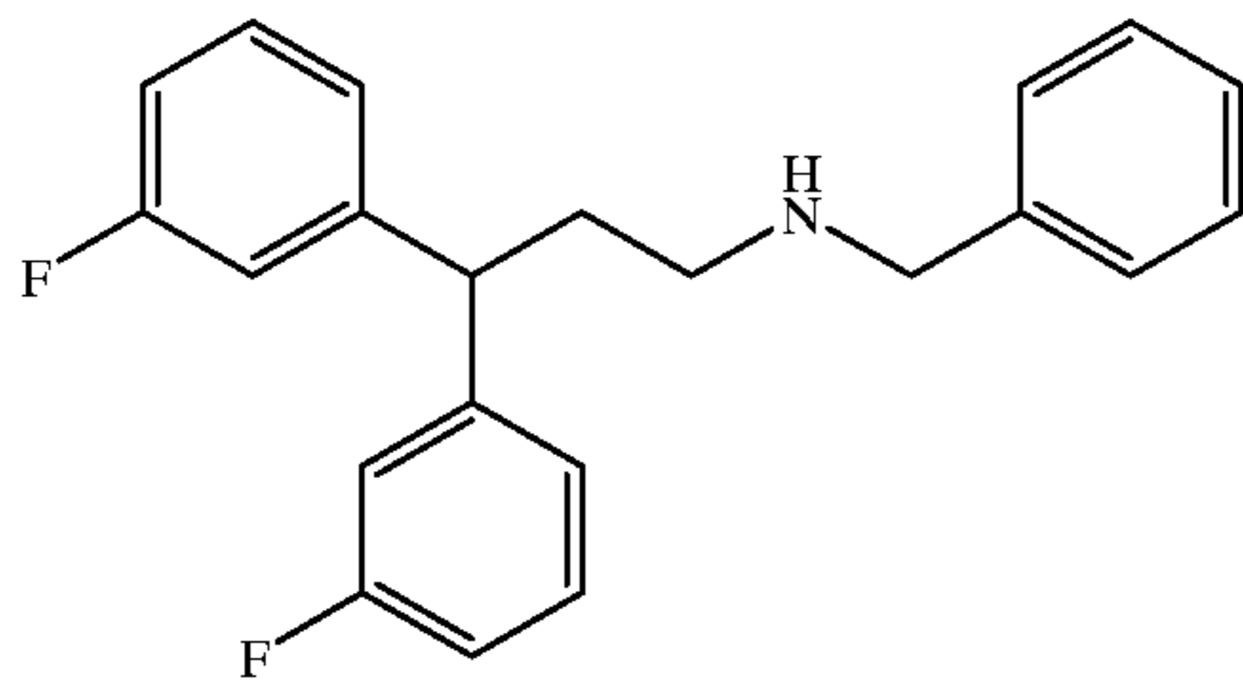
Compound 92
