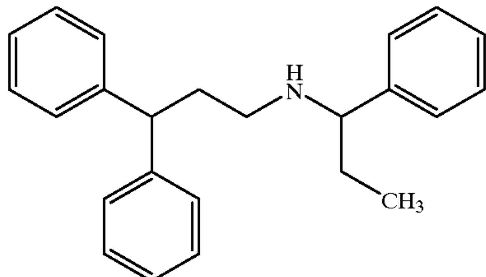
Compound 91
