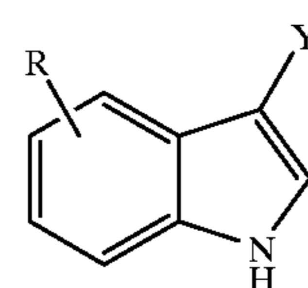
Headgroup B
