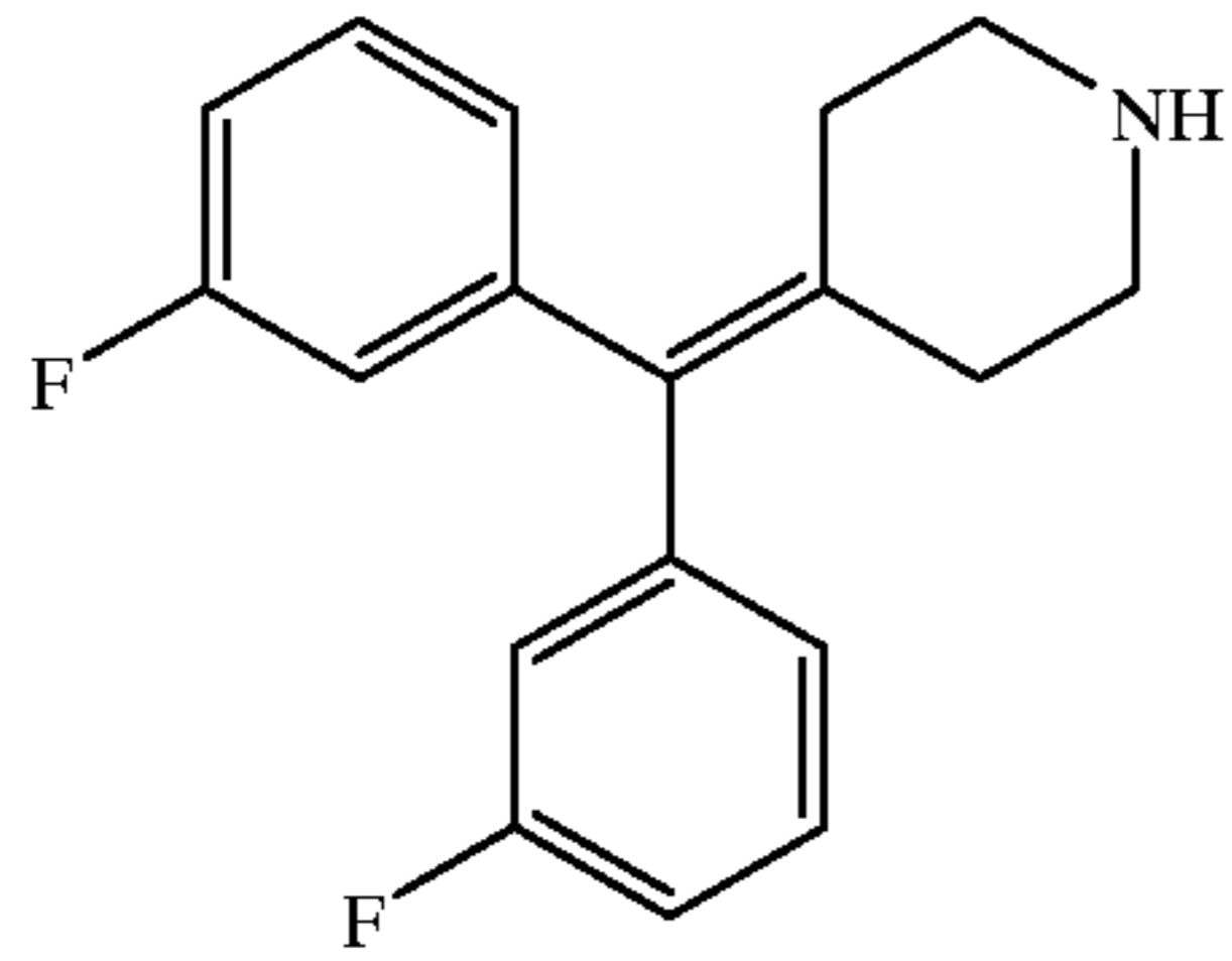
Compound 110
