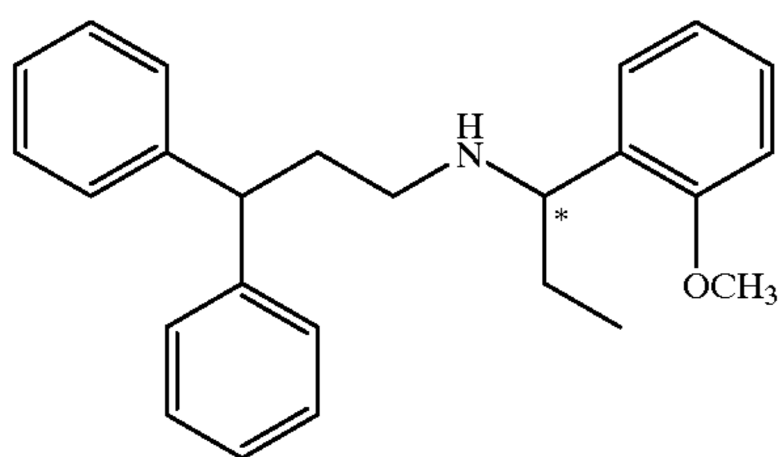
Compound 167
