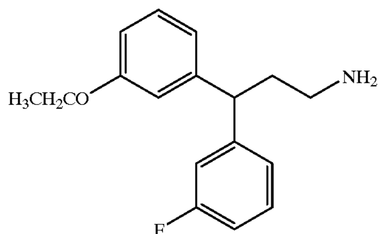
Compound 135
