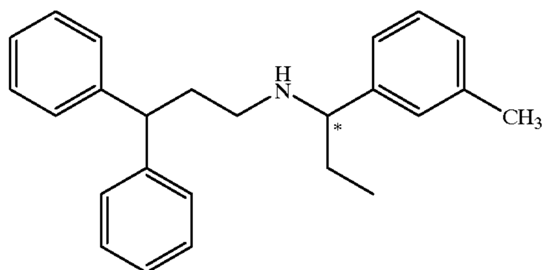
Compound 168
