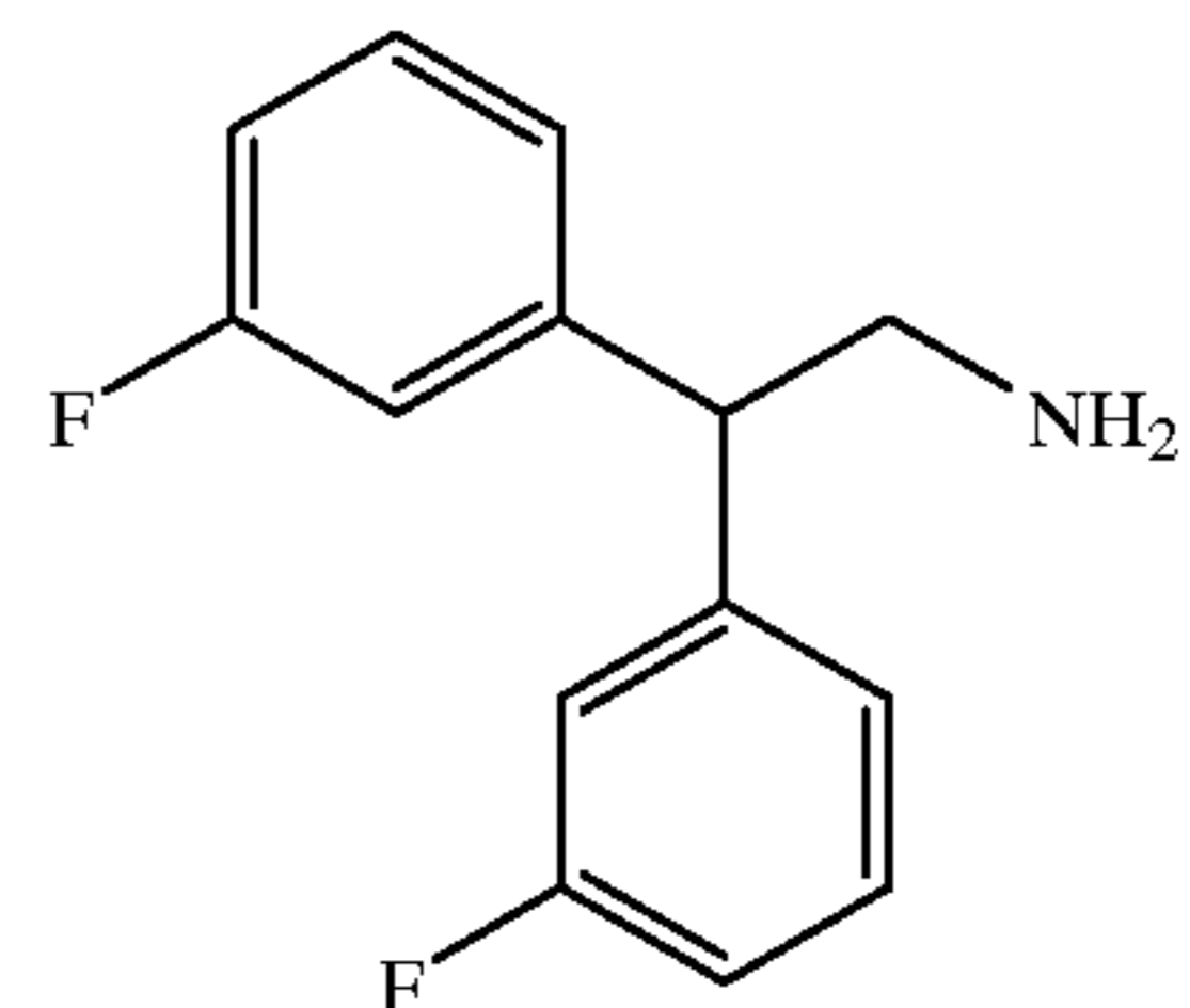
Compound 98
