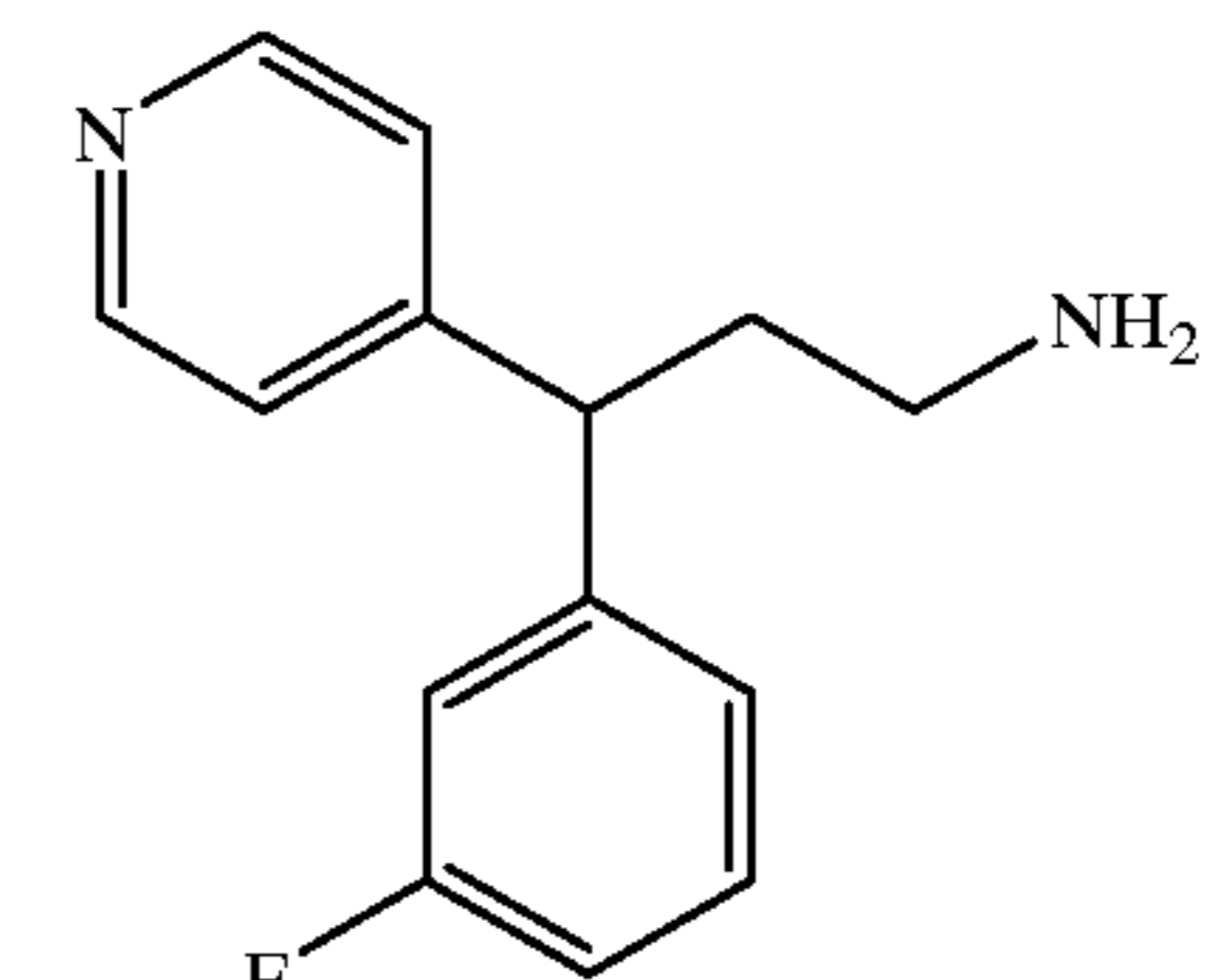
Compound 79
