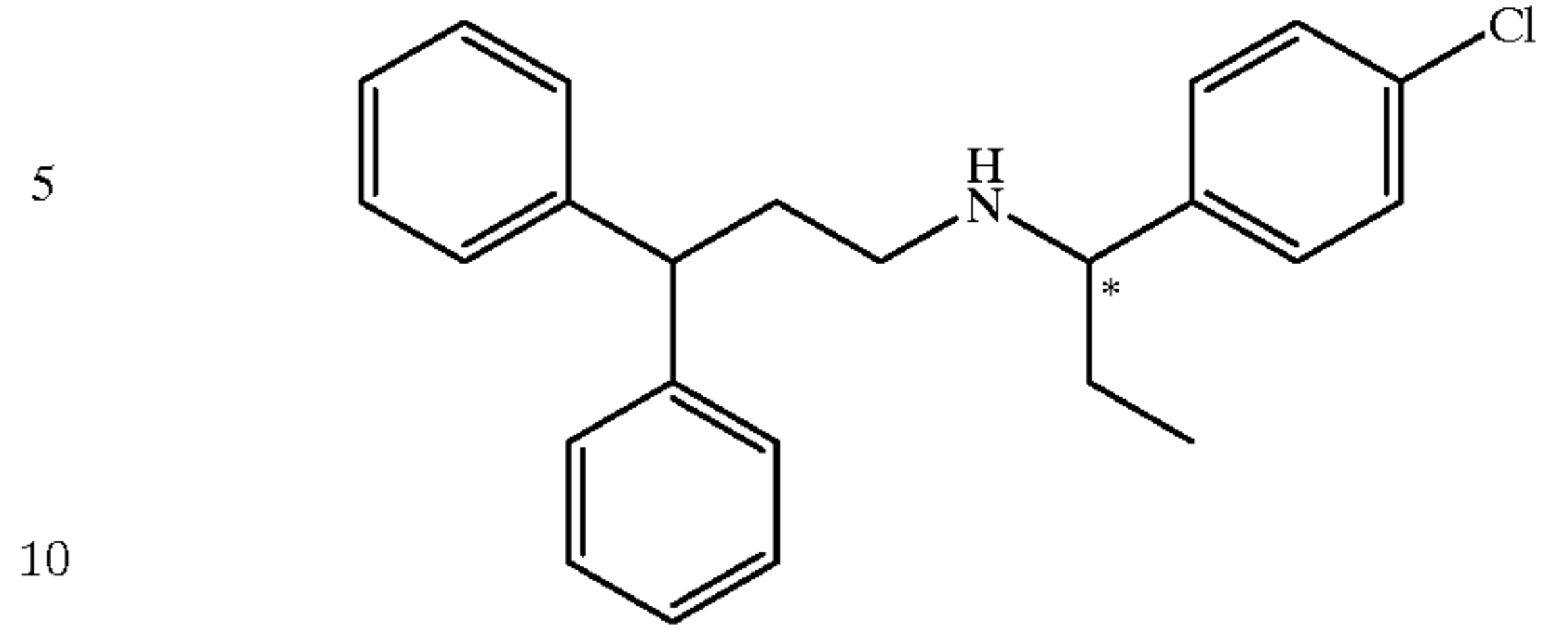
Compound 160
