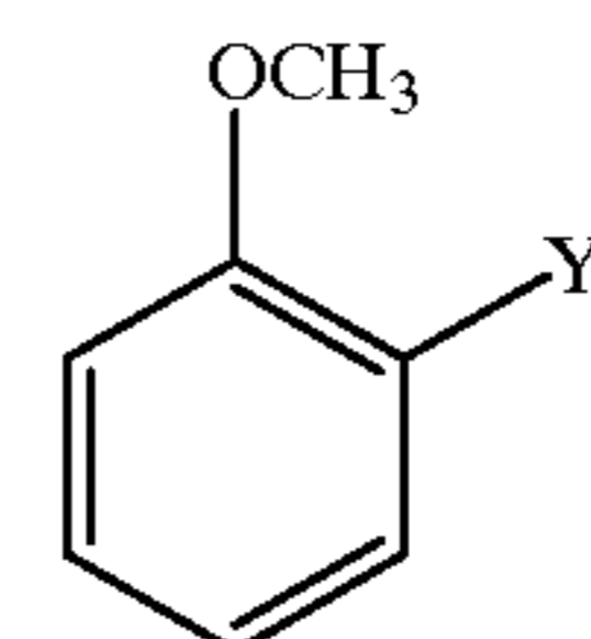
Headgroup A
