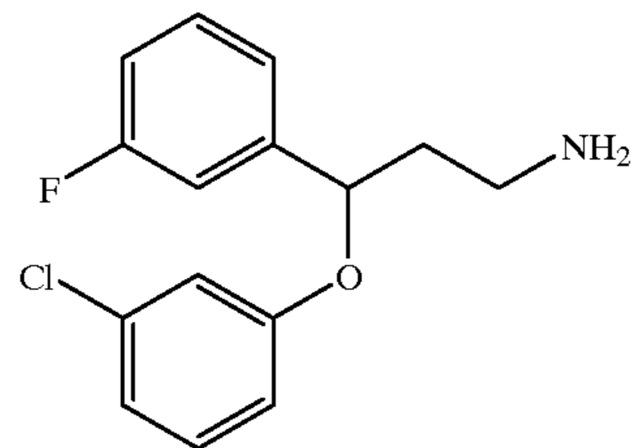
Compound 120
