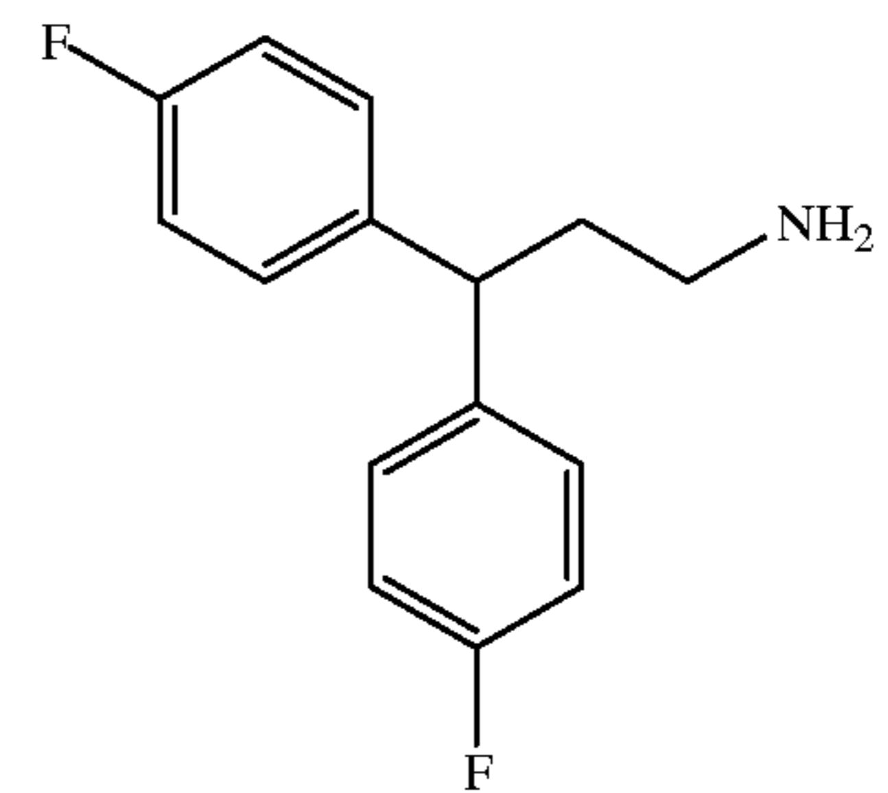
Compound 77
