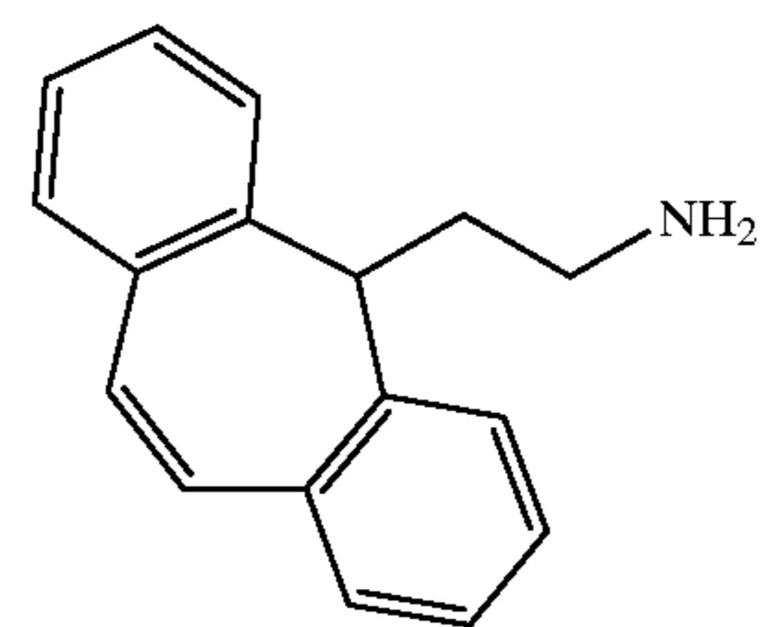
Compound 184
