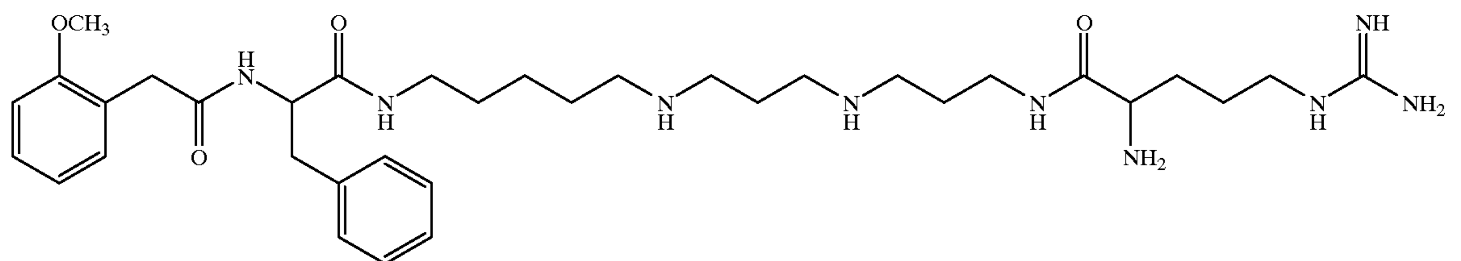
Compound 6
