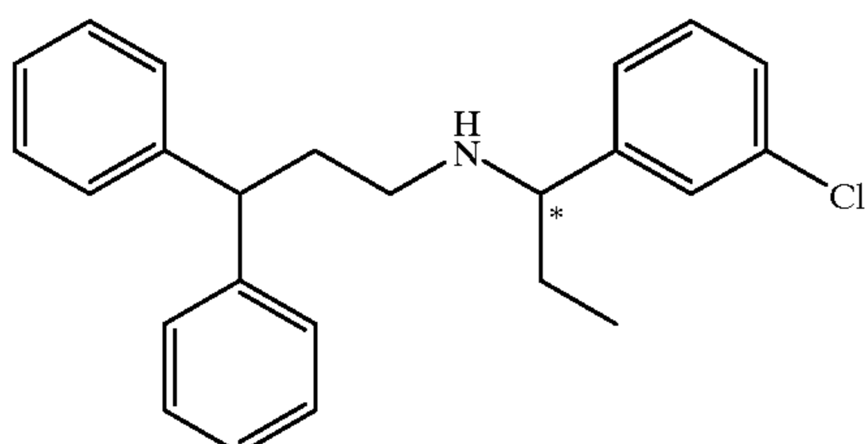
Compound 159
