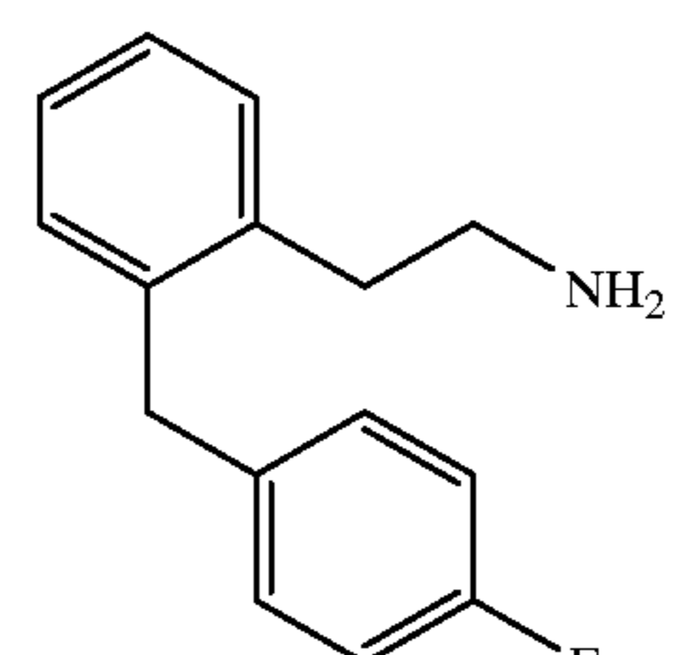
Compound 131
