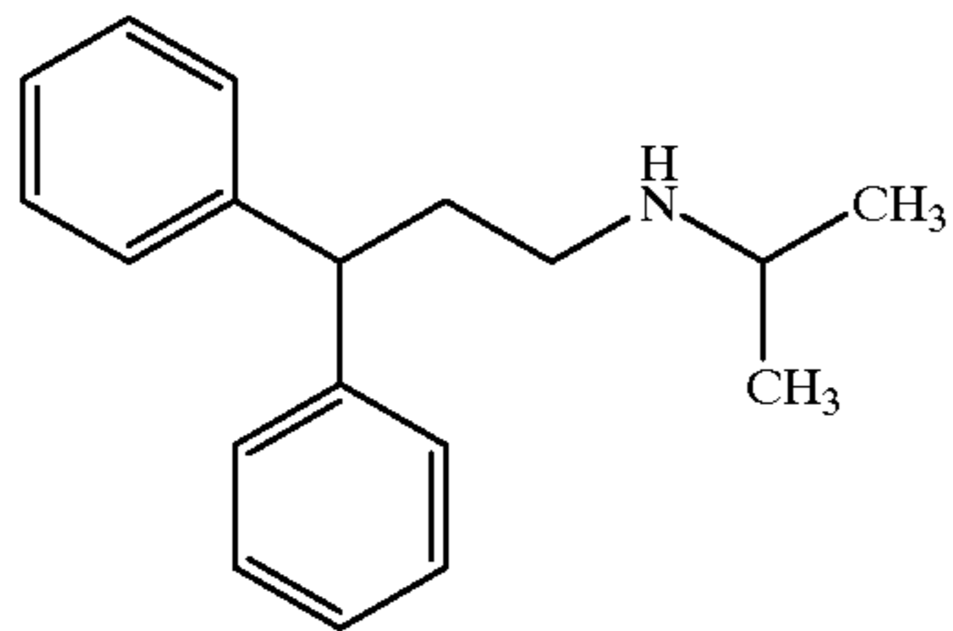
Compound 72
