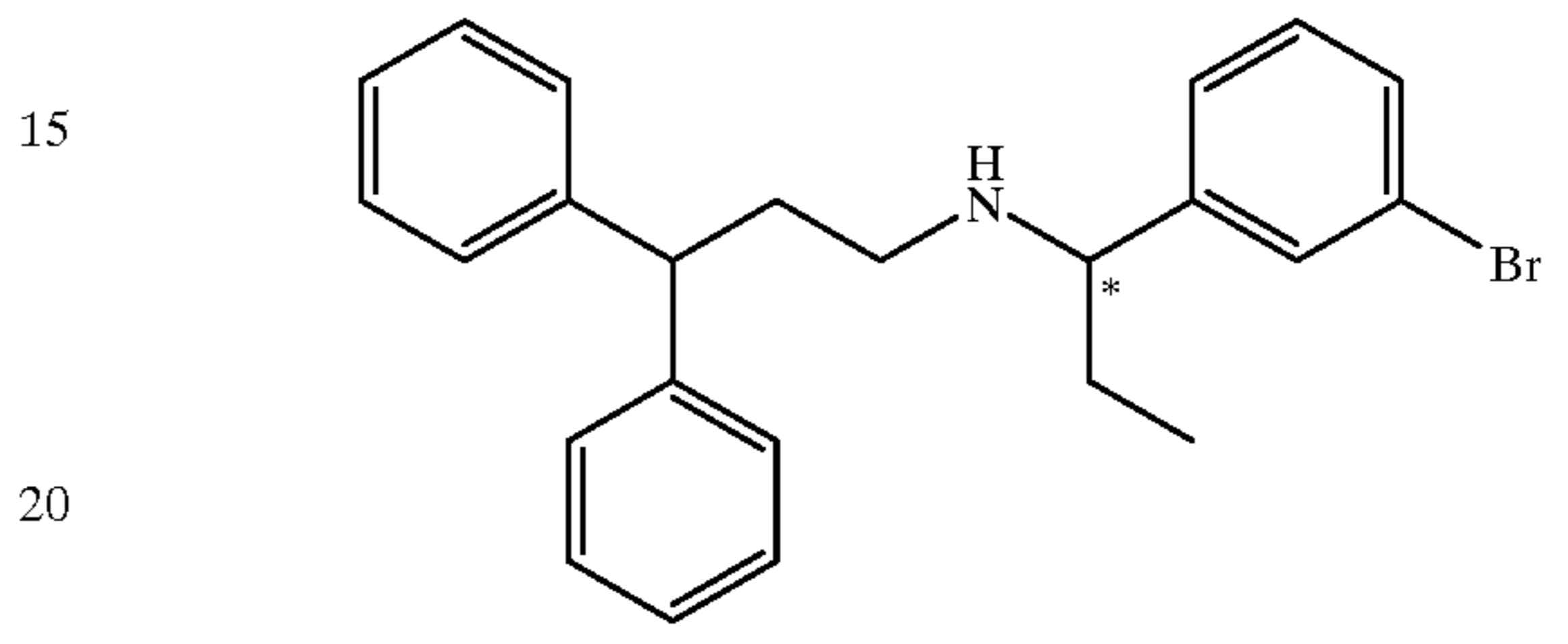
Compound 161
