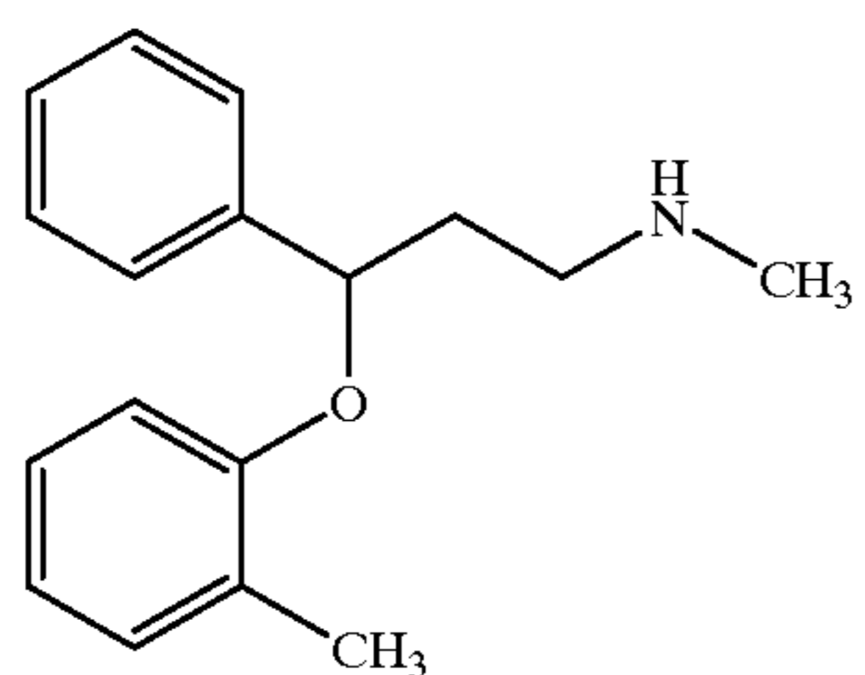
Compound 179
