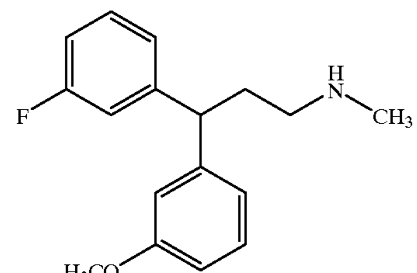
Compound 142
