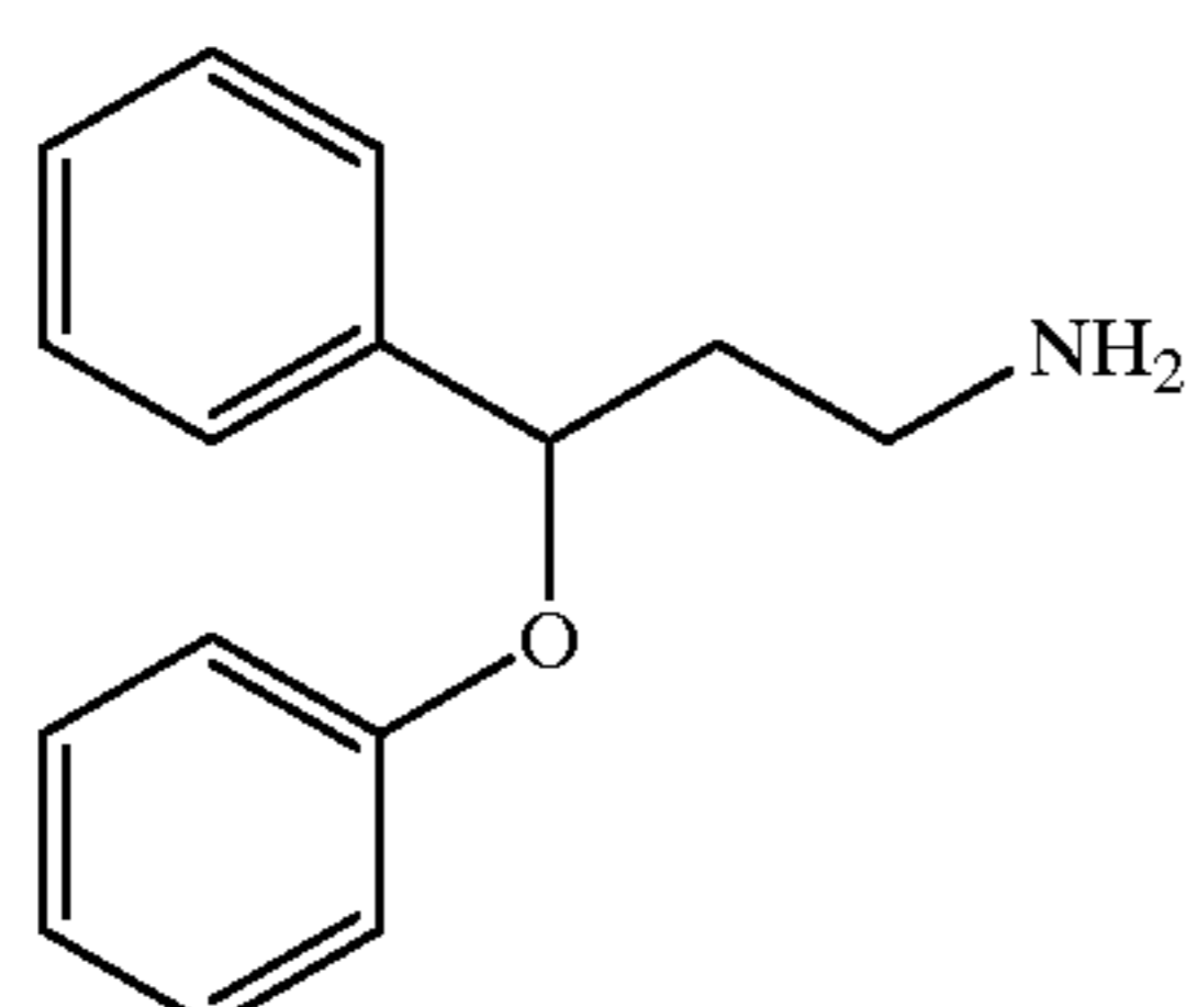
Compound 146
