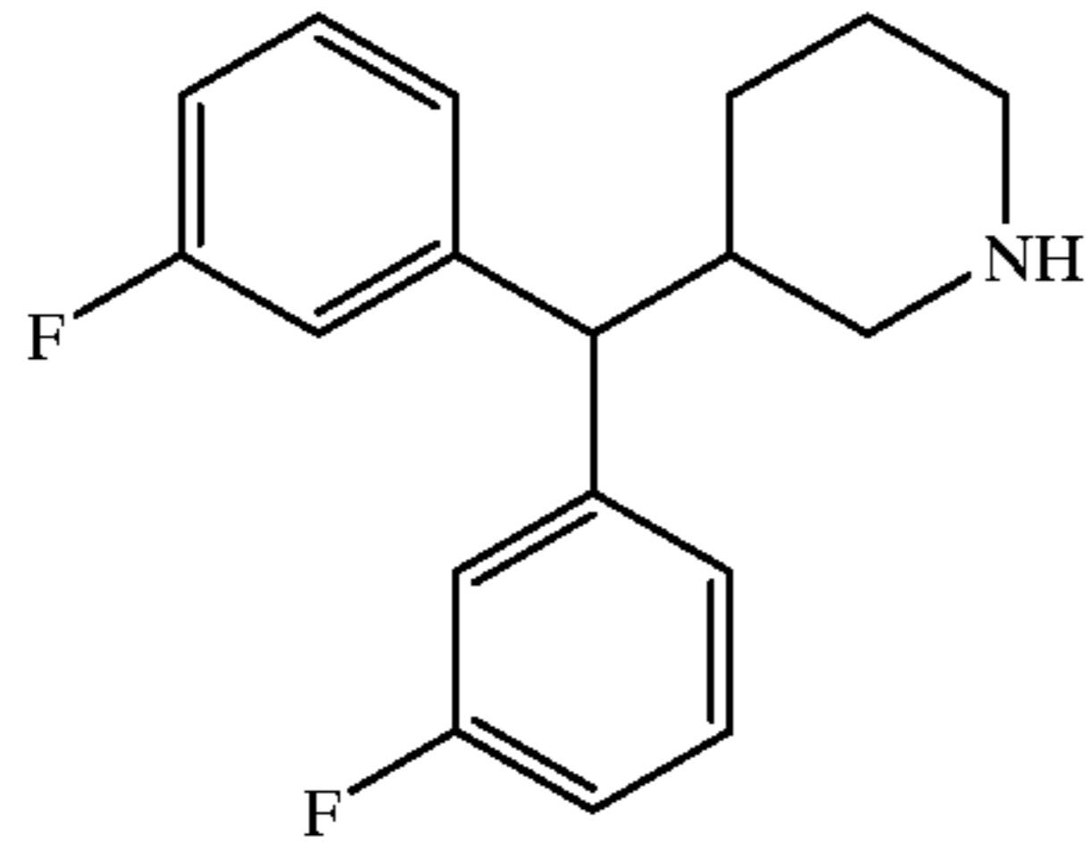
Compound 111
