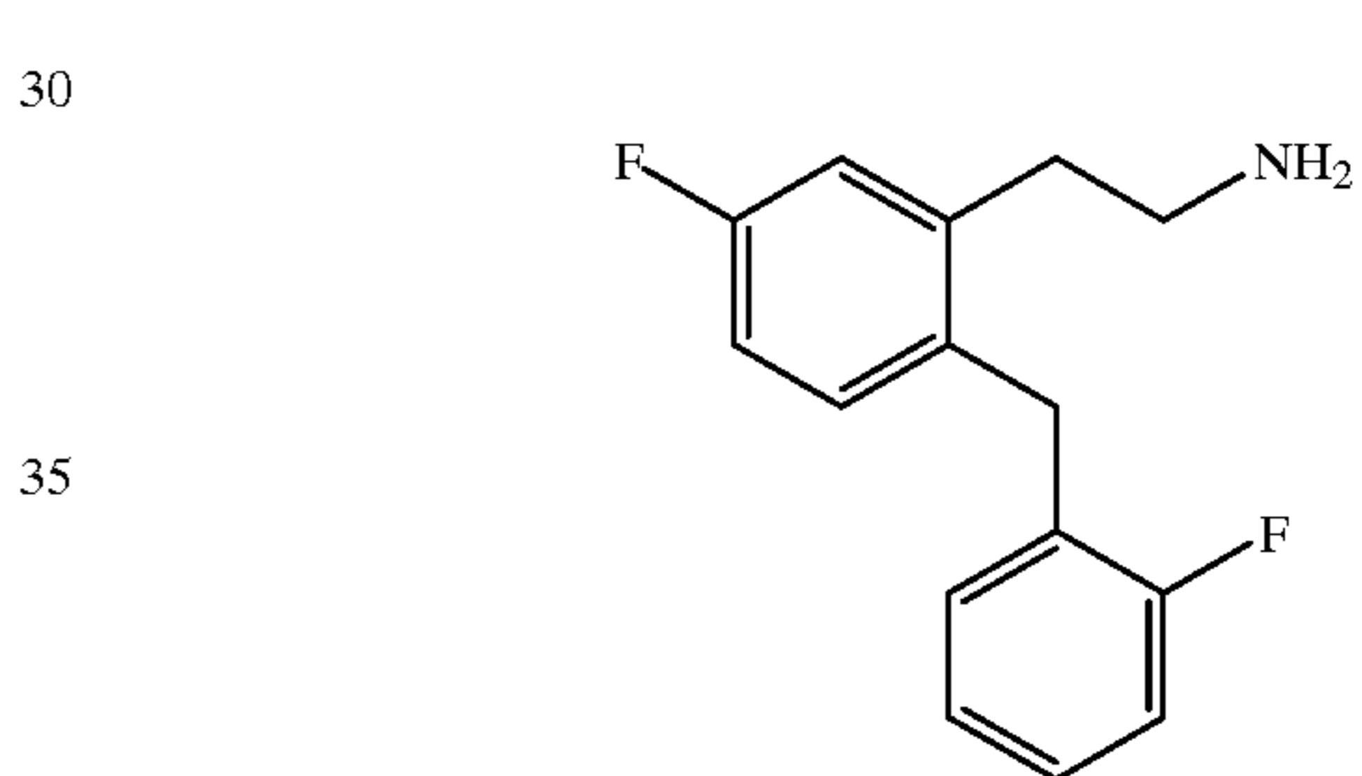
Compound 203
