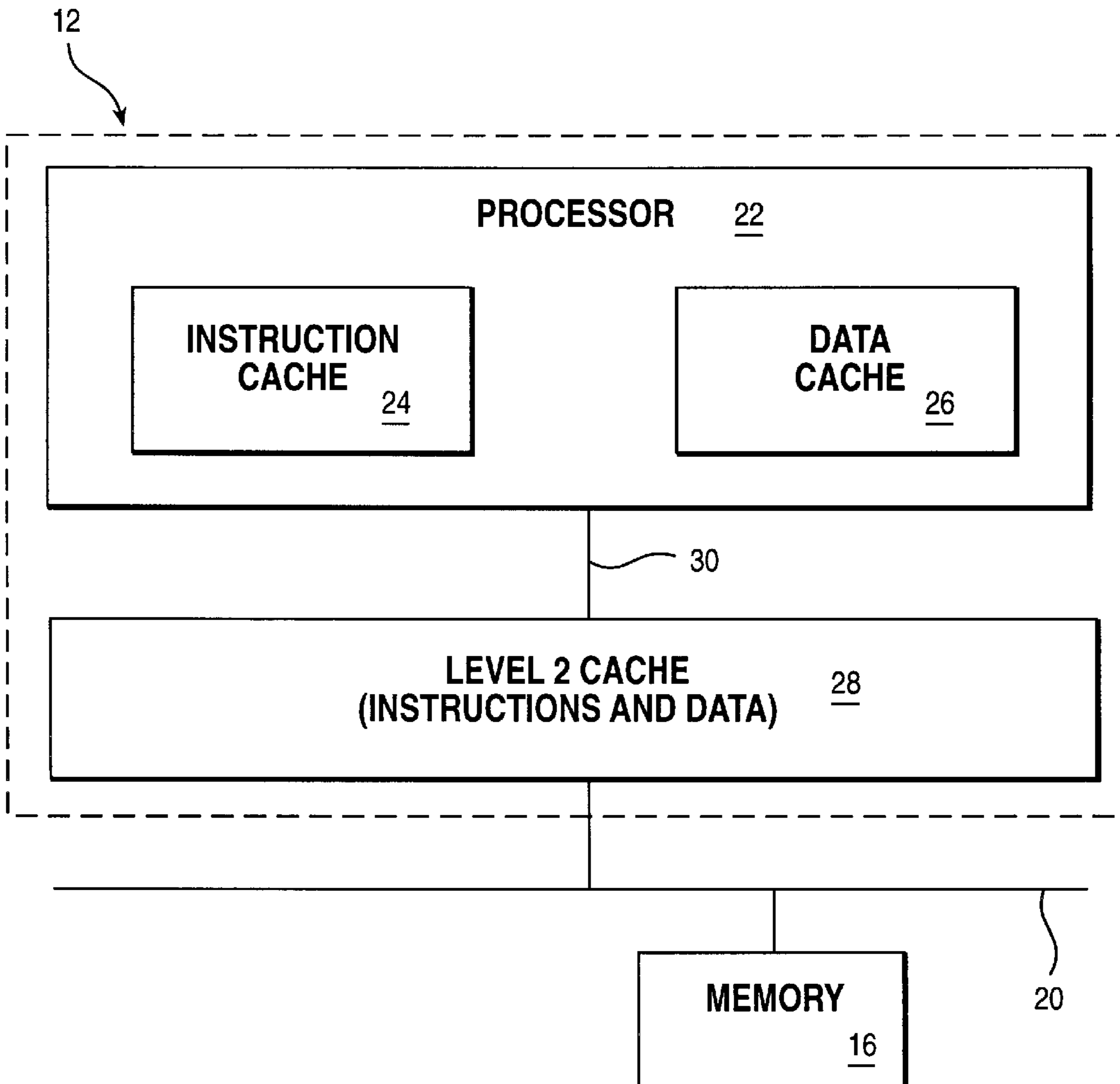
FIG. 1 PRIOR ART
