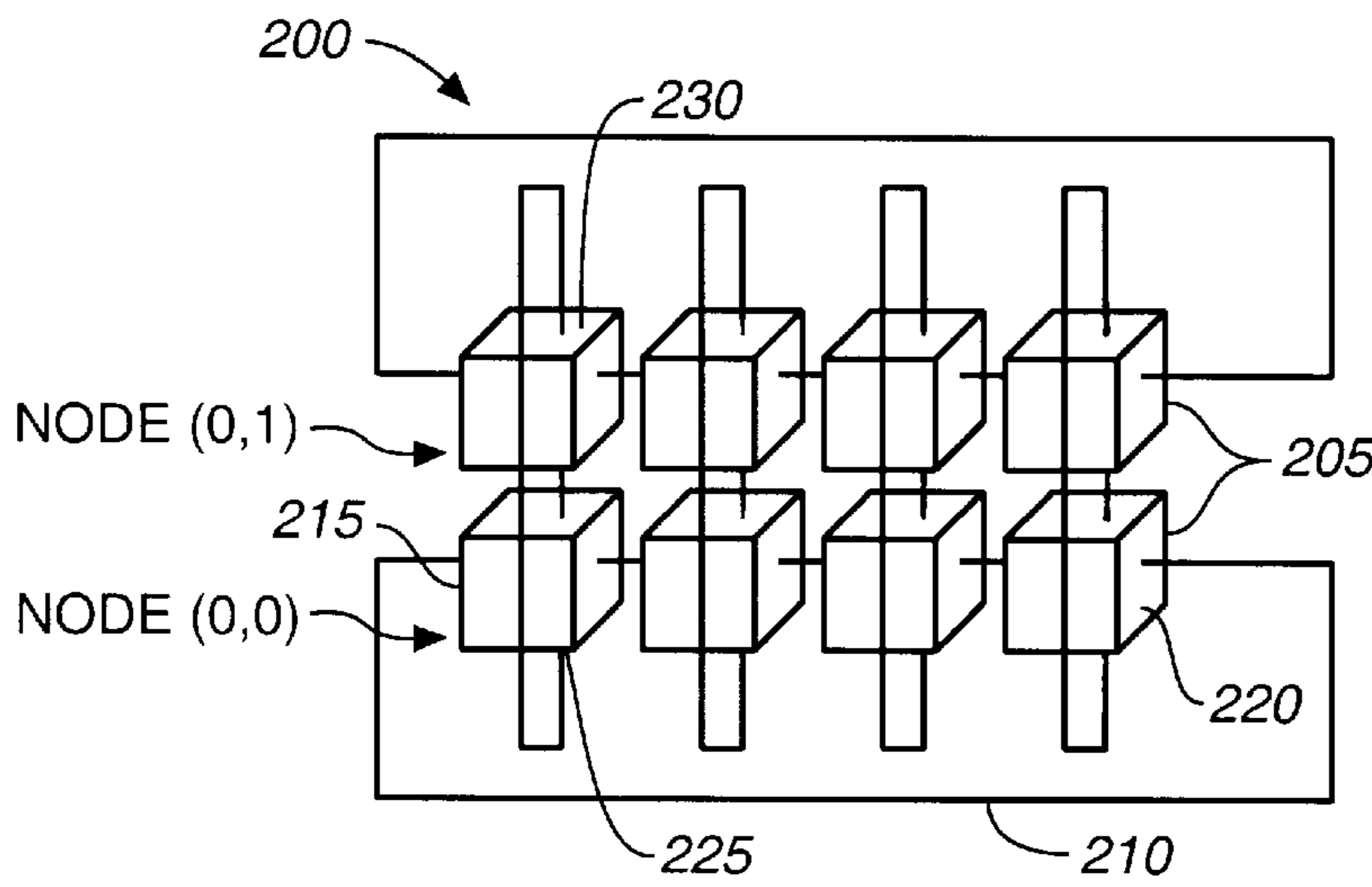
FIG. 2 (PRIOR ART)
