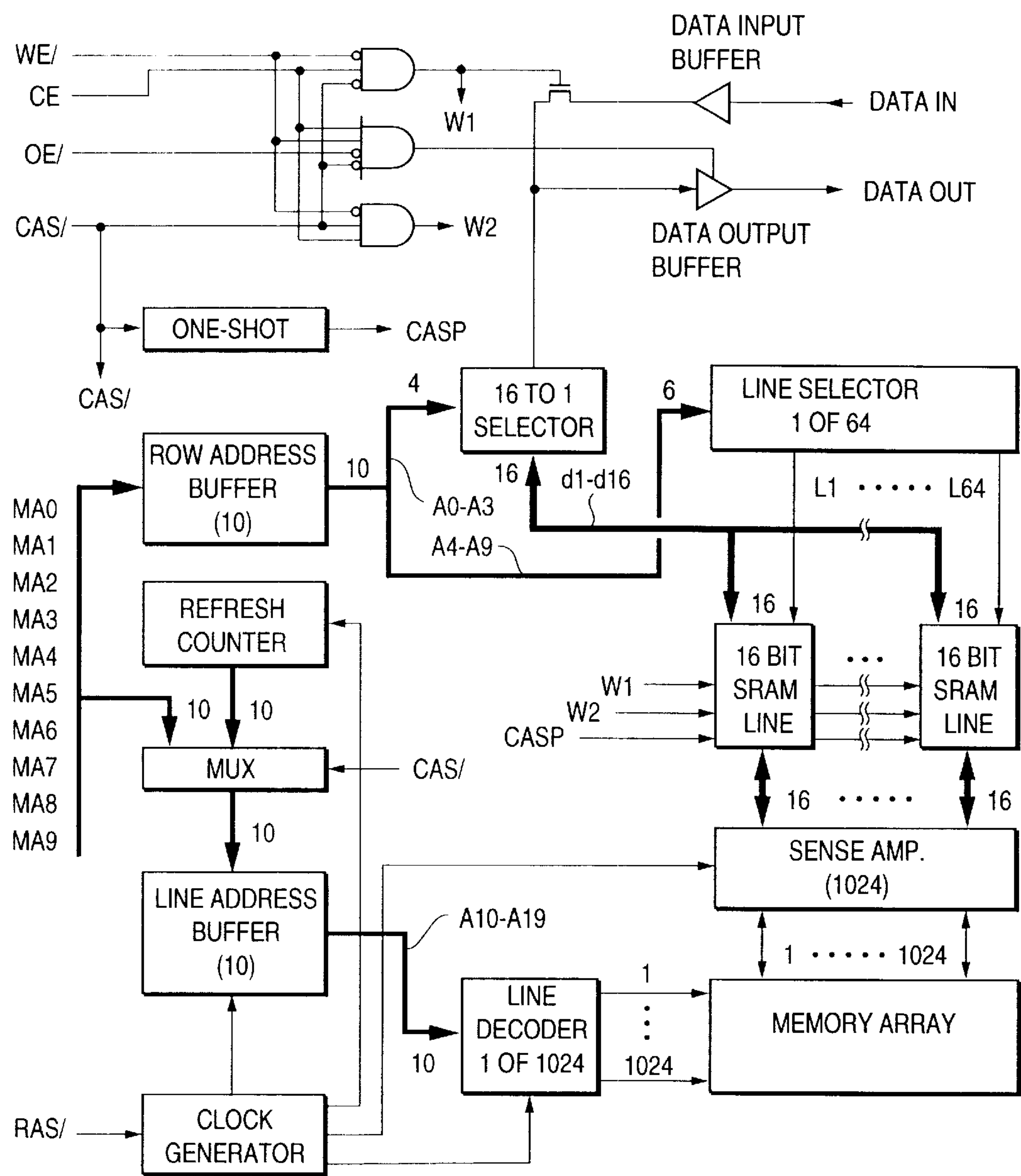
FIG. 95 PRIOR ART
