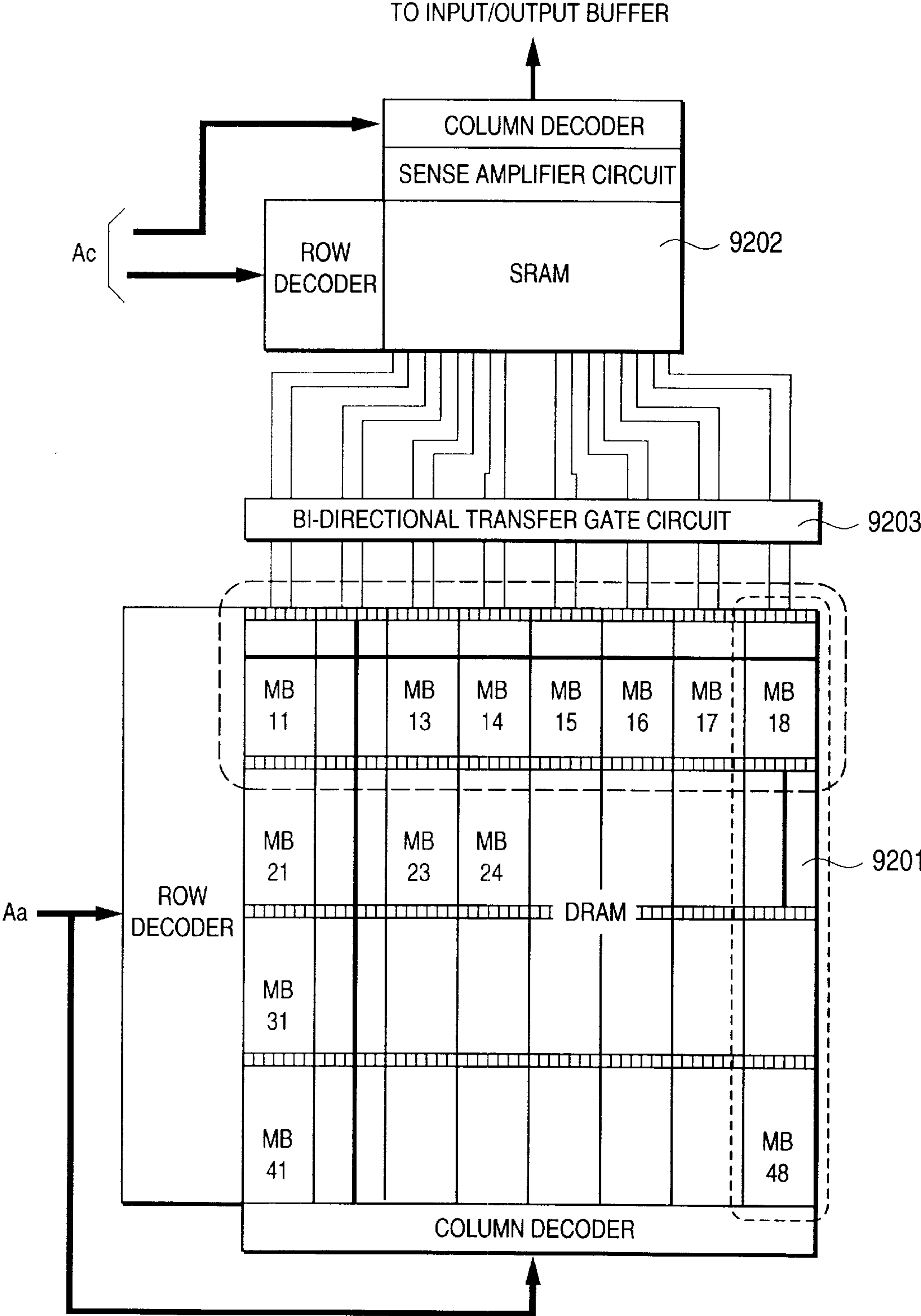
FIG. 92 PRIOR ART
