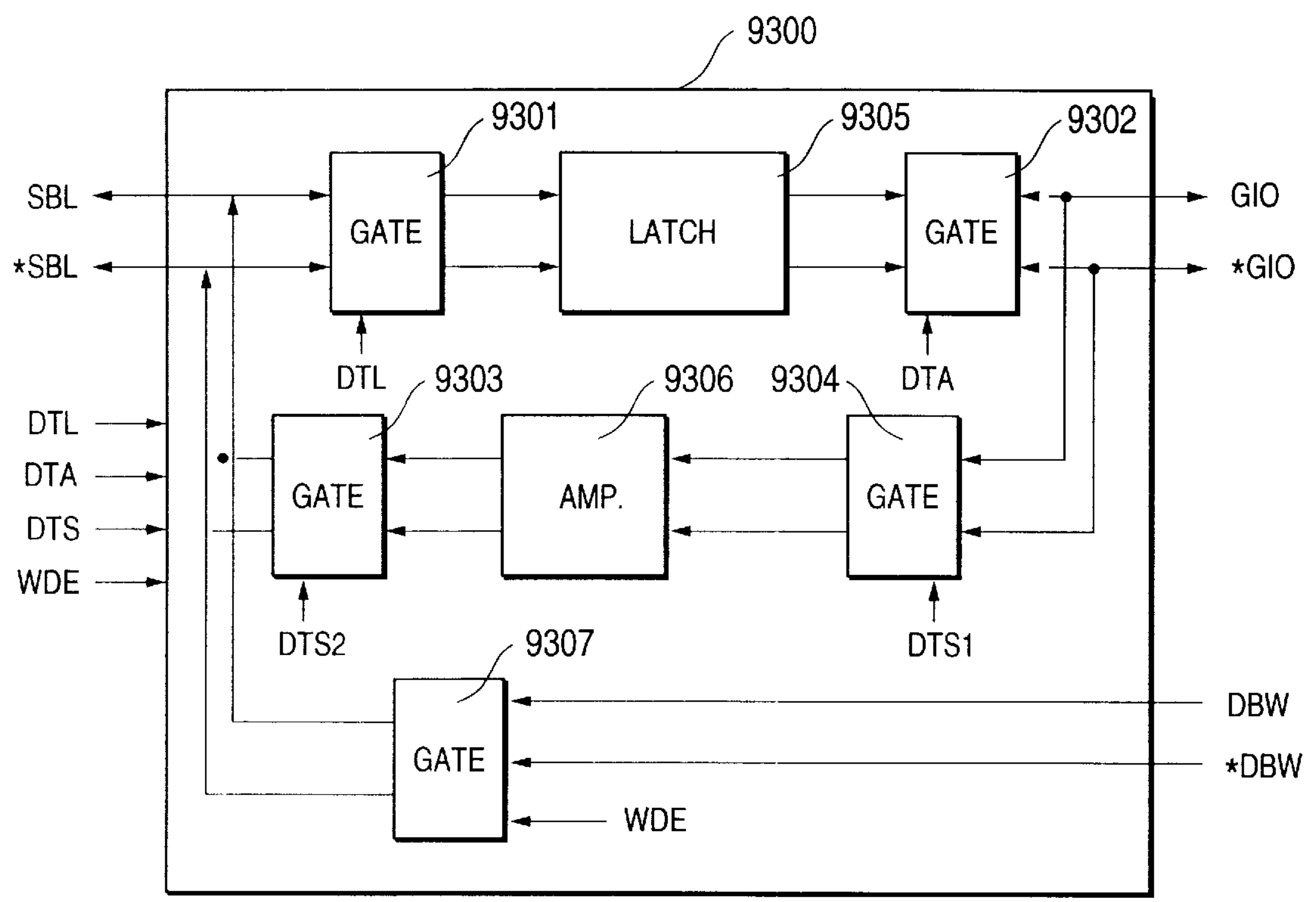
FIG. 93 PRIOR ART
