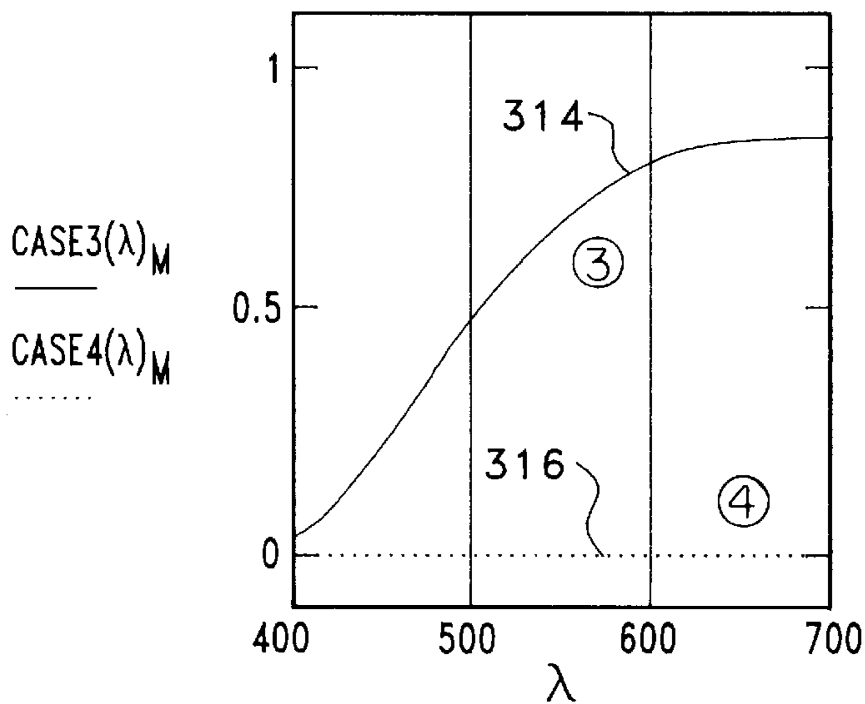
FIG. 3c (PRIOR ART)
