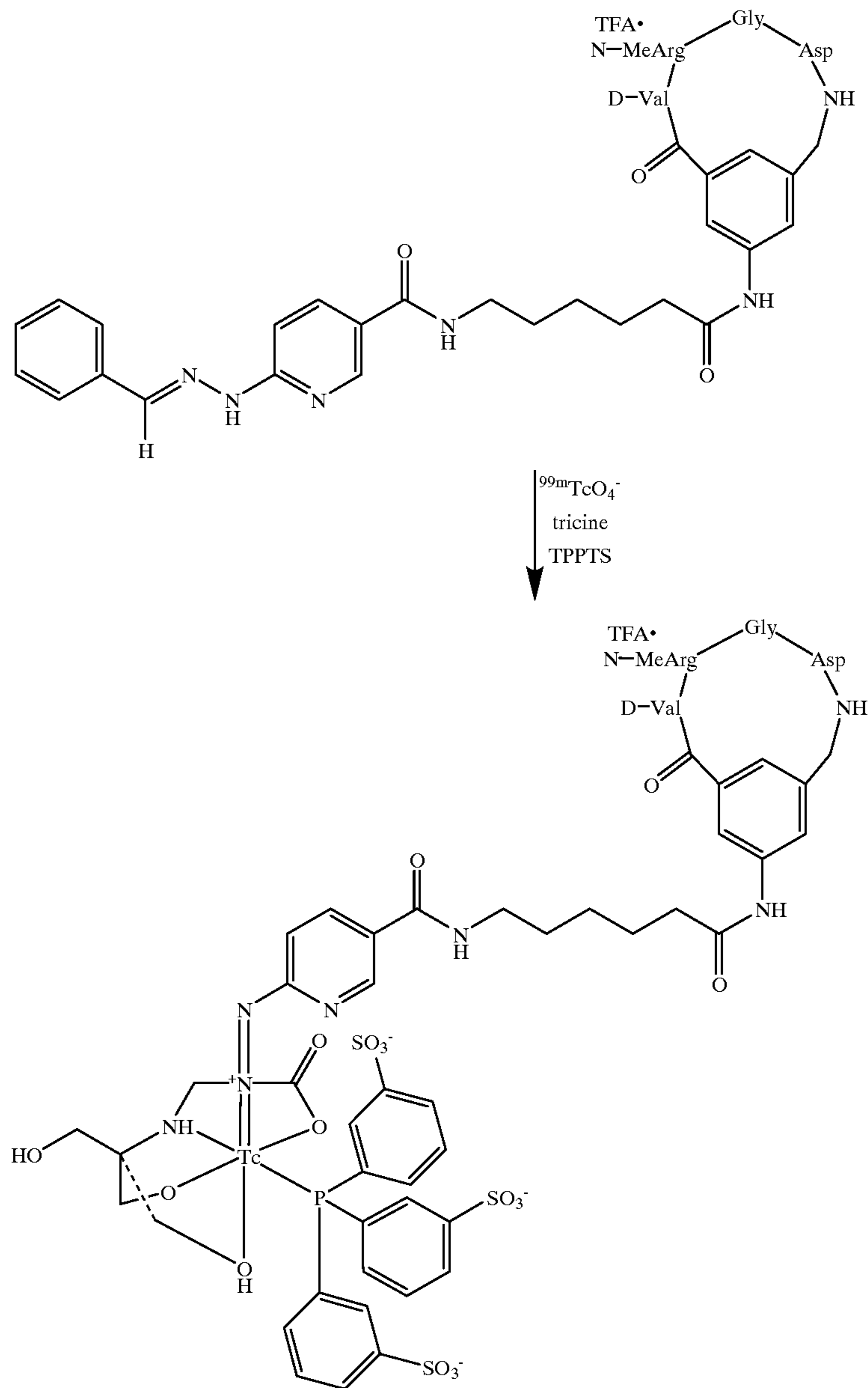
Scheme 6
