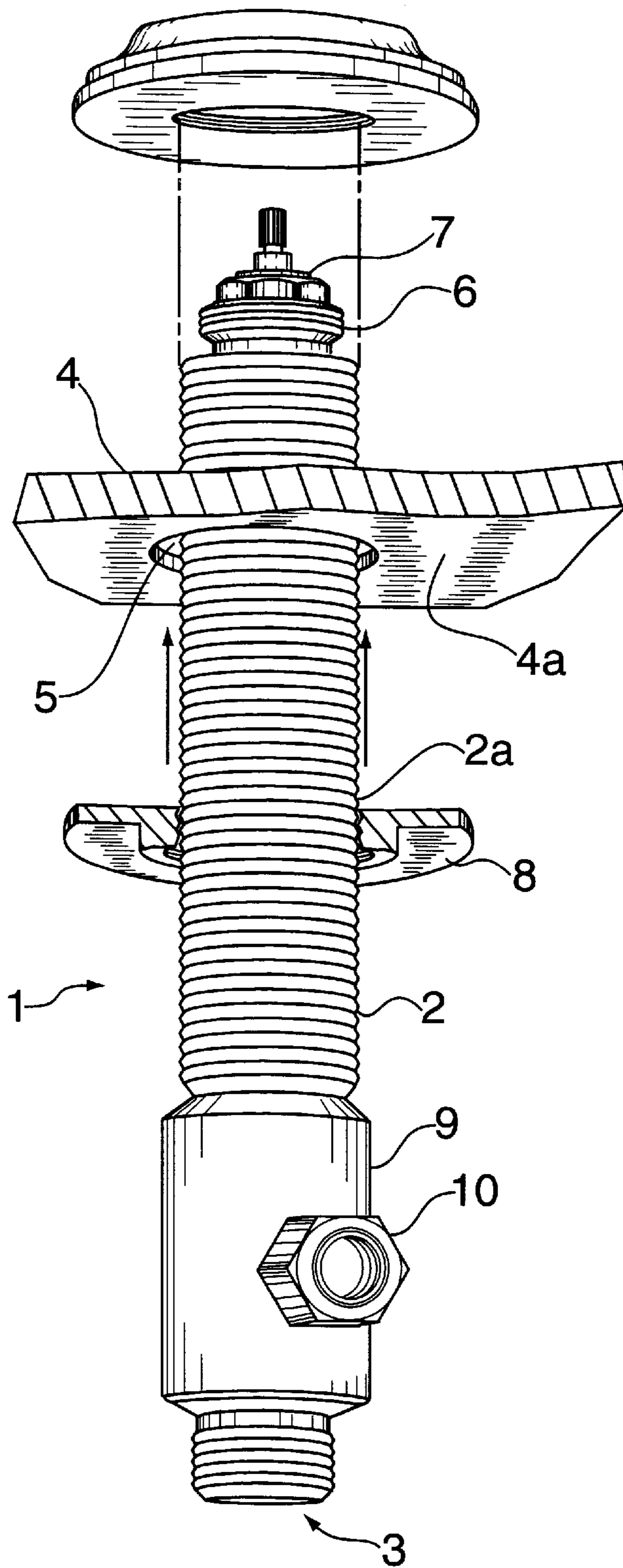
FIG. 1 PRIOR ART
