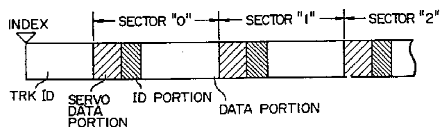
(1) IN WRITE OPERATION (SECTOR "1")
