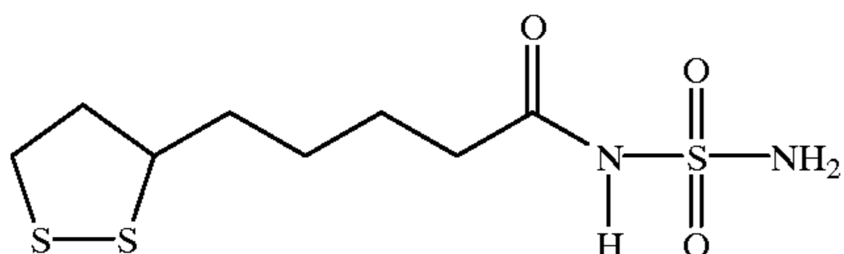
N-[5-(1,2-Dithiolan-3-yl)pentanoyl]sulfamide (Compound No. 1-539)
