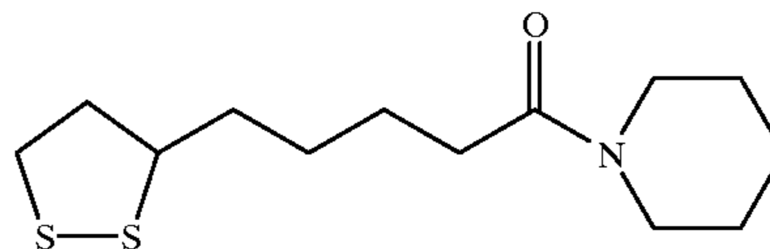
1-[5-(1,2-Dithiolan-3-yl)pentanoyl]piperidine (Compound No. 1-1130)
