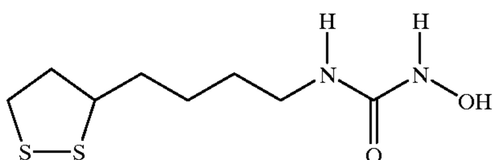
N-Hydroxy-N'-[4-(1,2-dithiolan-3-yl)butyl]urea (Compound No. 1-750)
