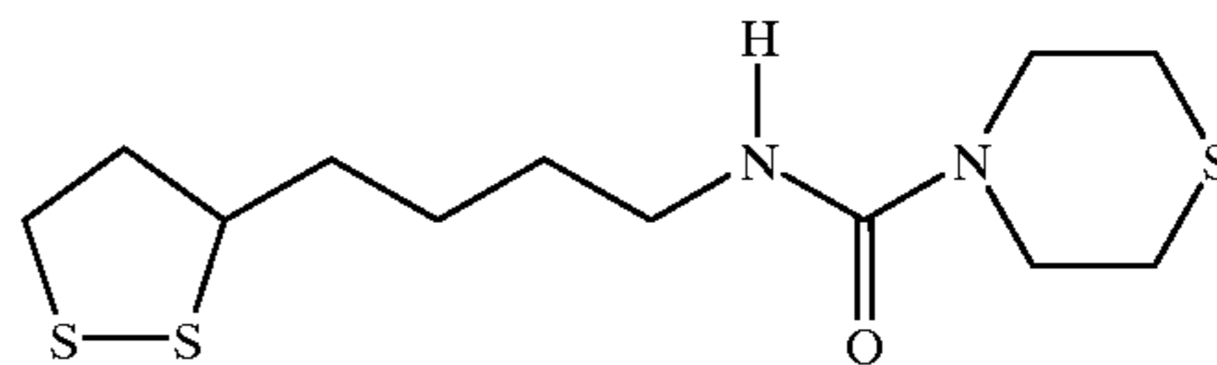
N-[4-(1,2-Dithiolan-3-yl)butyl]thiomorpholine-4-carboxamide (Compound No. 1-1143)
