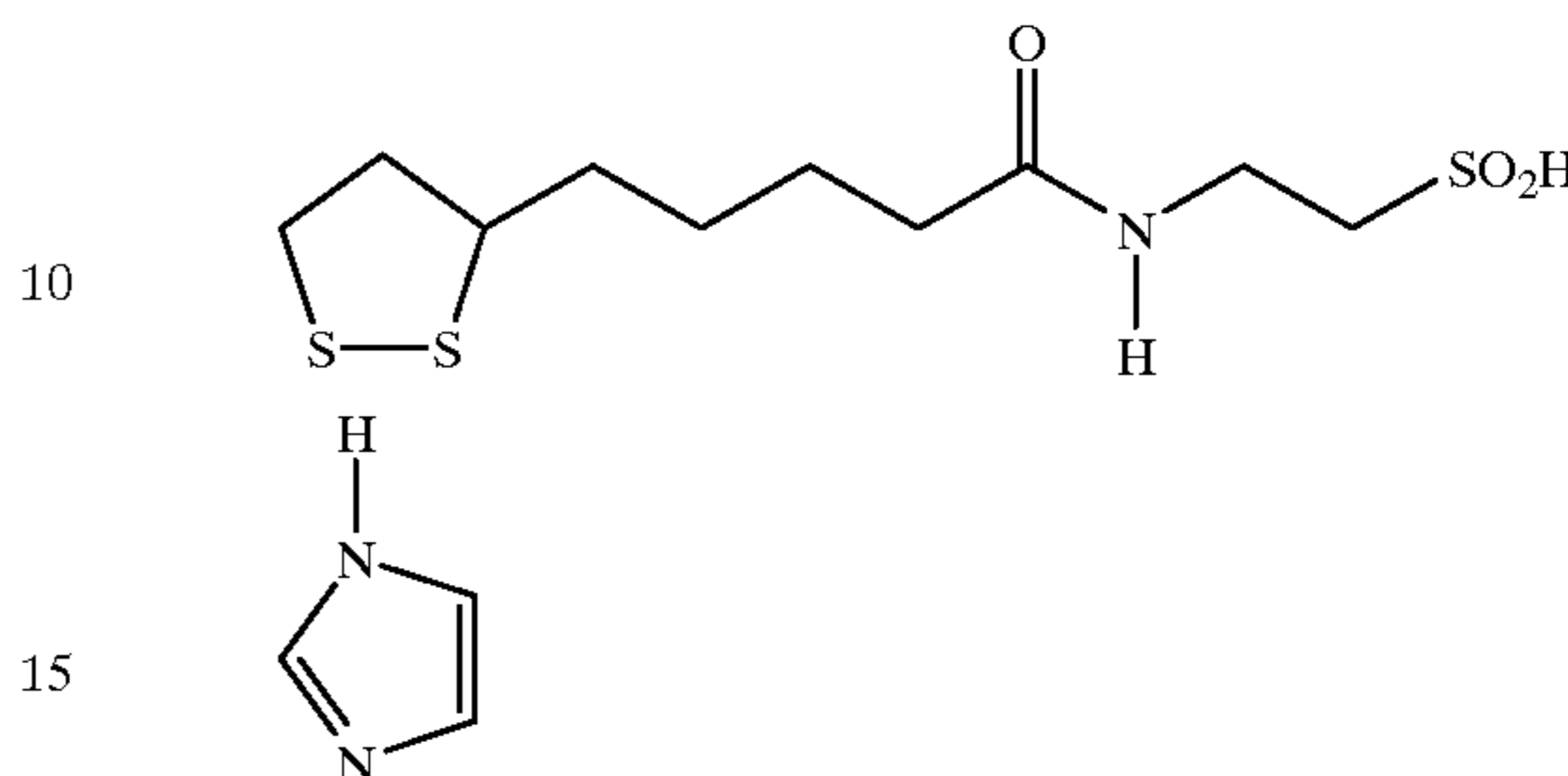
2-[5-(1,2-Dithiolan-3-yl)pentanoylamino] ethanesulfonic acid imidazole salt (Compound No. 1-57 imidazole salt)
