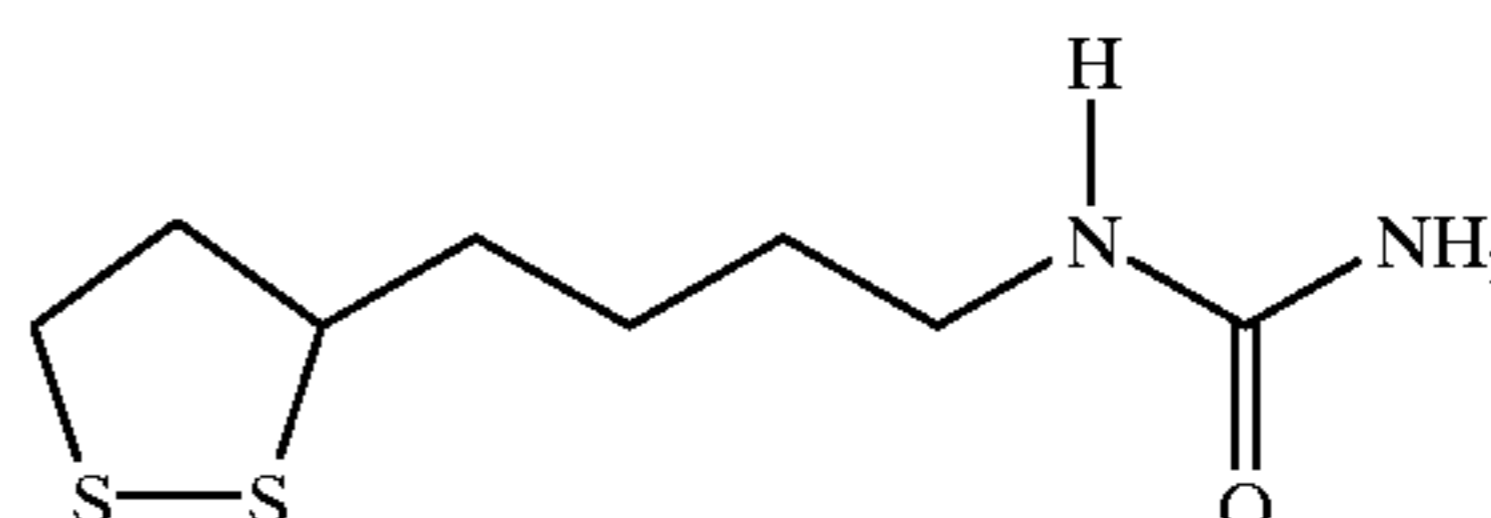
N-[4-(1,2-Dithiolan-3-yl)butyl]urea (Compound No. 1-693)
