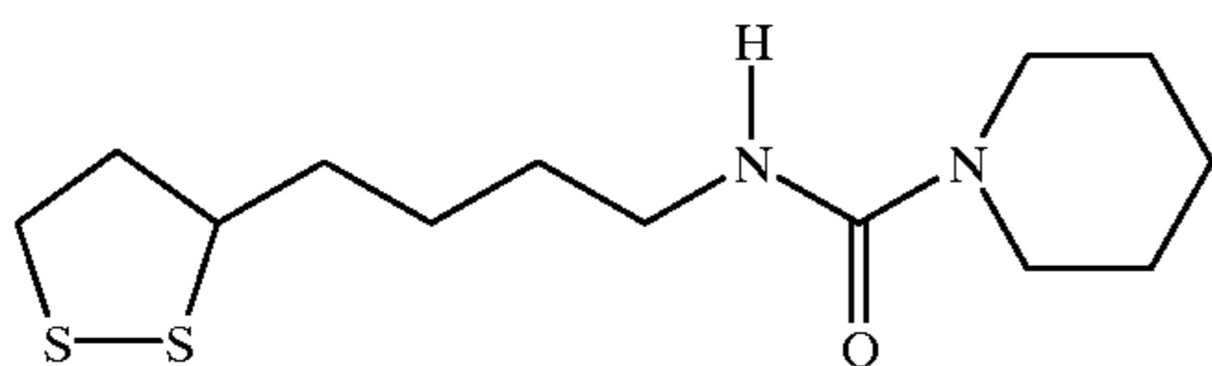
N-[4-(1,2-Dithiolan-3-yl)butyl]piperidine-1-carboxamide (Compound No. 1-1140)
