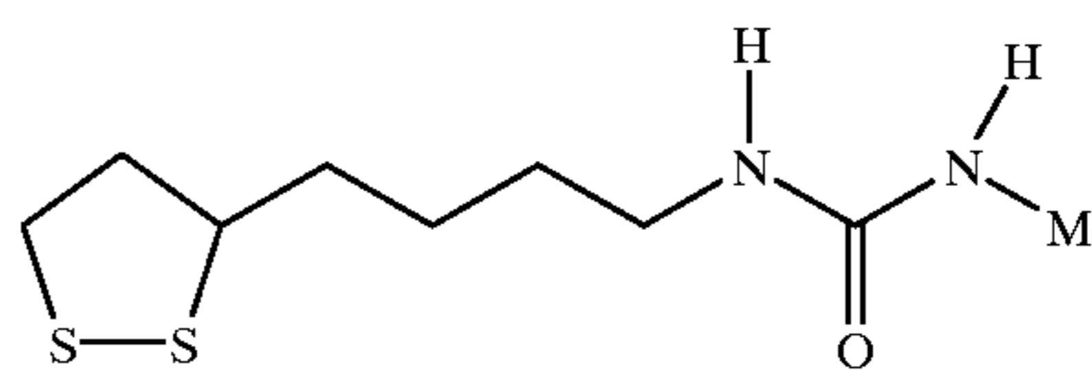
N-[4-(1,2-Dithiolan-3-yl)butyl-N'-methylurea (Compound No. 1-733)
