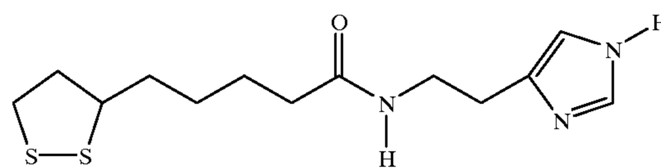
N \beta -[5-(1,2-Dithiolan-3-yl)pentanoyl]histamine (Compound No. 1-75)
