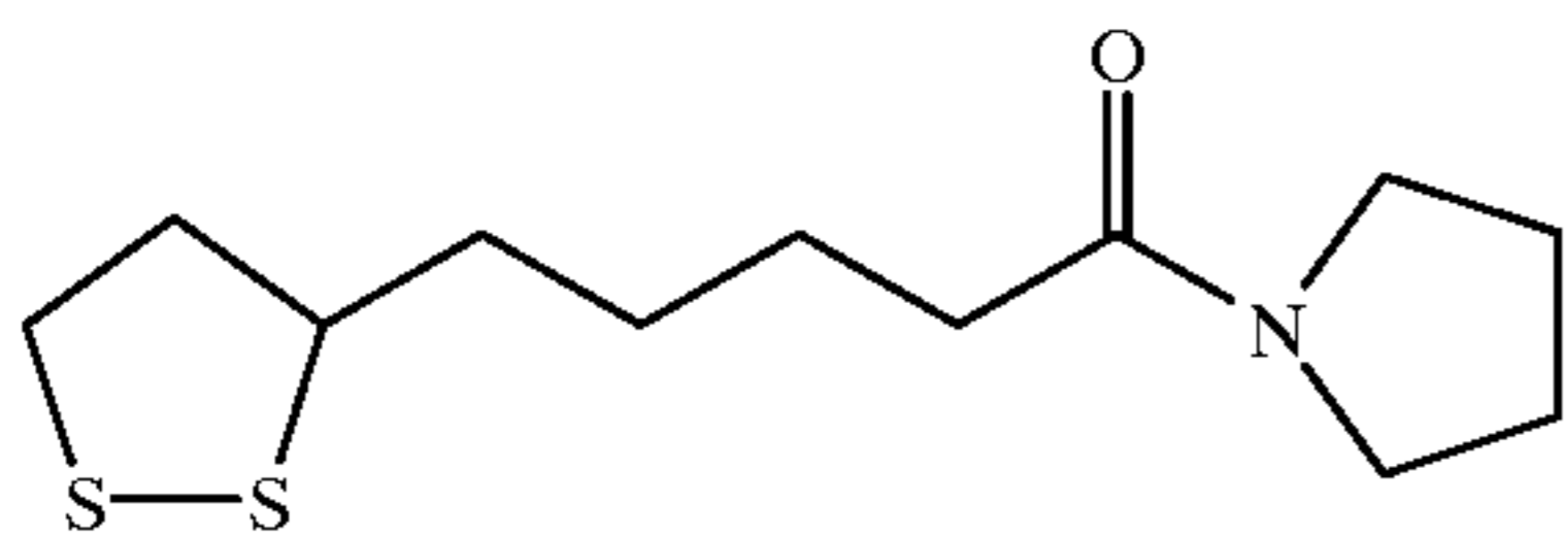
1-[5-(1,2-Dithiolan-3-yl)pentanoyl]pyrrolidine (Compound No. 1-1129)
