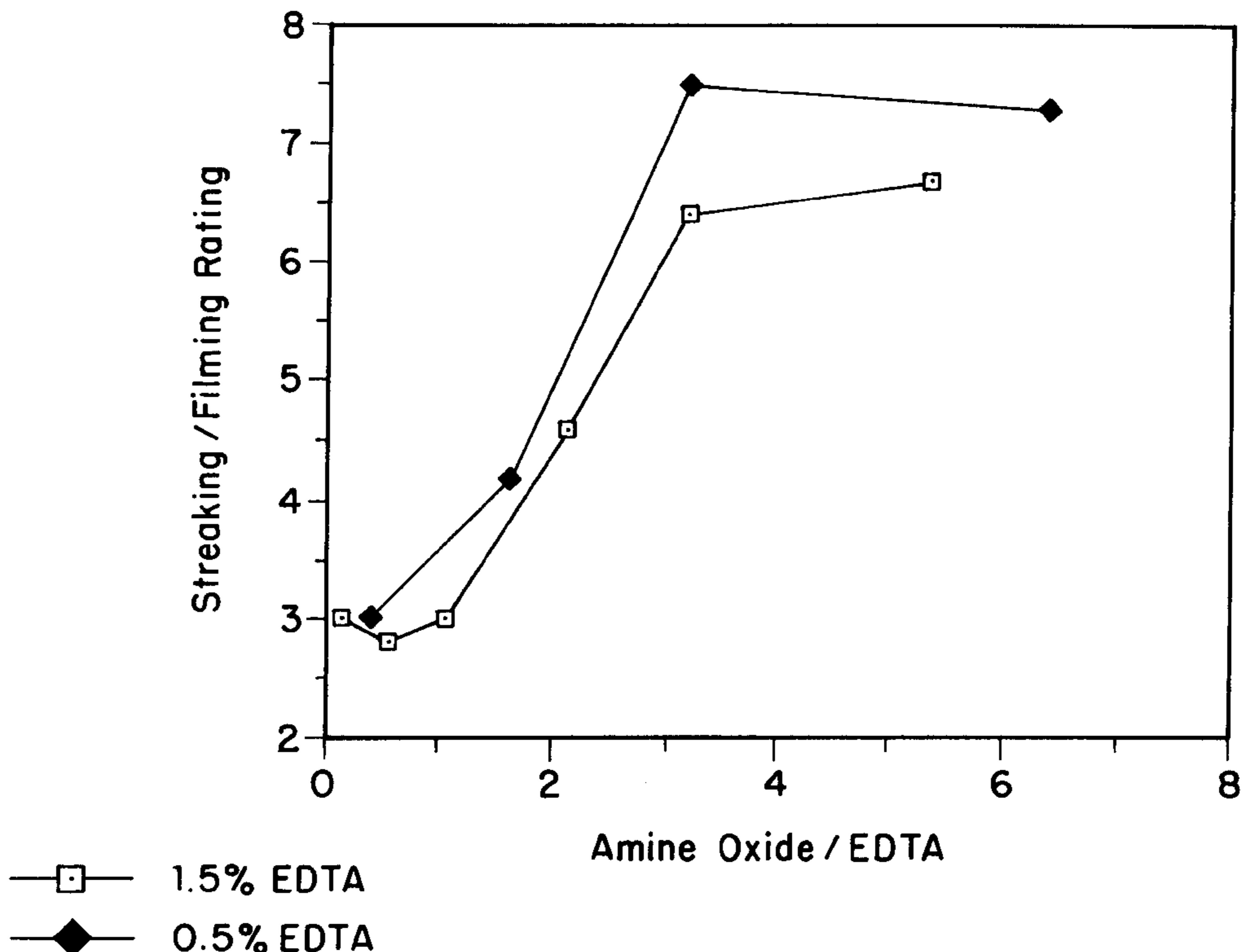
Streaking/Filming Rating vs. Amine Oxide/EDTA Ratio
