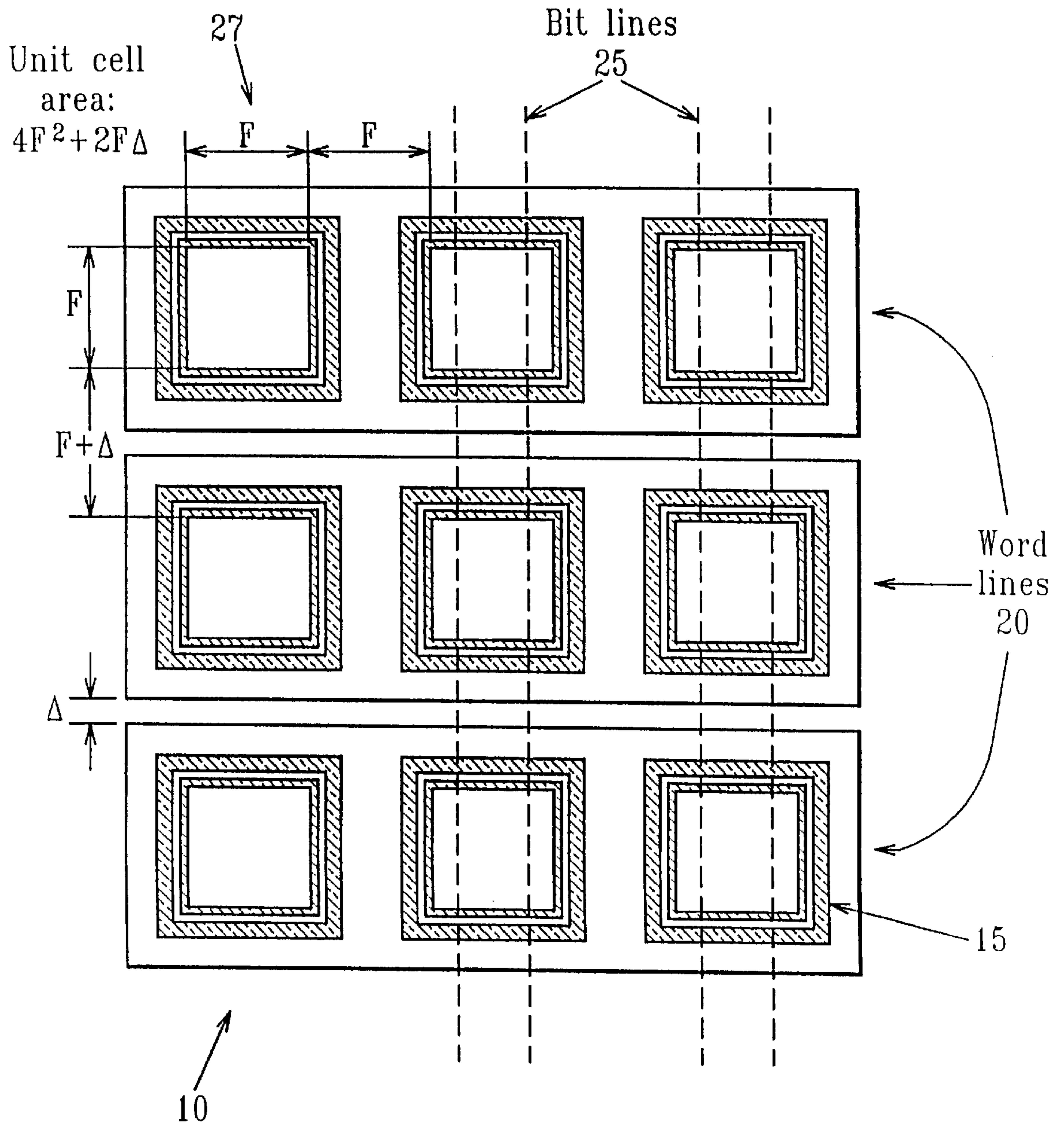
FIG. 1 (PRIOR ART)
