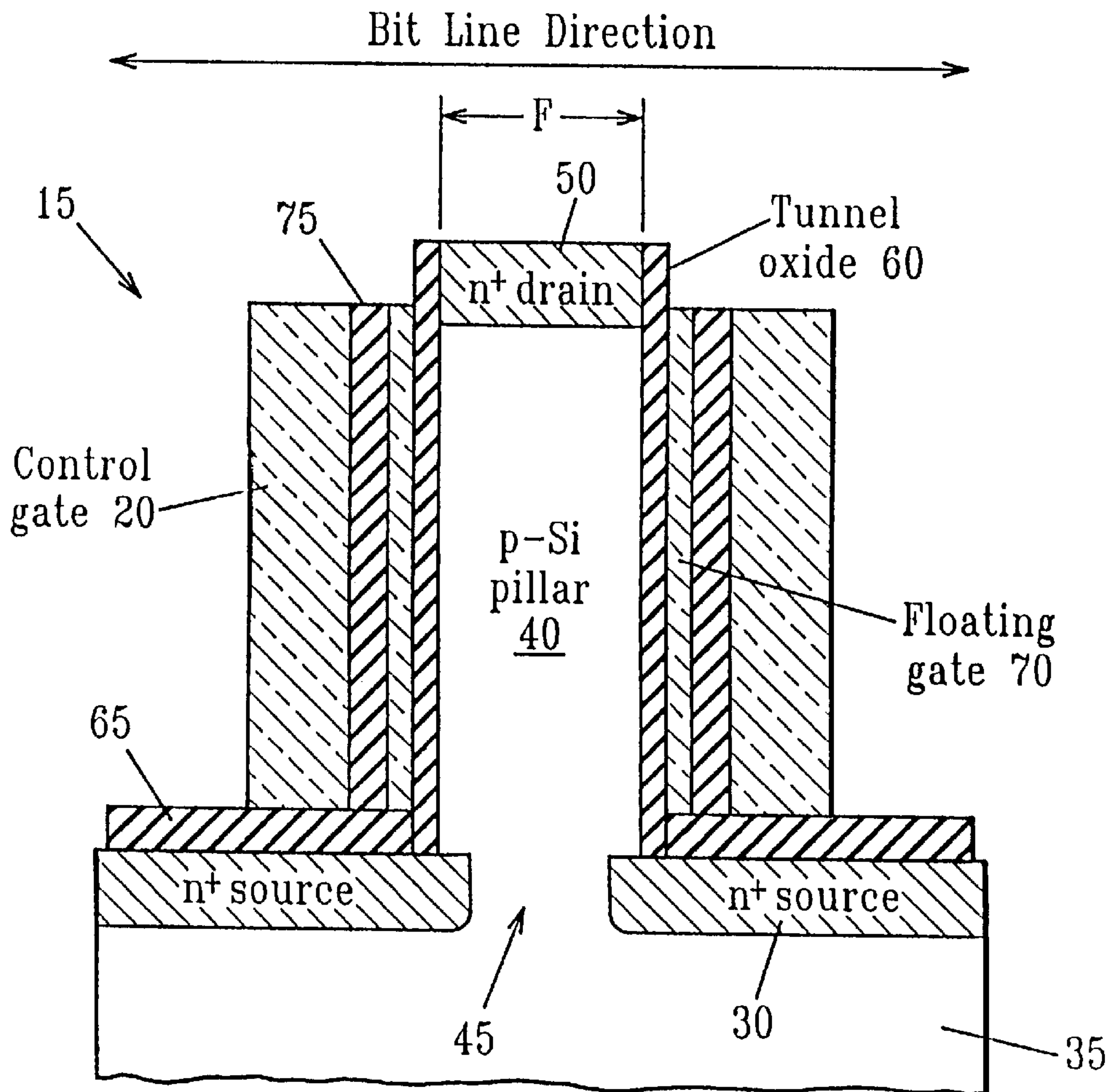
FIG. 3 (PRIOR ART)
