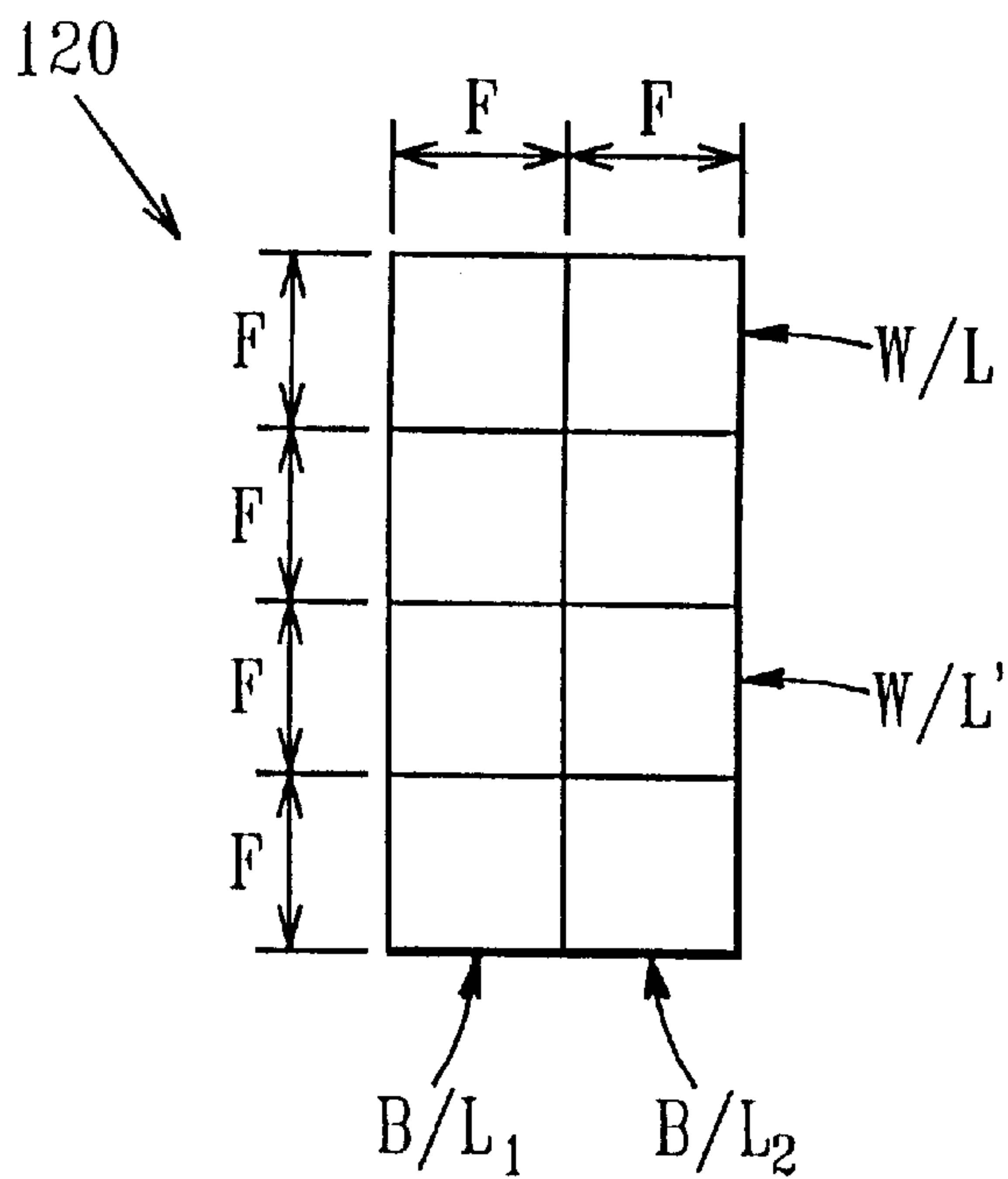
FIG. 6 (PRIOR ART)
