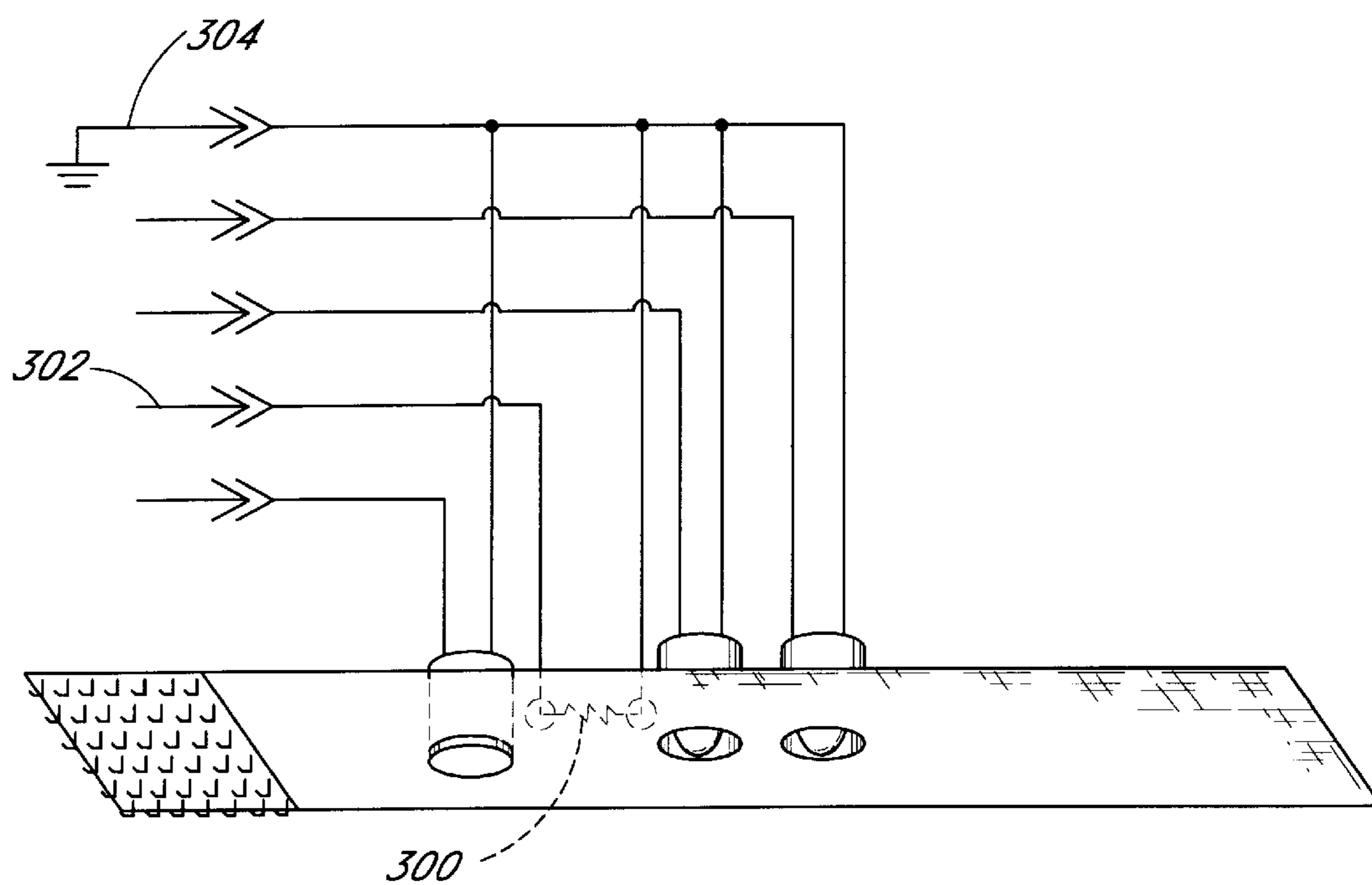
FIG. 1 (PRIOR ART)
