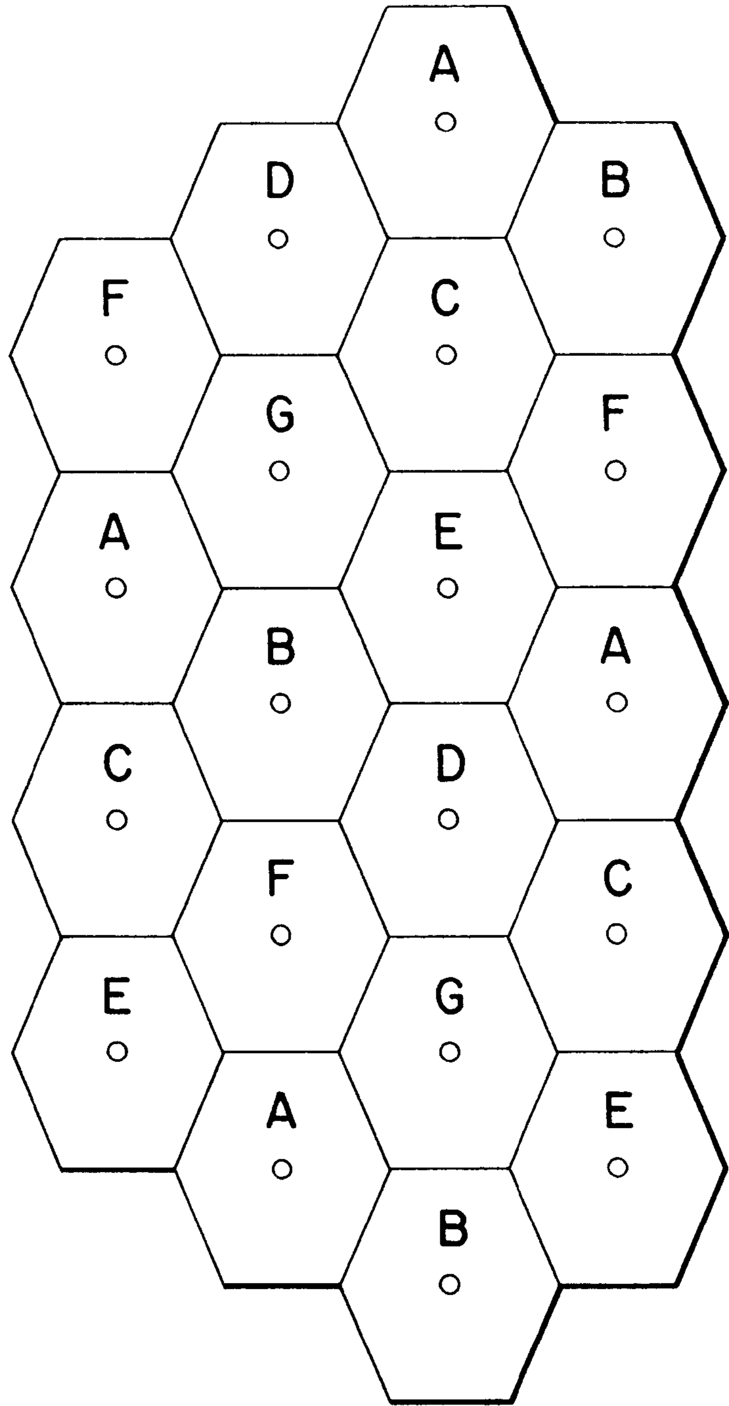
FIG. 1 (PRIOR ART)
