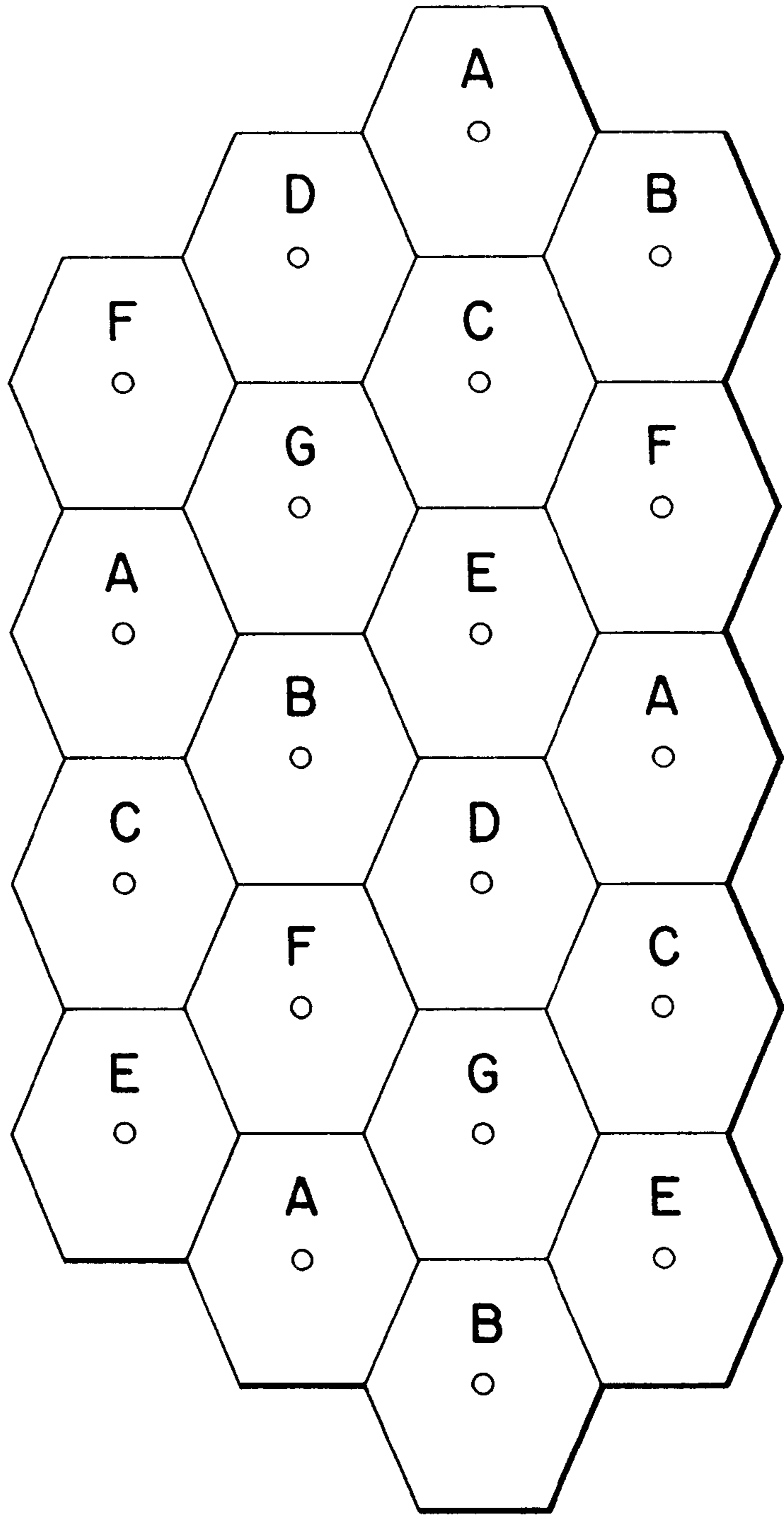
FIG. 1 (PRIOR ART)
