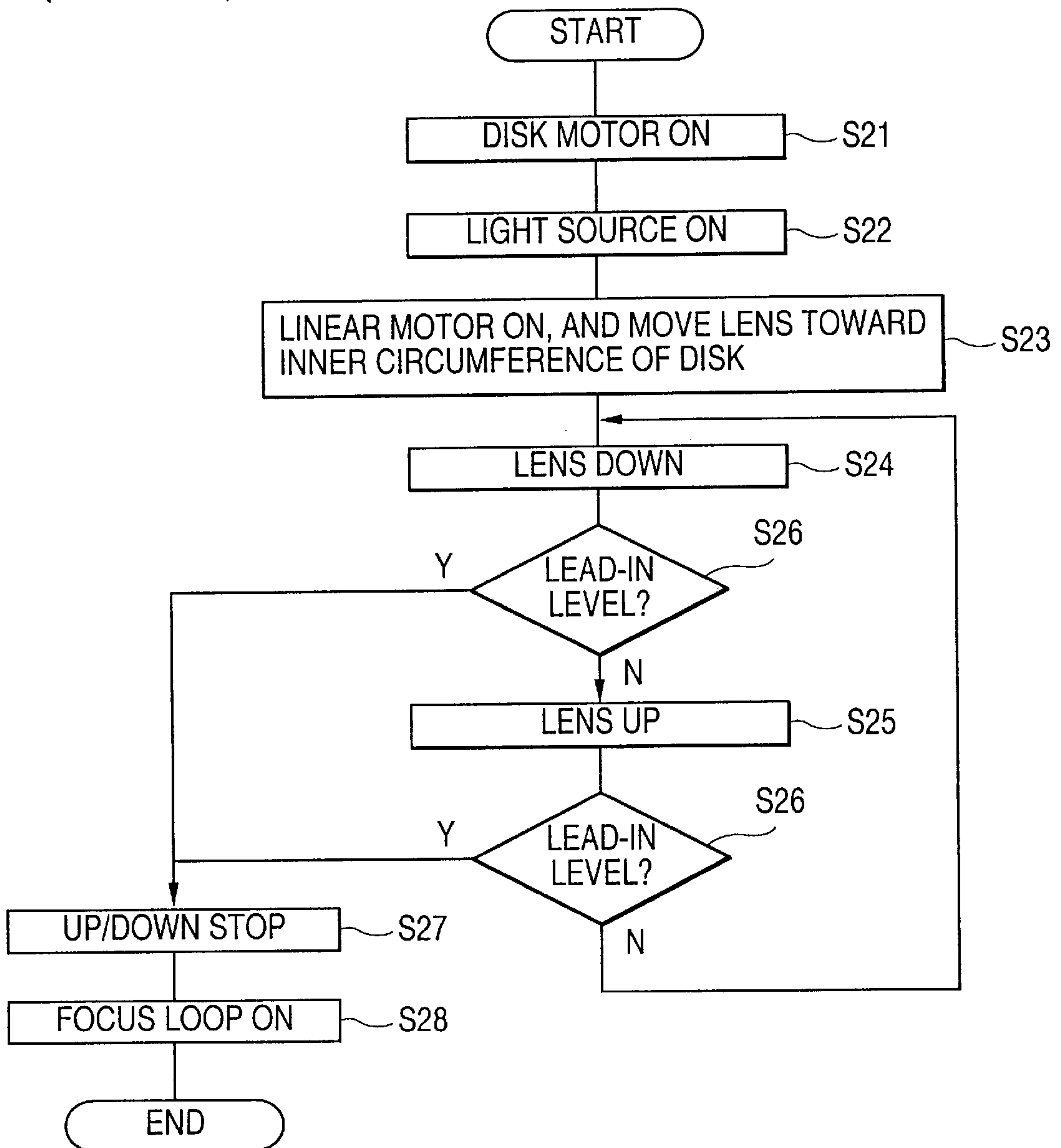
FIG. 22 (PRIOR ART)
