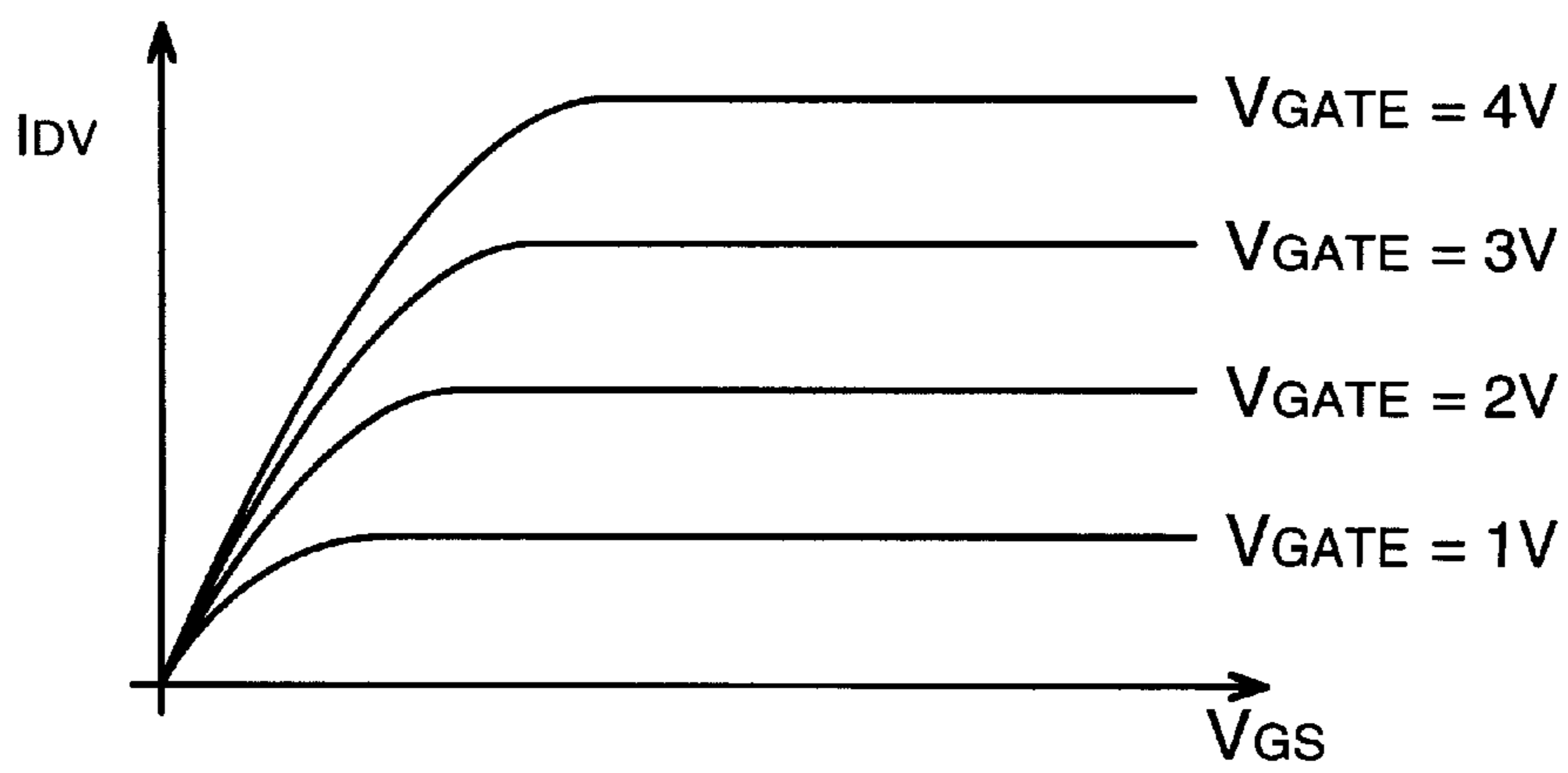
FIG. 3 (PRIOR ART)
