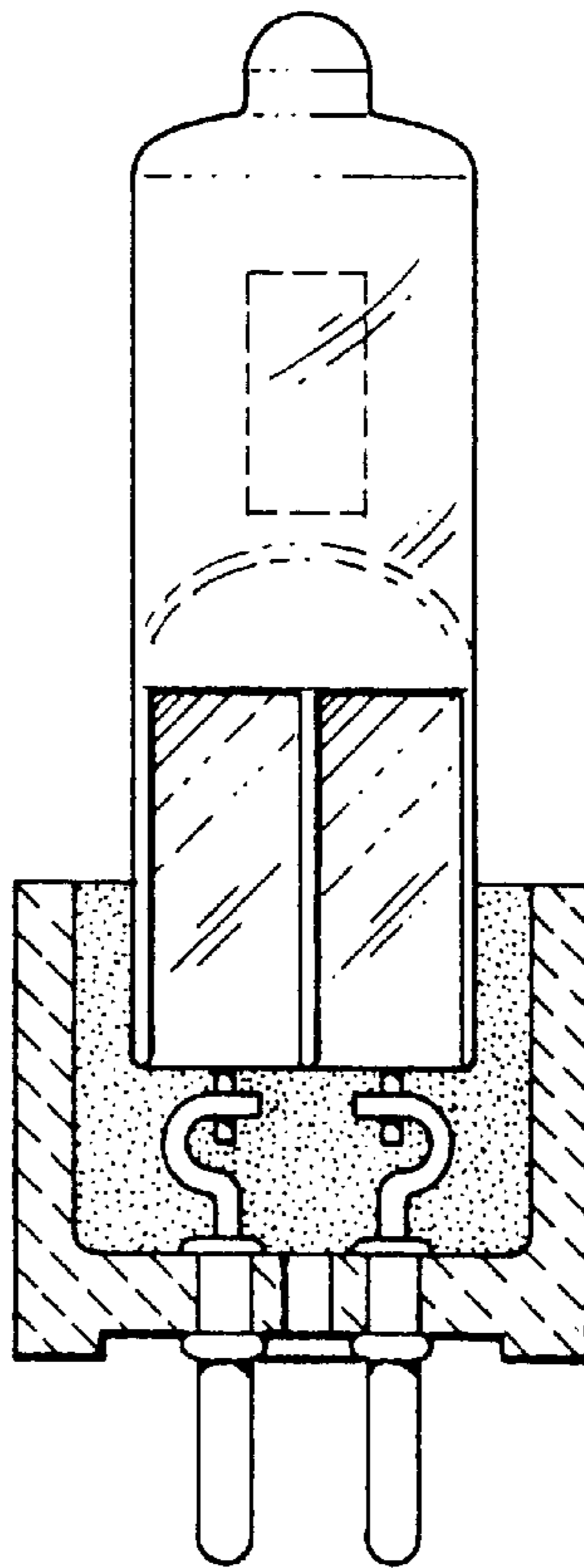
Fig. 2 (PRIOR ART)
