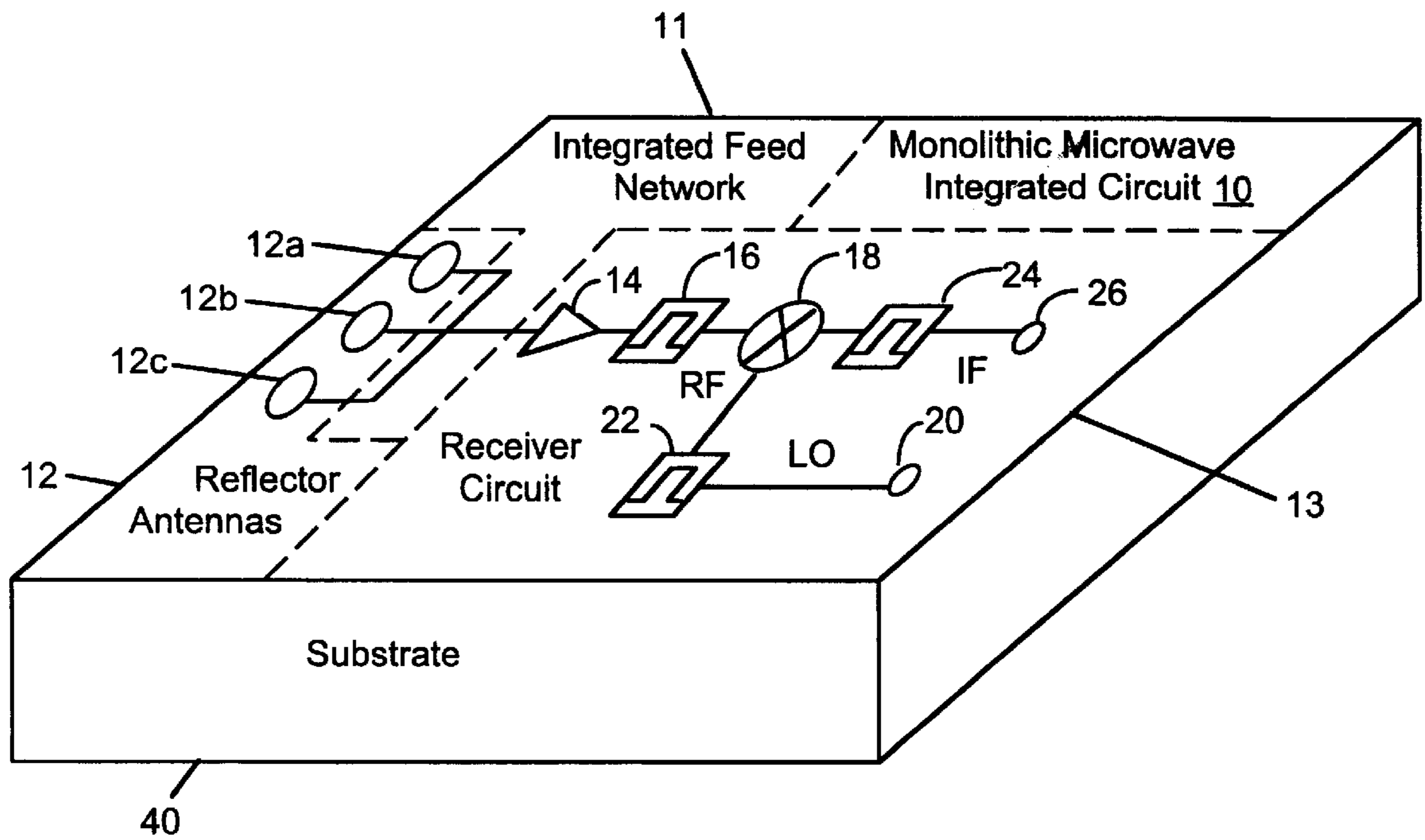
MEMS INTEGRATED RECEIVER
