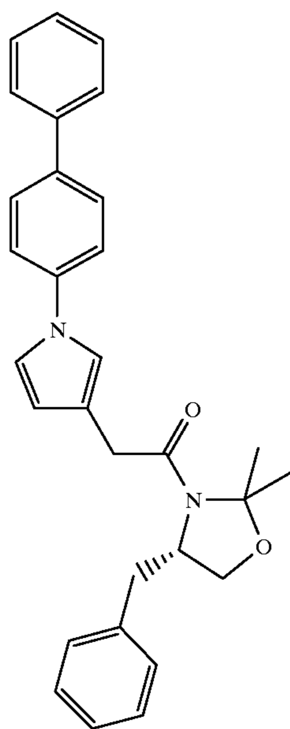
1-(4(S)-benzyl-2,2-dimethyl-oxazolidin-3-yl)-2-[1-(biphenyl-4-yl)-1H-pyrrol-3-yl]-ethanone
