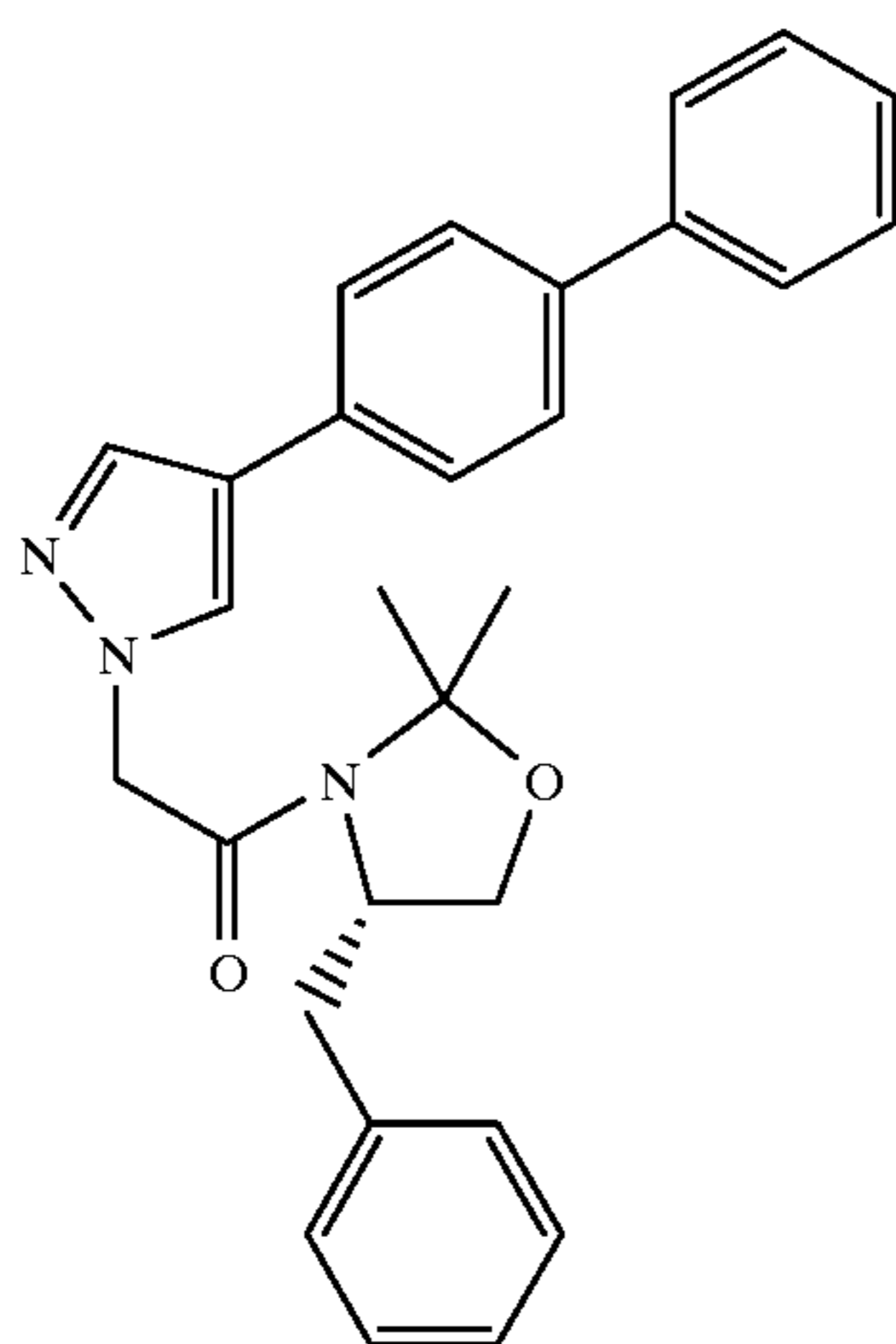
1-(4(S)-Benzyl-2,2-dimethyl-oxazolidinyl)-2-(4-biphenyl-4-yl-pyrazol-1-yl)-ethanone
