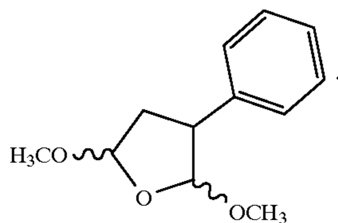
2,5-Dimethoxy-3-phenyl-tetrahydrofuran
