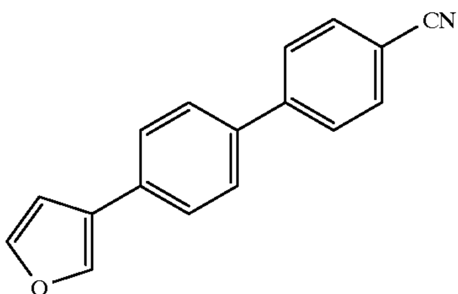
4'-(Furan-3-yl)-biphenyl-4-carbonitrile
