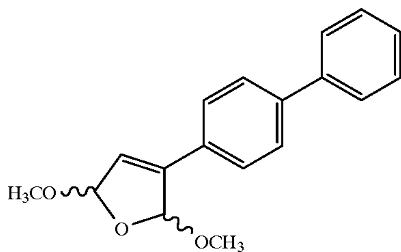
3-(Biphenyl-4-yl)-2,5-dihydro-2,5-dimethoxyfuran
