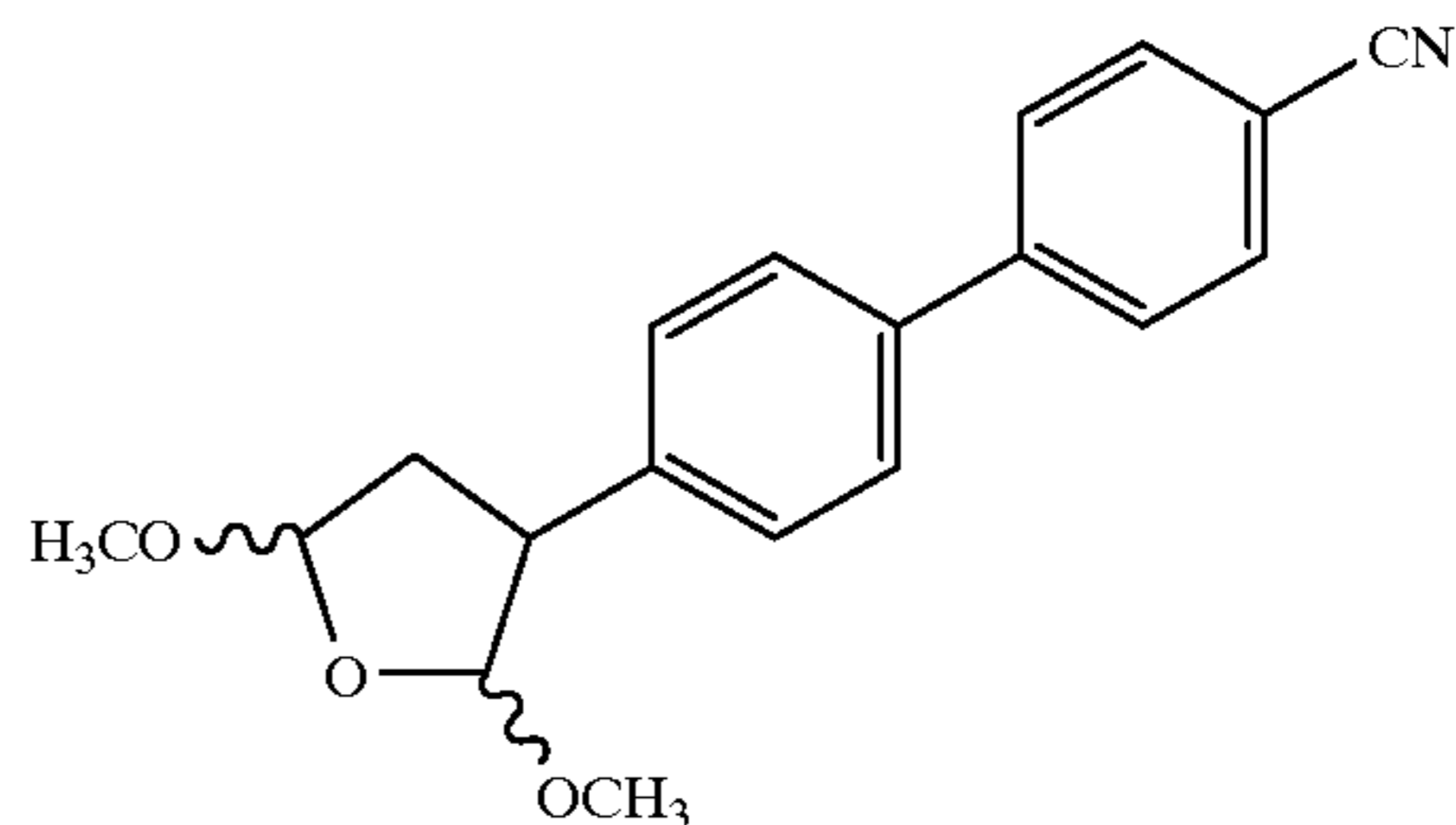
4'-(2,5-Dimethoxy-tetrahydrofuran-3-yl)-biphenyl-4-carbonitrile
