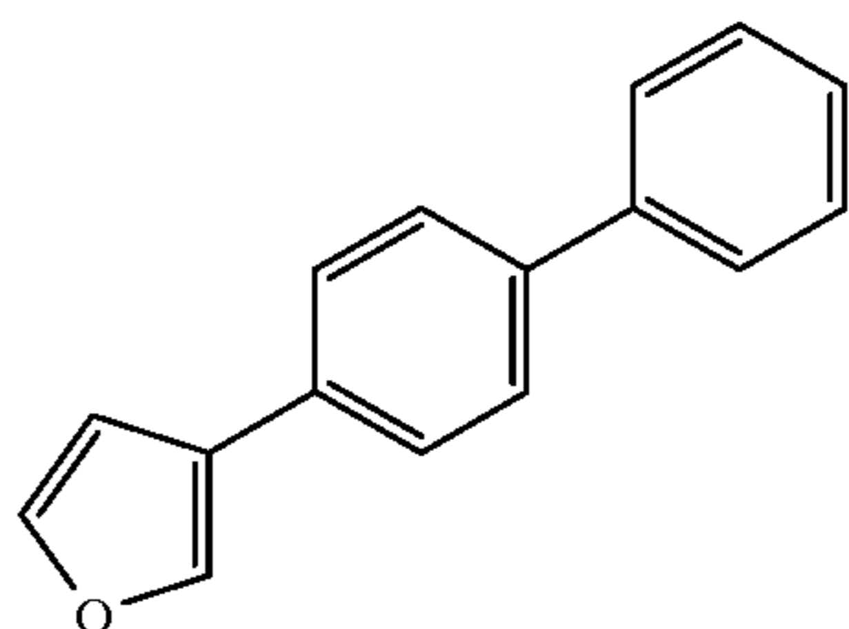
3-(Biphenyl-4-yl)furan
