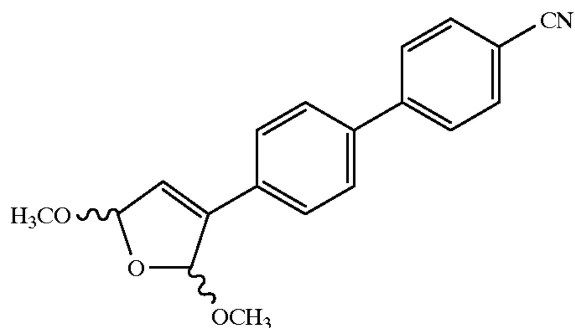
4'-(2,5-Dimethoxy-2,5-dihydro-furan-3-yl)-biphenyl-4-carbonitrile
