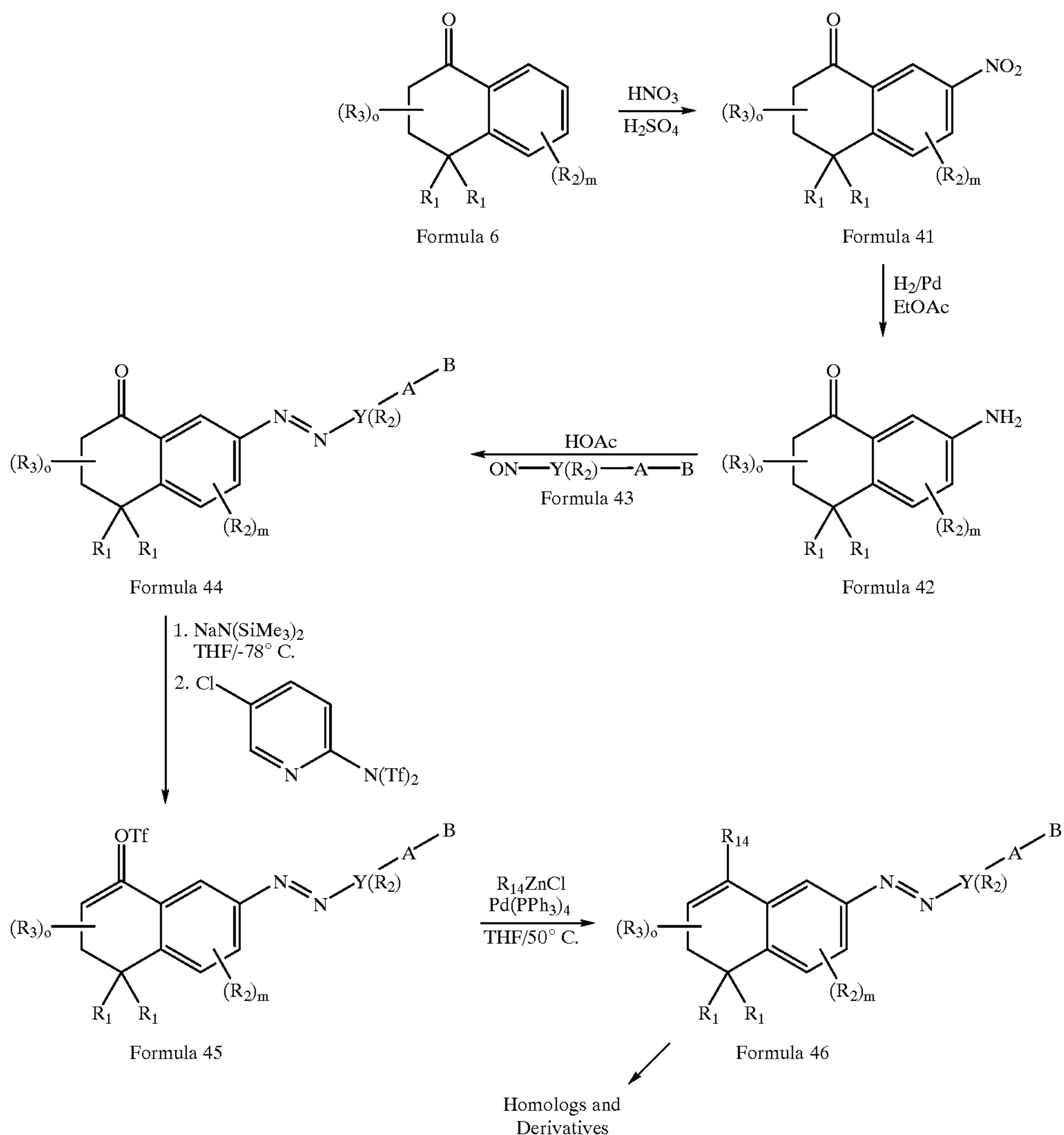
Reaction Scheme 5
