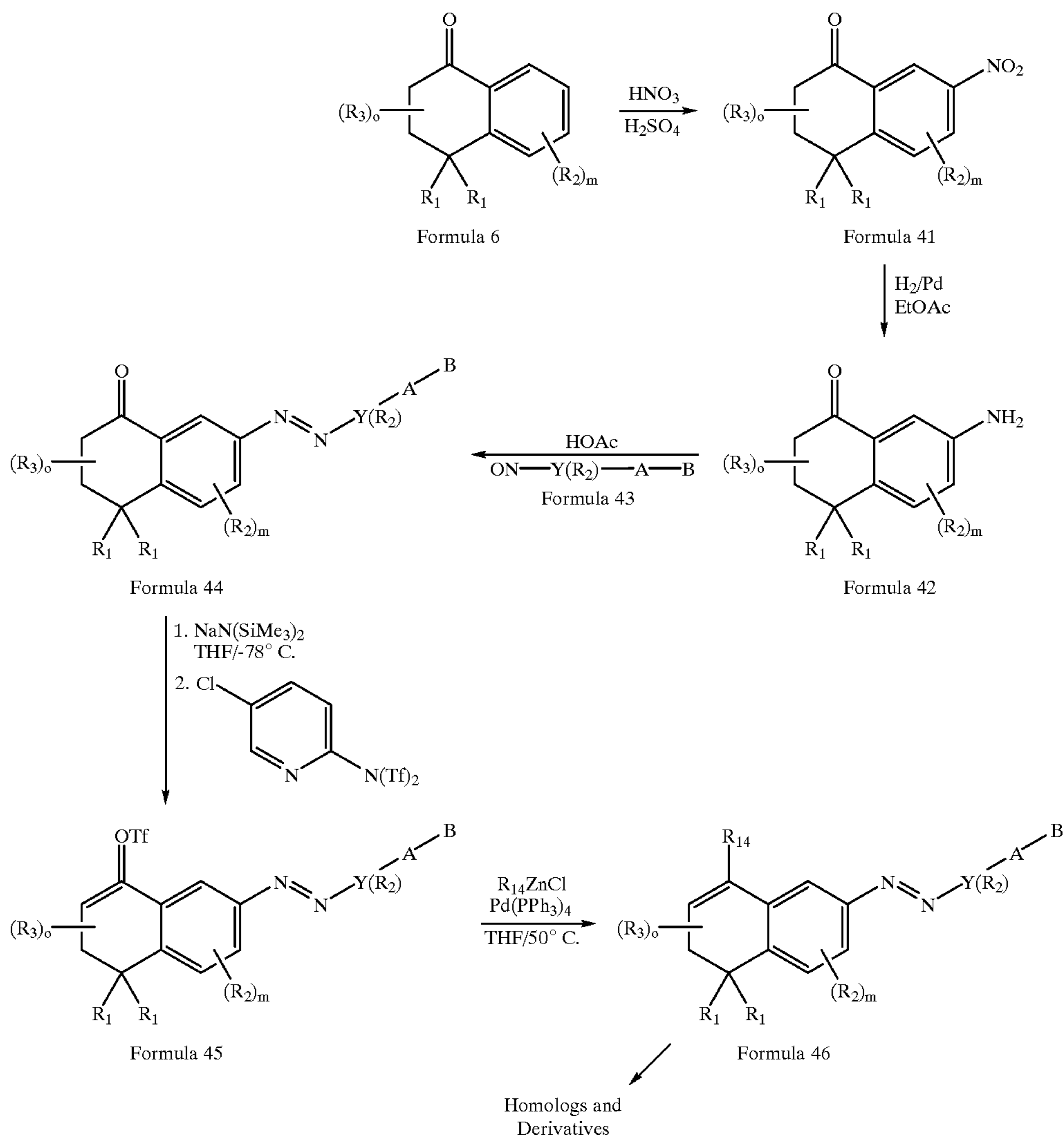
Reaction Scheme 5
