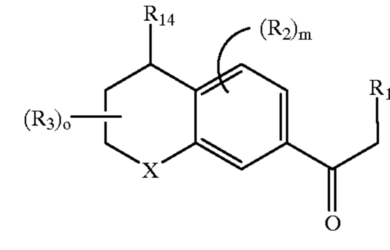
FORMULA 127
