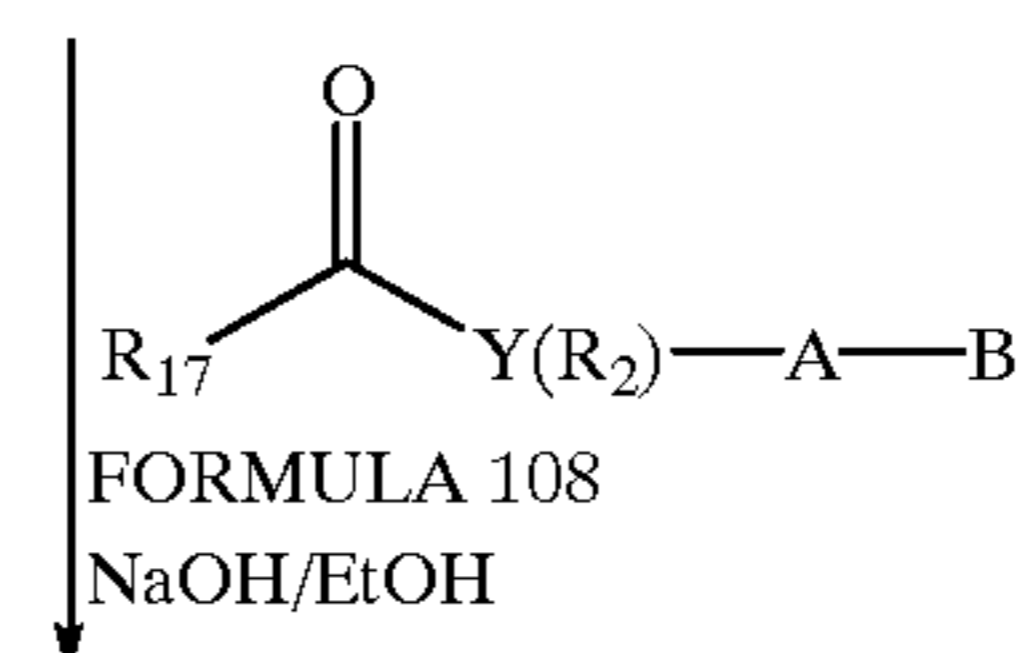
FORMULA 127
