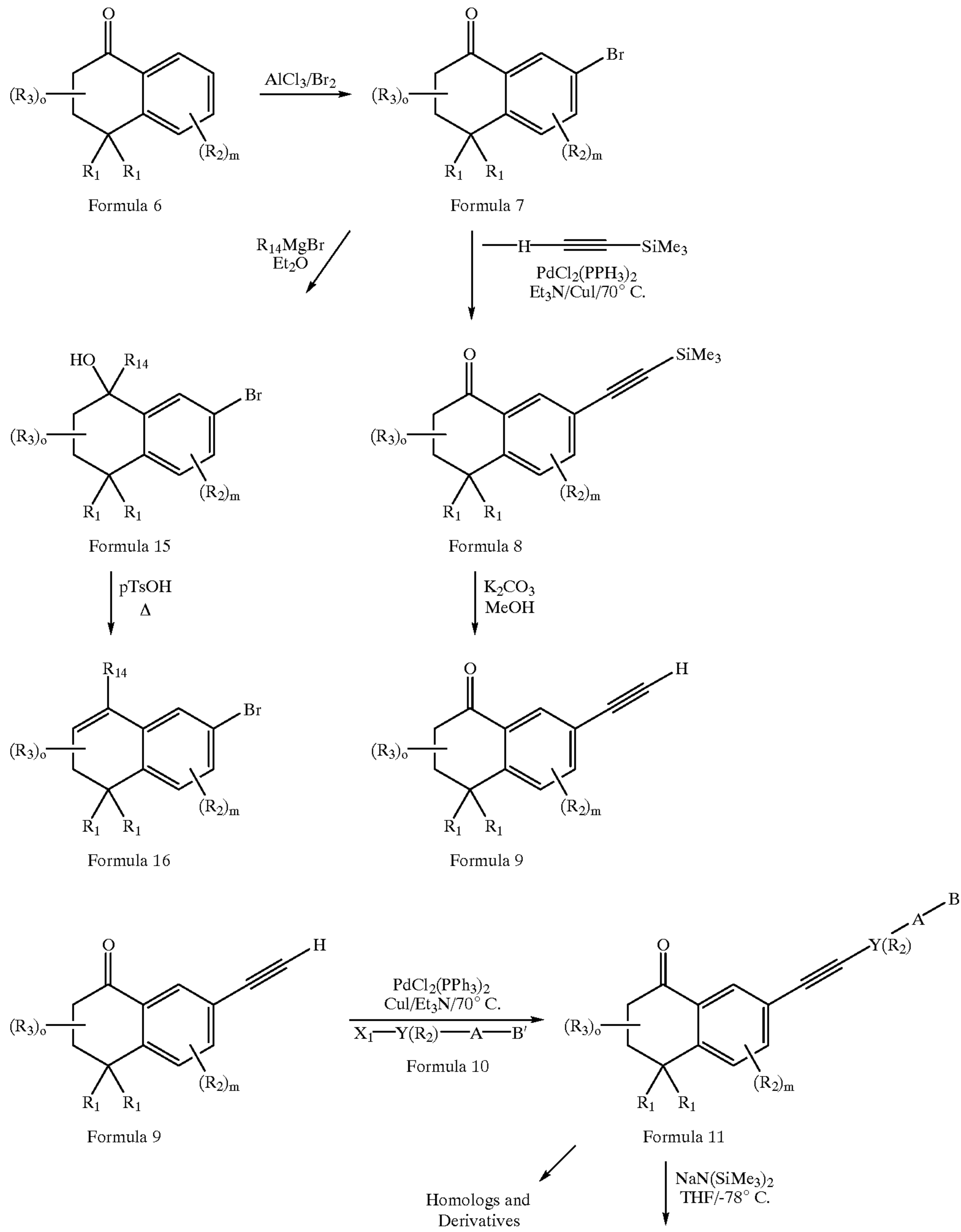
Reaction Scheme 1
