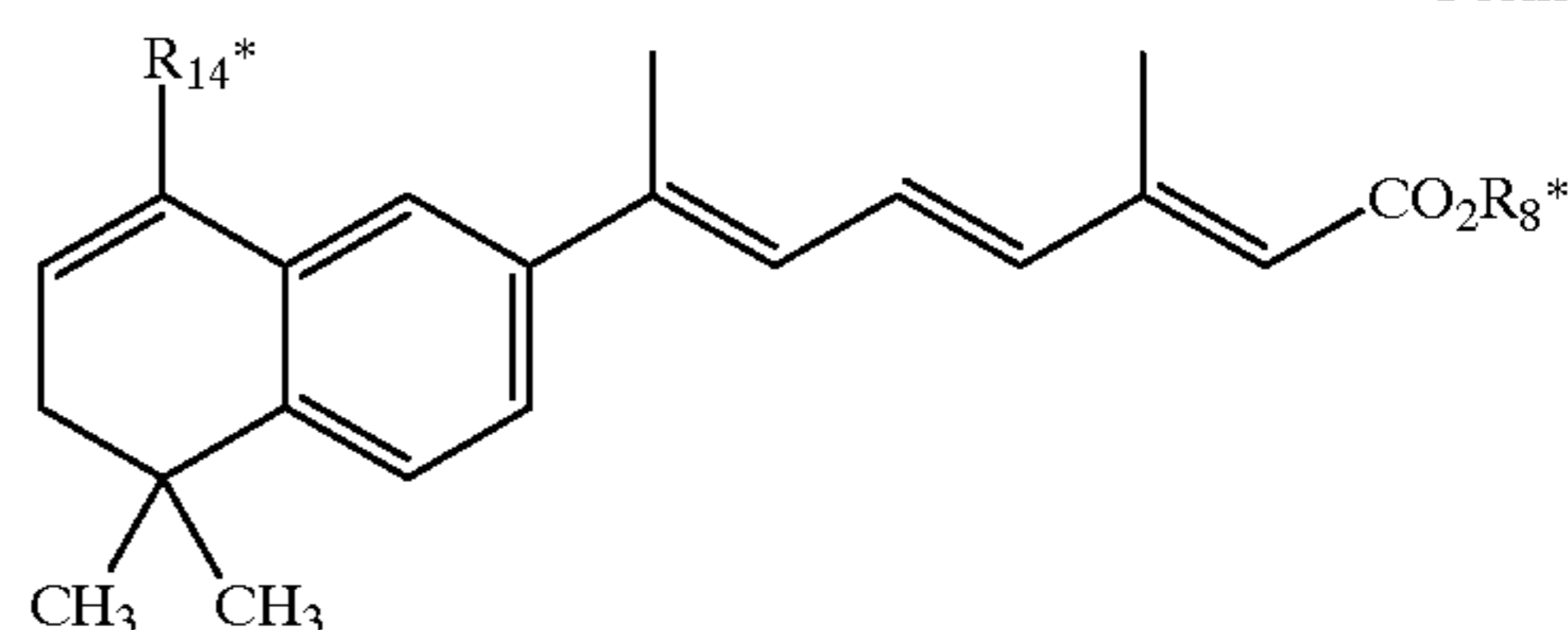
Formula 5a
