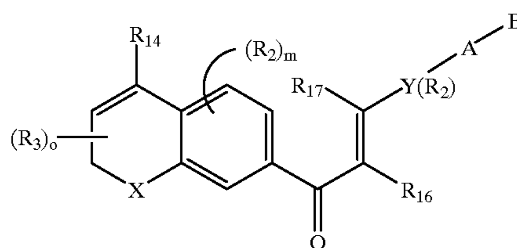
FORMULA 128
