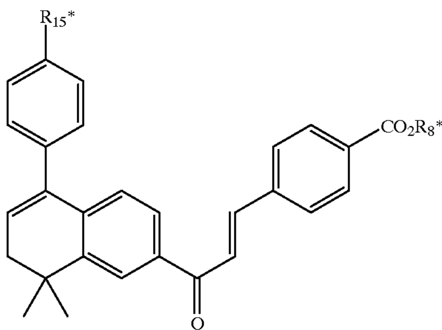
Formula 102
