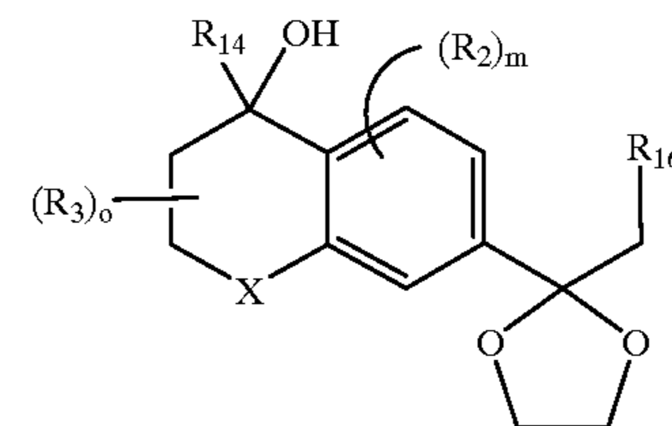
FORMULA 126
