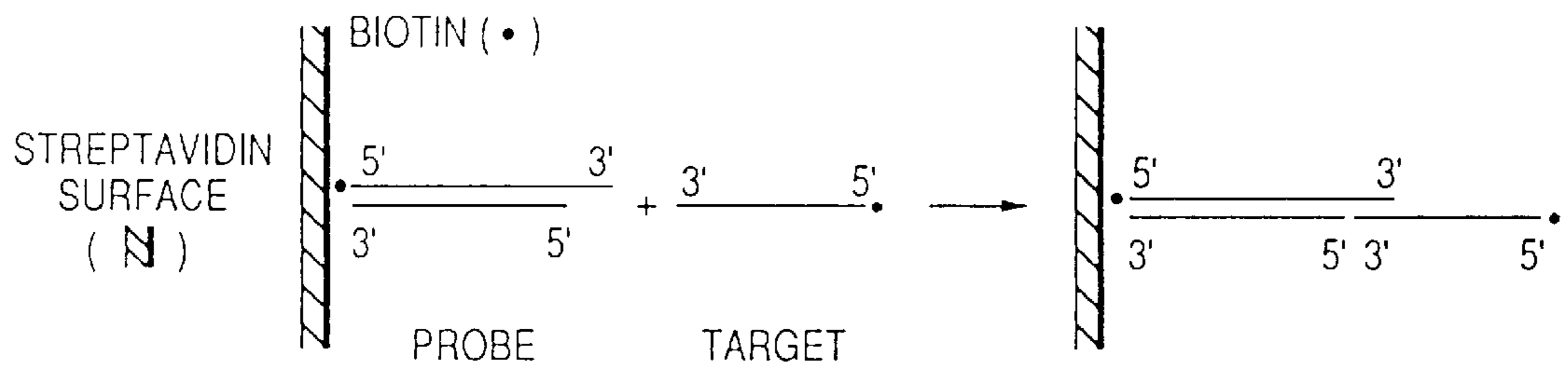
BASIC SCHEME FOR POSITIONAL SBH
