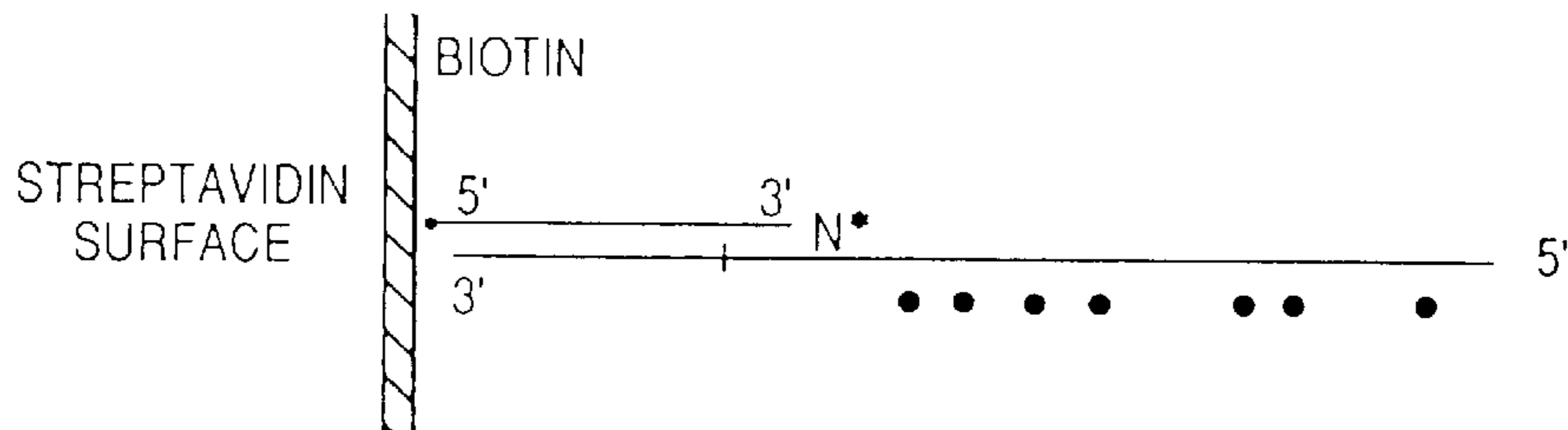
POSITIONAL INFORMATION FROM RATIO OF INTERNAL LABEL (•) TO EXTENSION LABEL (•). A 5' LABEL COULD ALSO BE USED.
