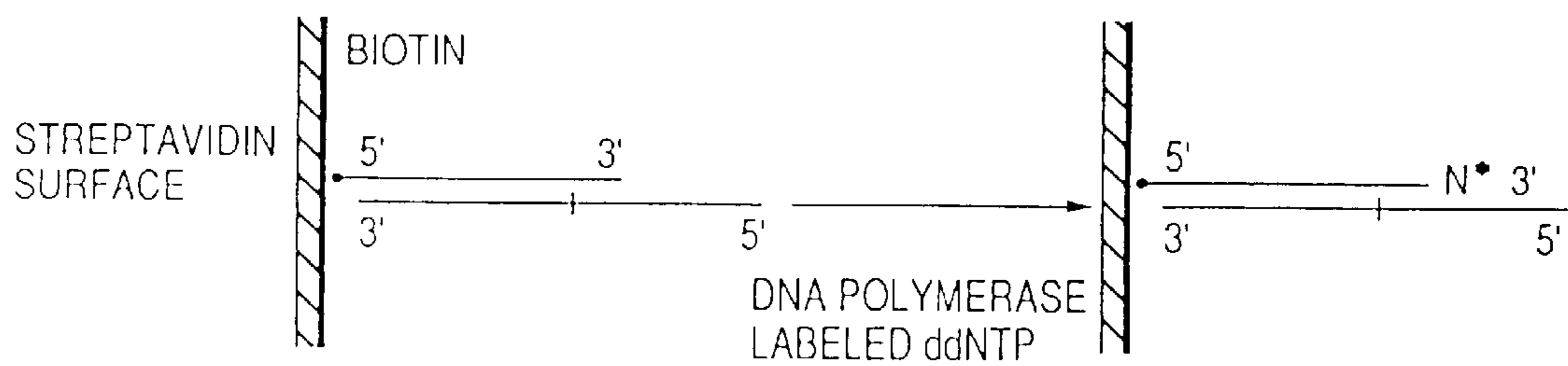
READING AN EXTRA TARGET BASE BY 3' EXTENSION OF THE PROBE
