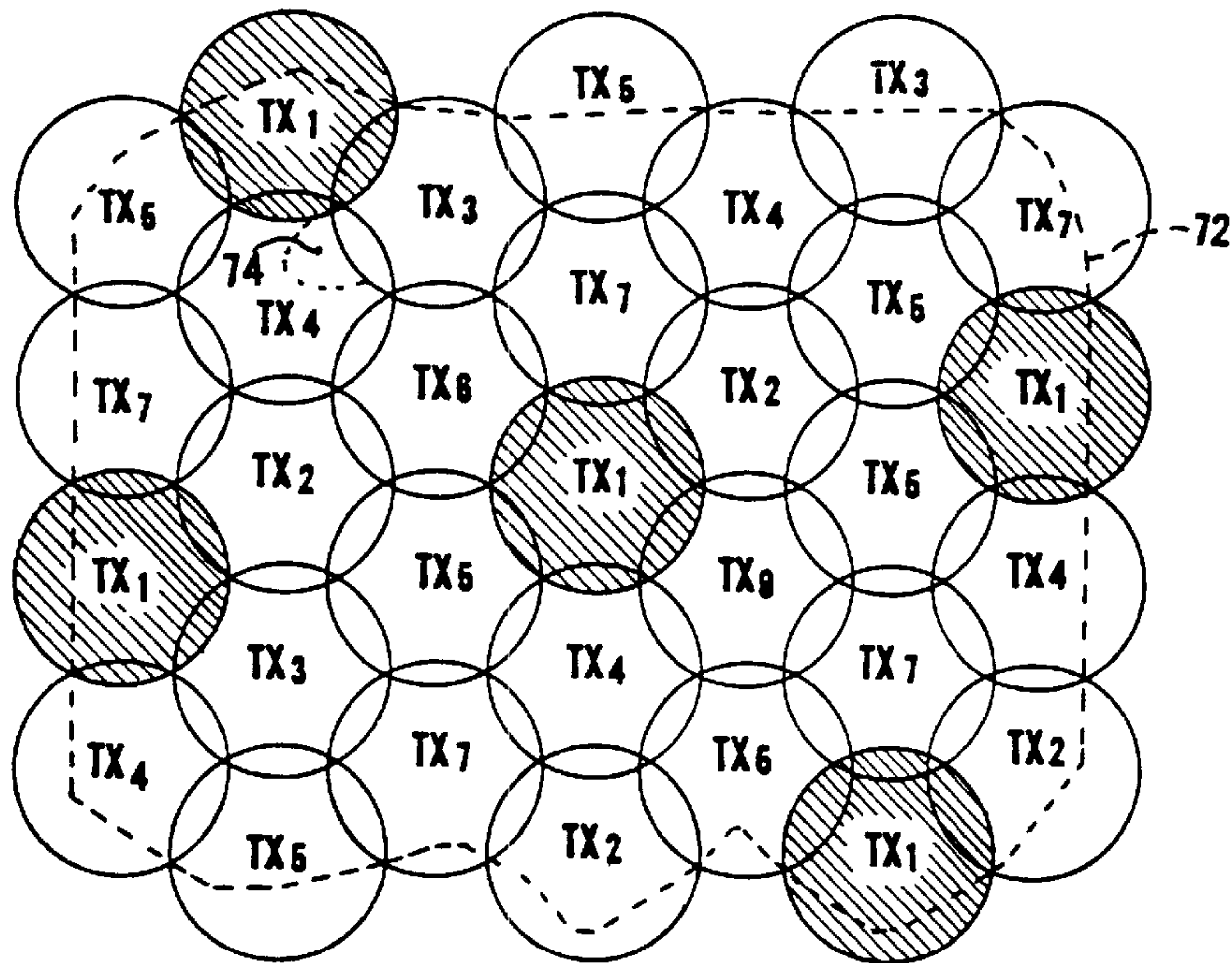
FIGURE 2 (PRIOR ART)
