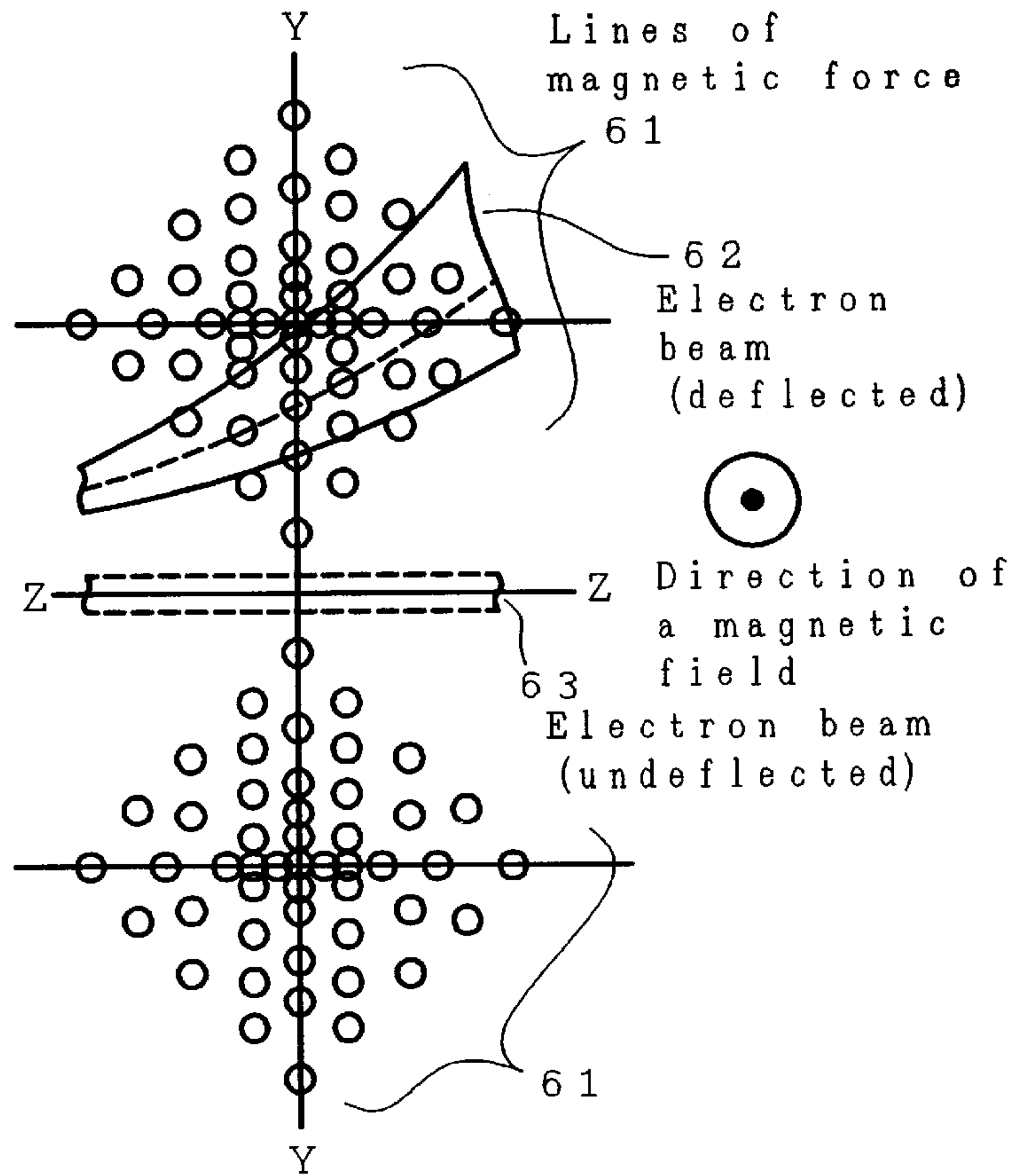
Direction of an electron beam travel
