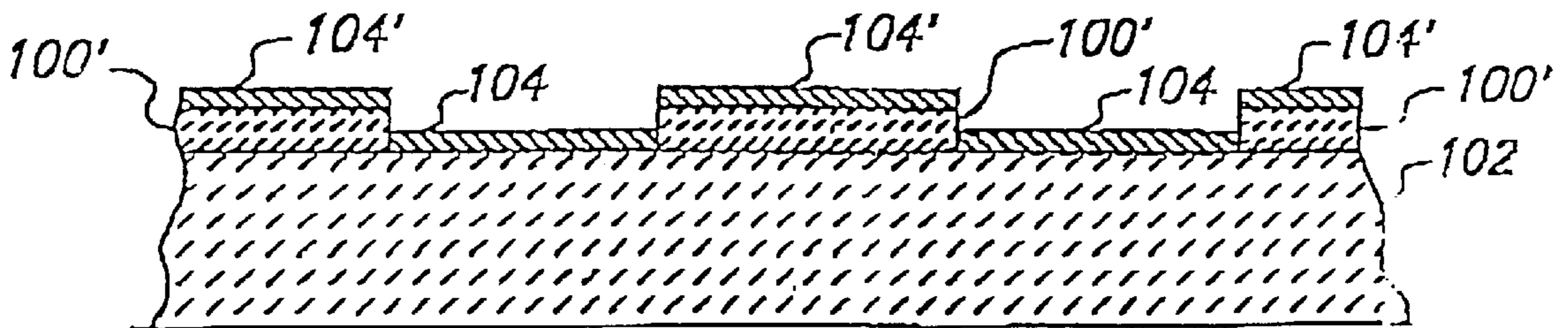
FIG. 2 (PRIOR ART)
