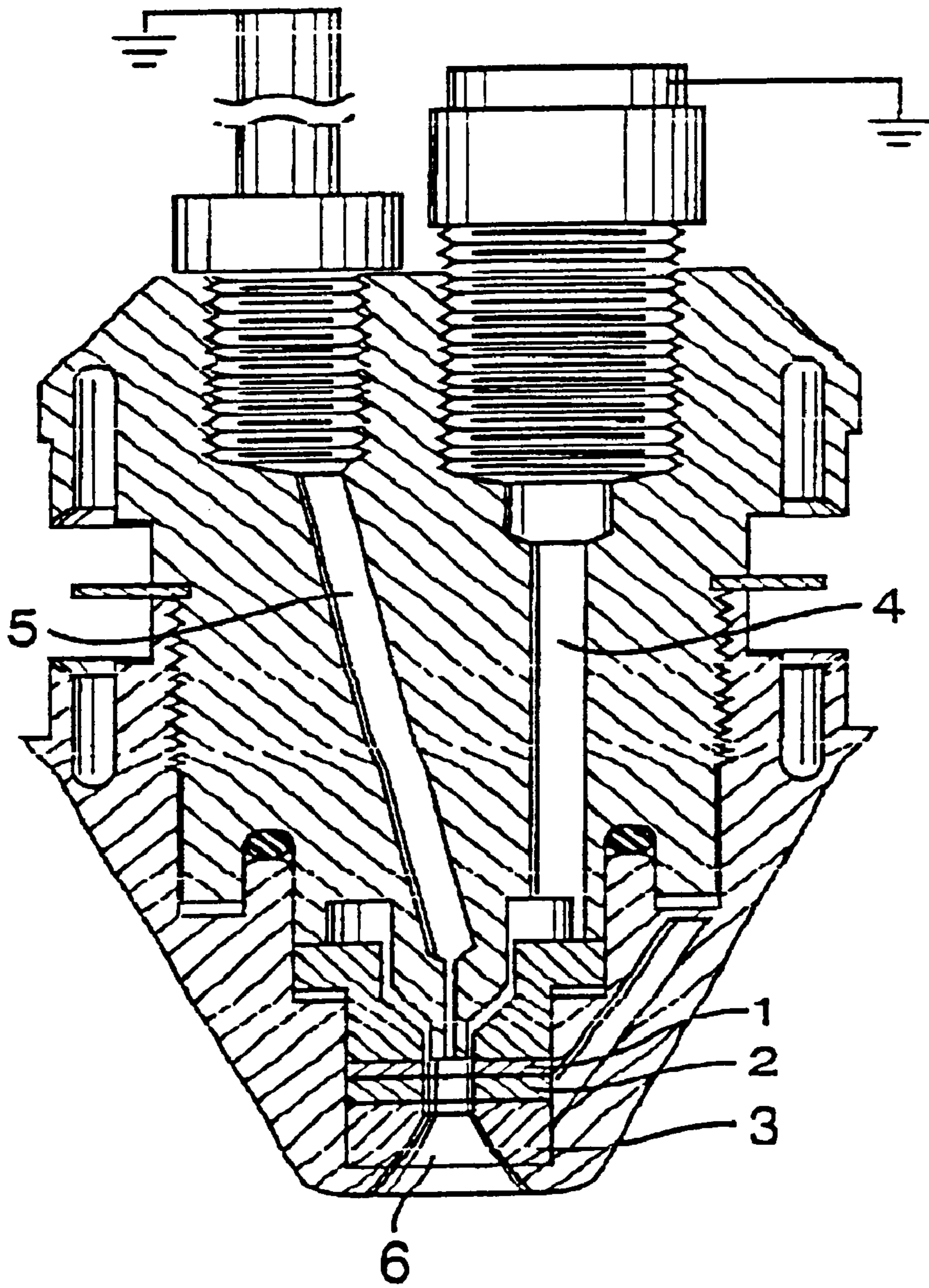
FIG. 1 (Prior Art)
