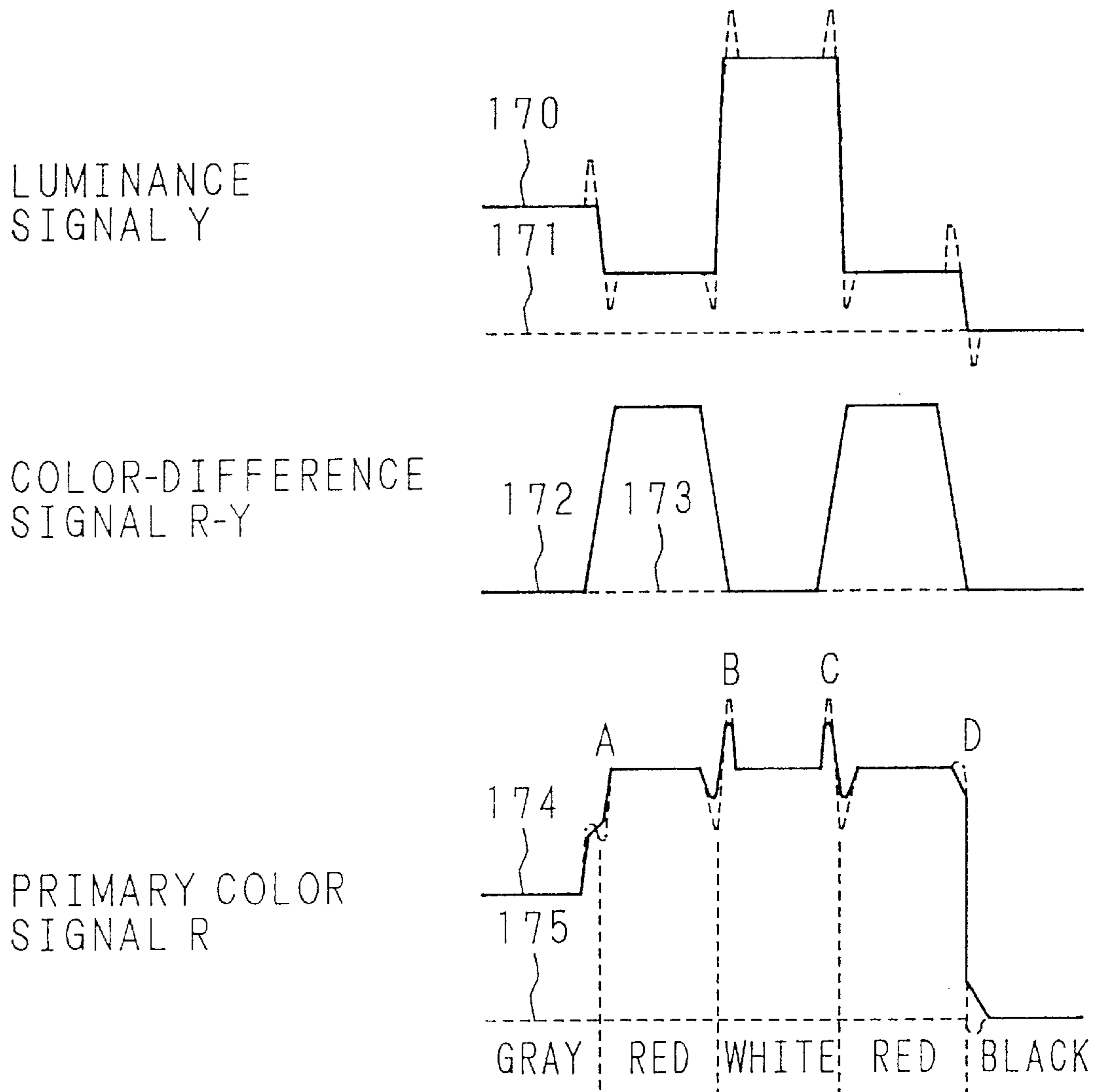
Fig. 2 Prior Art
