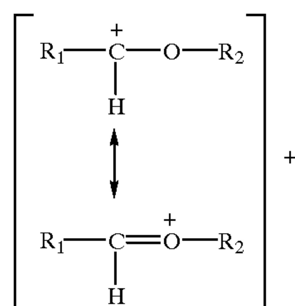
Carbocation cation (1)
