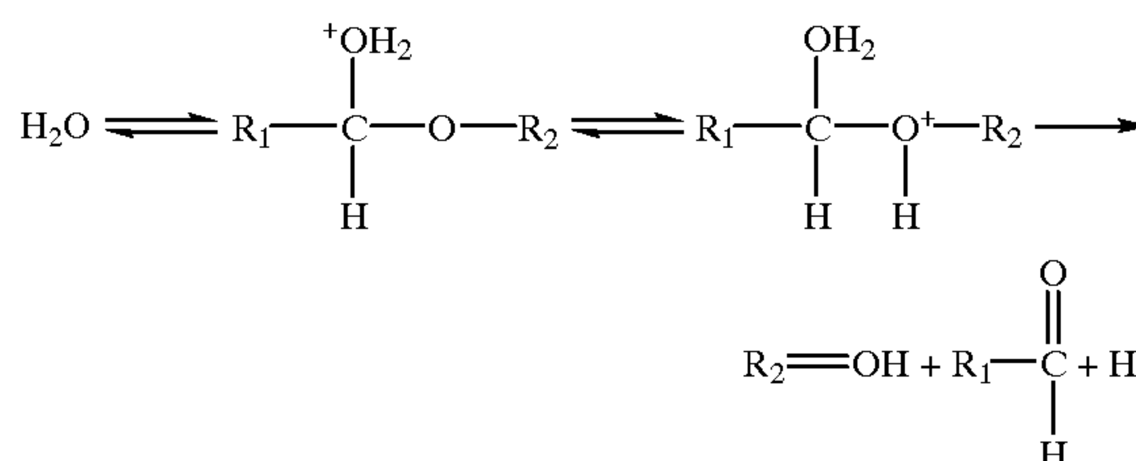
Carbocation cation (1)
