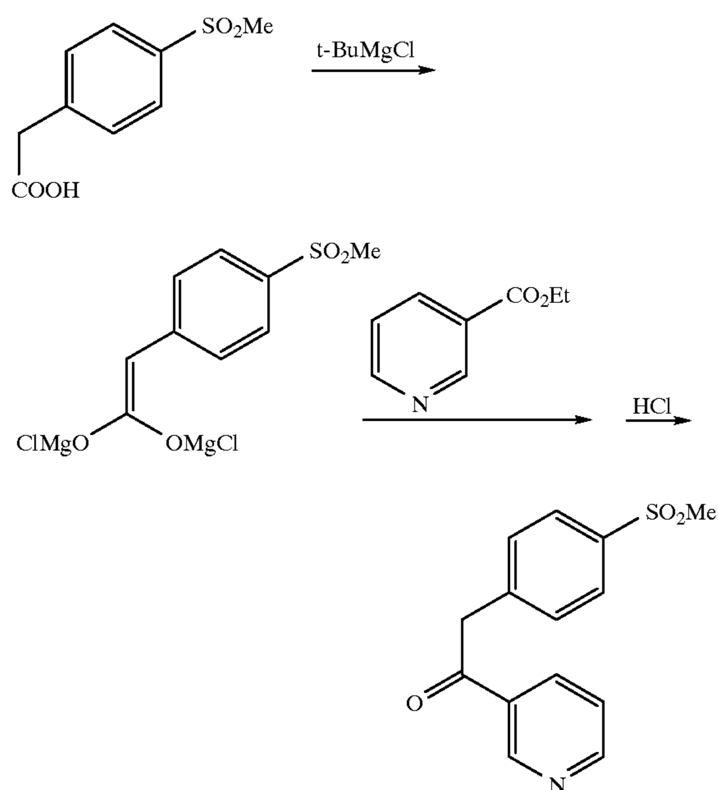
(4-Methylsulfonyl)benzyl-3-pyridylketone from ethyl nicotinate and (4-methylsulfonyl)phenylacetic acid
