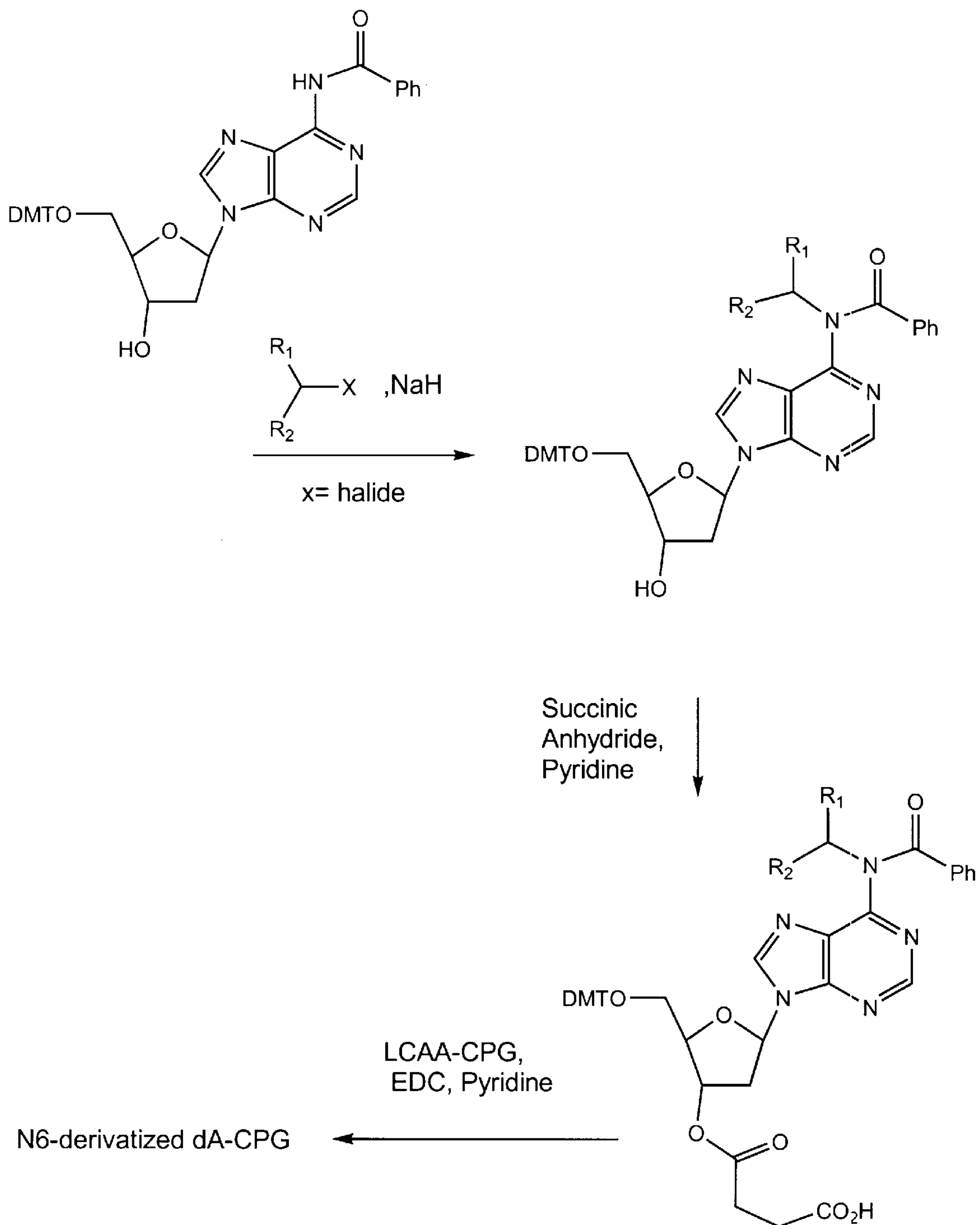
FIGURE 6 Synthesis of derivatized dA CPG
