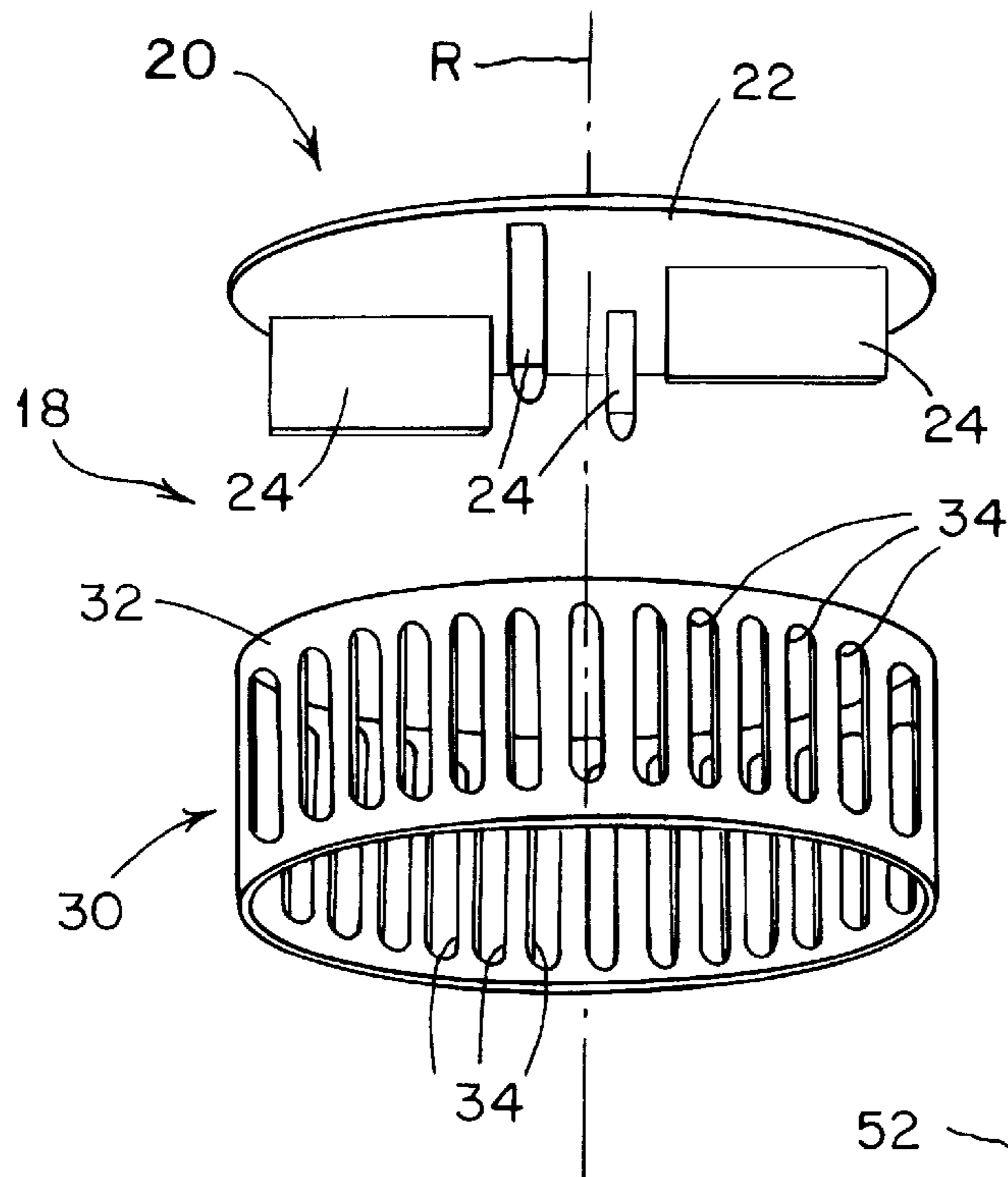
FIG. 2 (PRIOR ART)
