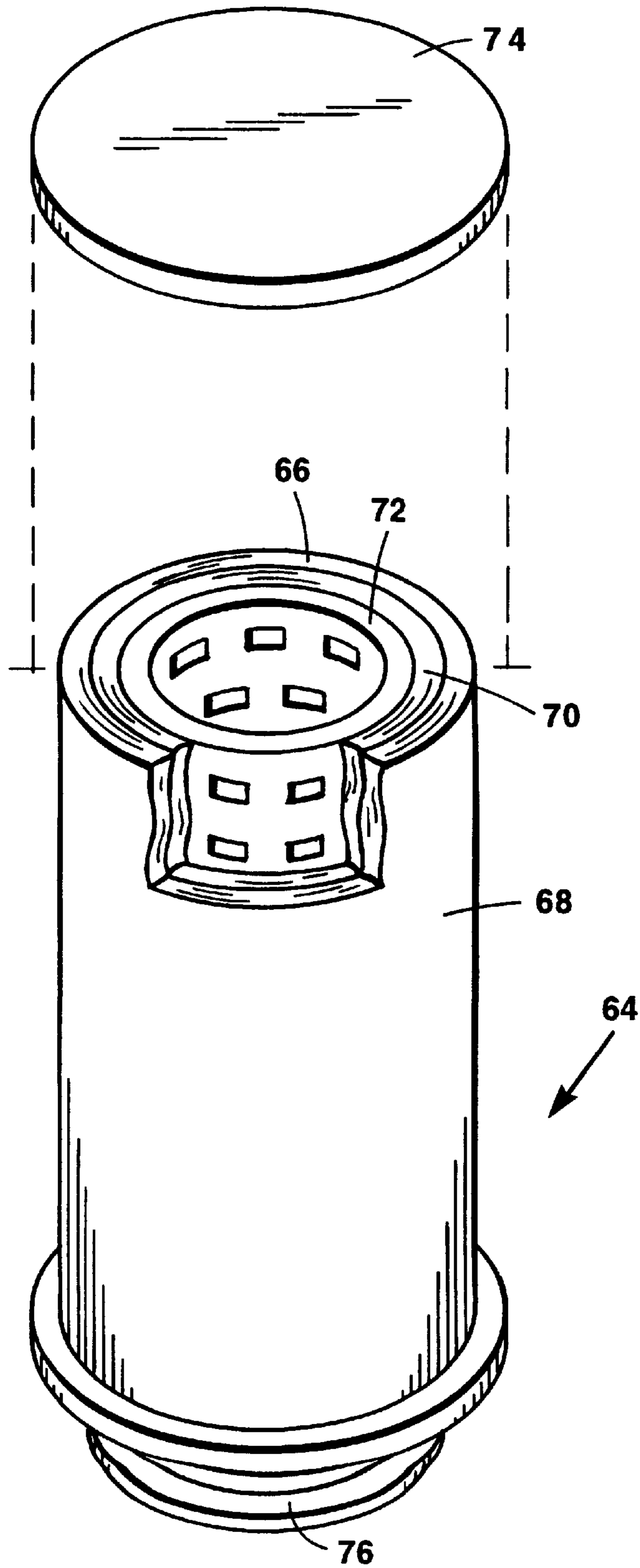
Fig. 6 PRIOR ART
