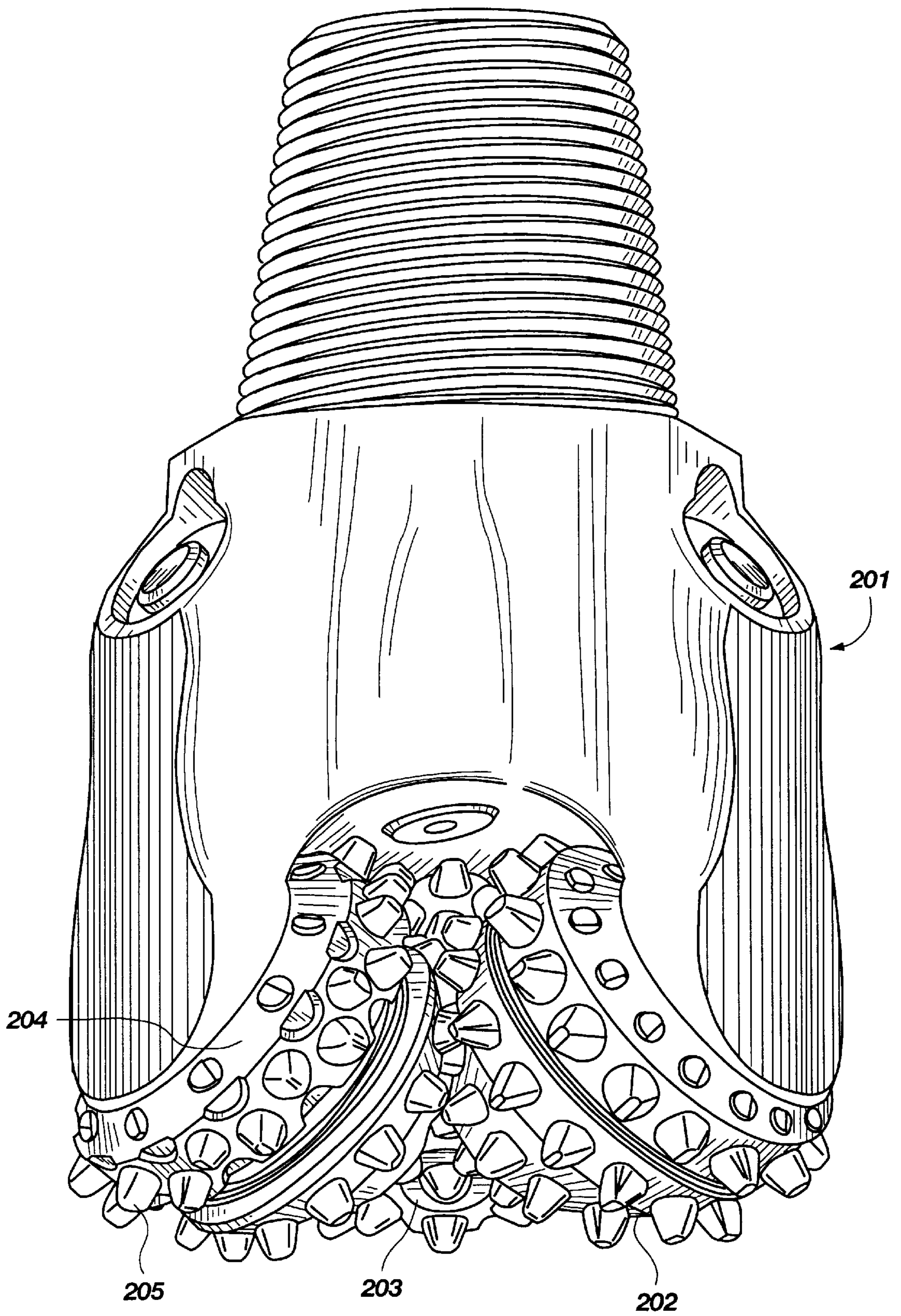
Fig. 2 (PRIOR ART)
