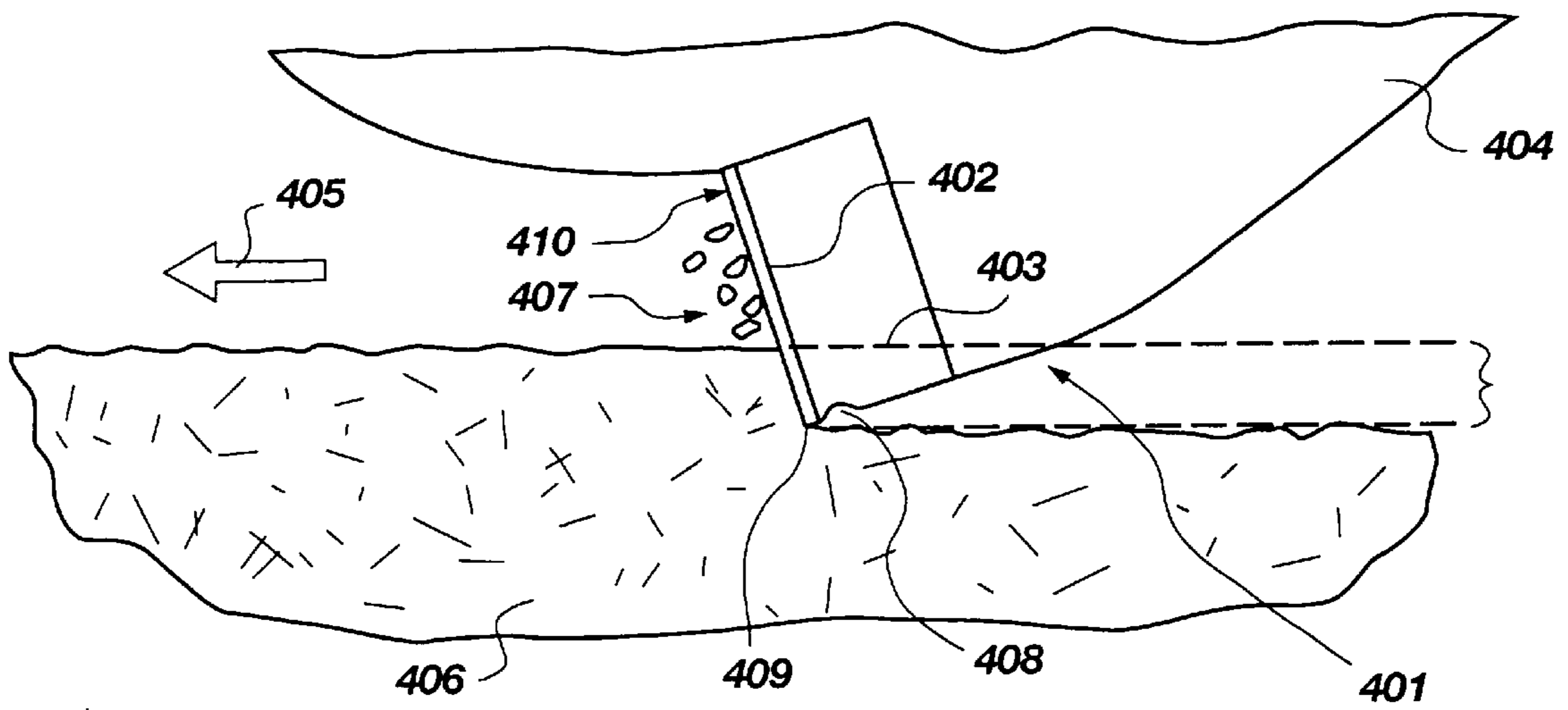
Fig. 4 (PRIOR ART)
