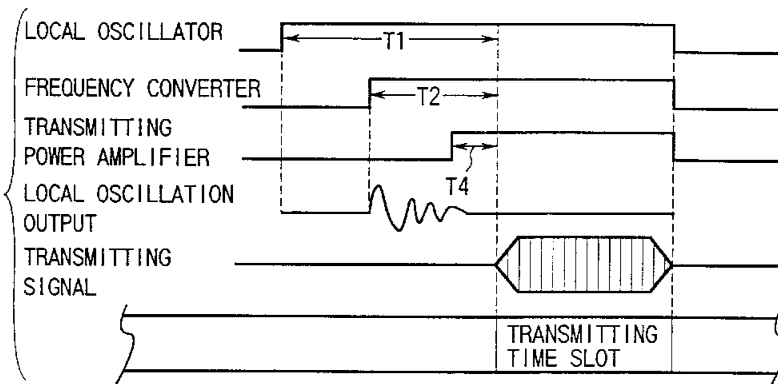
TIME CHART AT TRANSMITTING TIME
