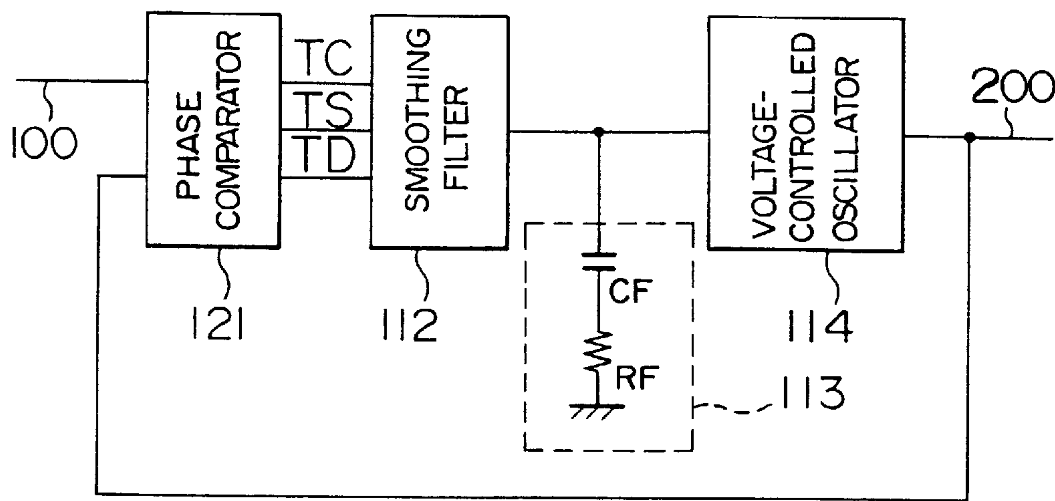
FIG. 22 PRIOR ART
