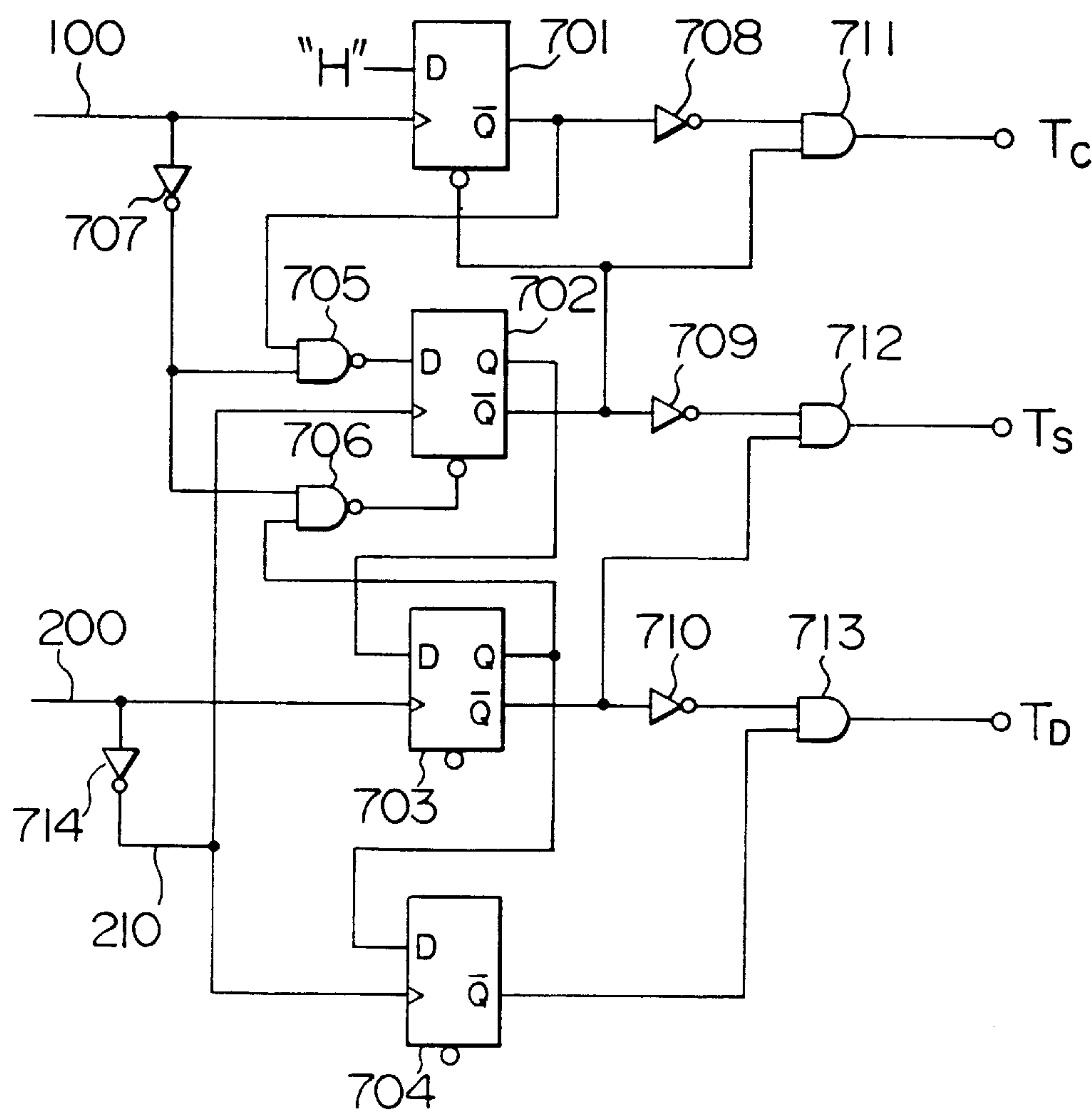
FIG. 23 PRIOR ART
