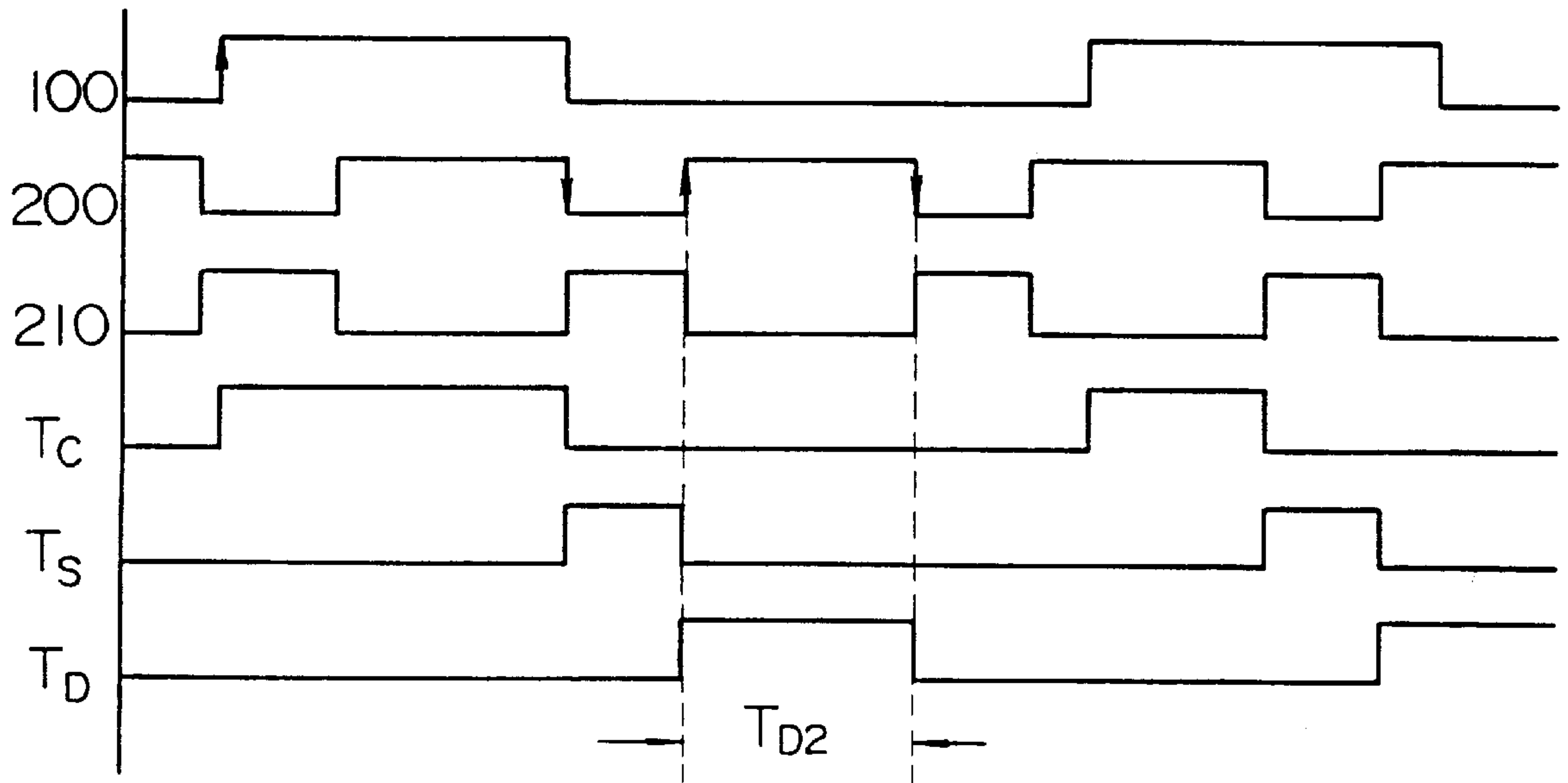
FIG. 25 PRIOR ART
