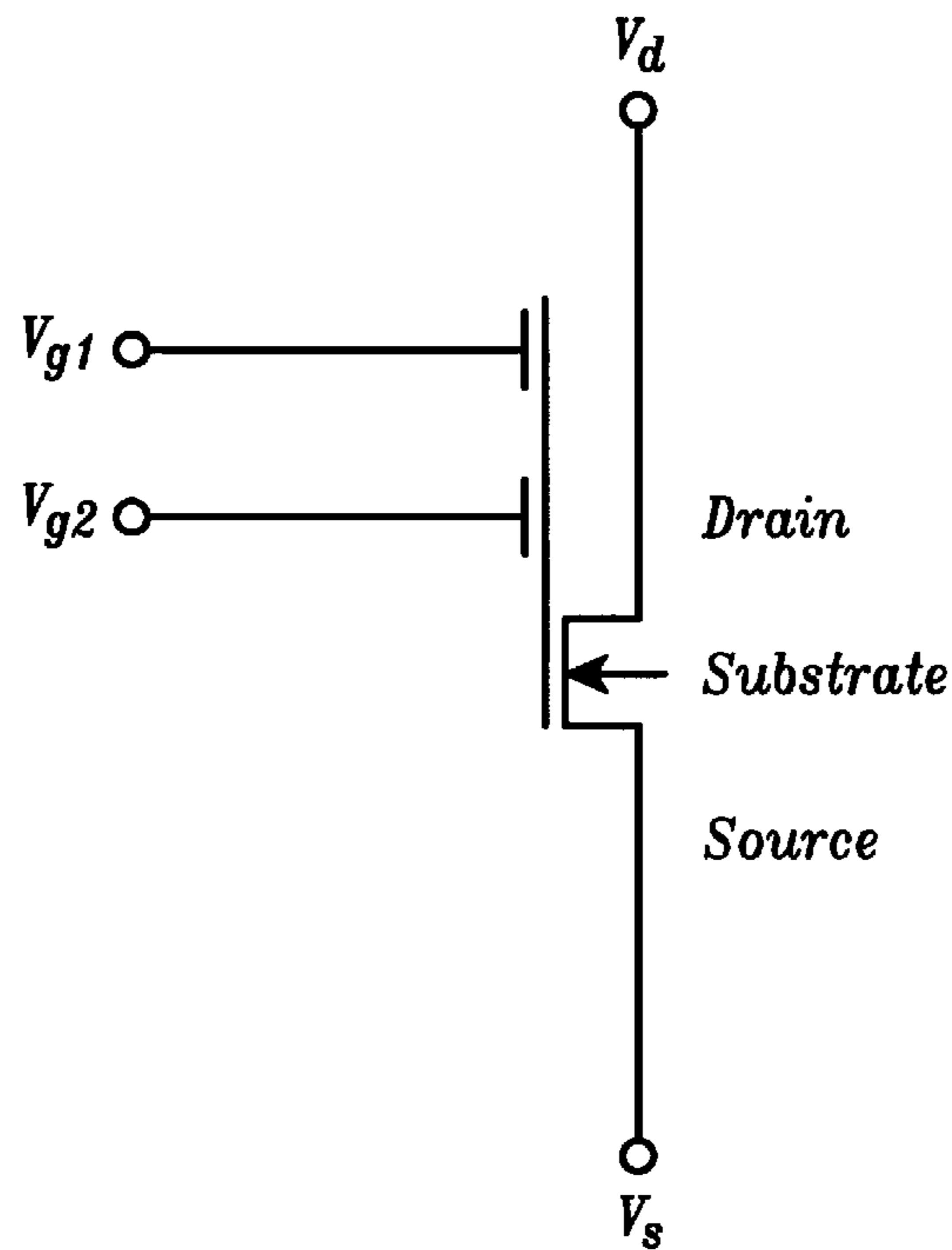
FIG. 25 (PRIOR ART)
