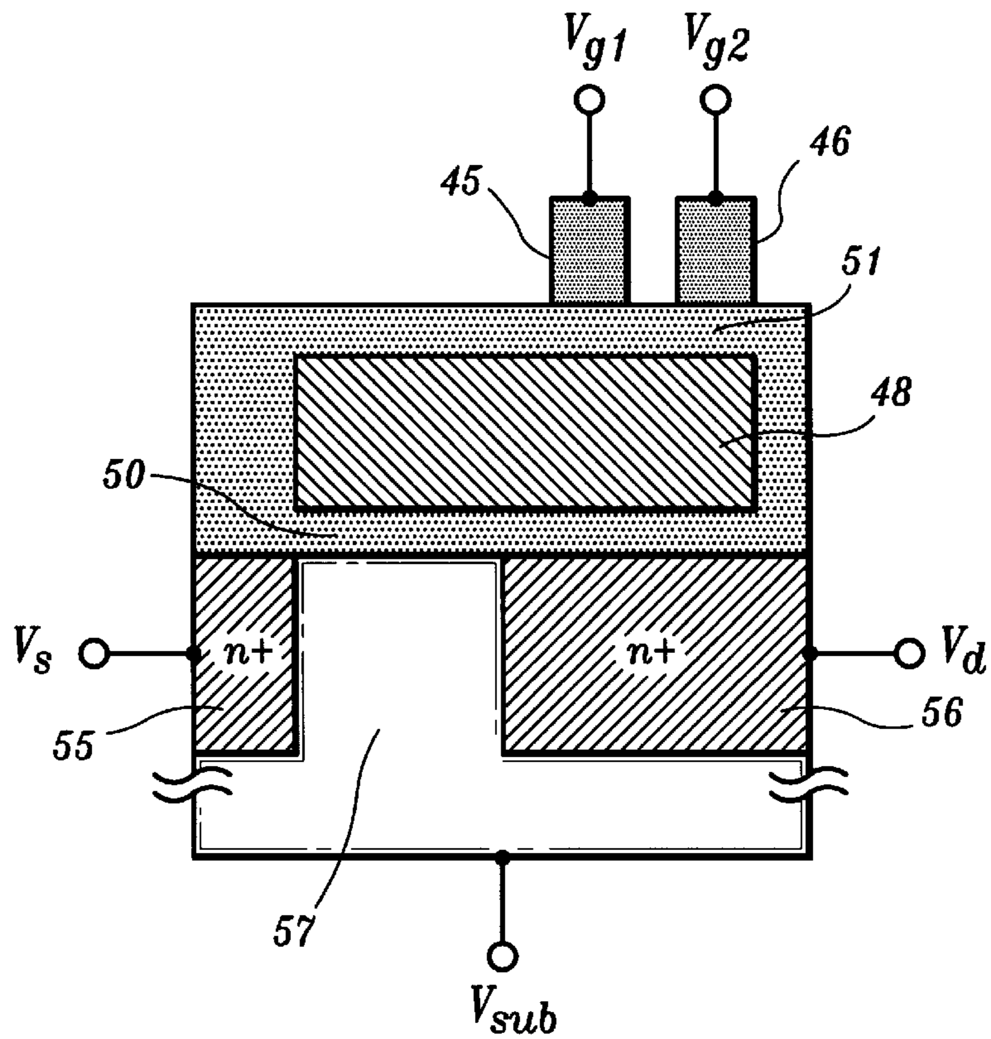
FIG. 24 (PRIOR ART)
