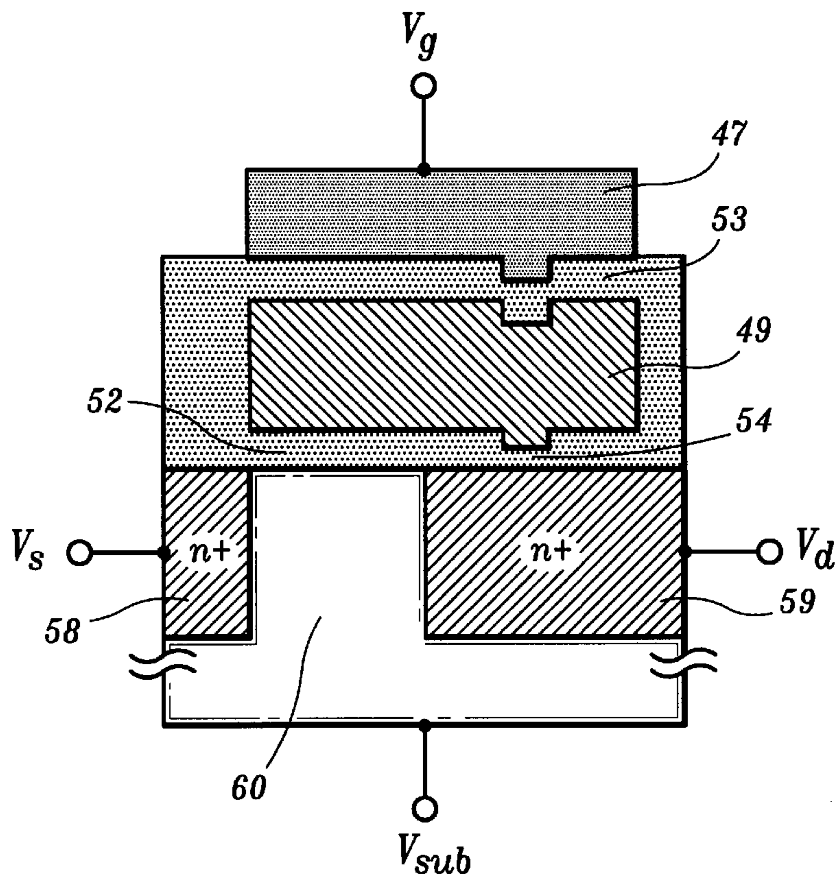
FIG. 29 (PRIOR ART)
