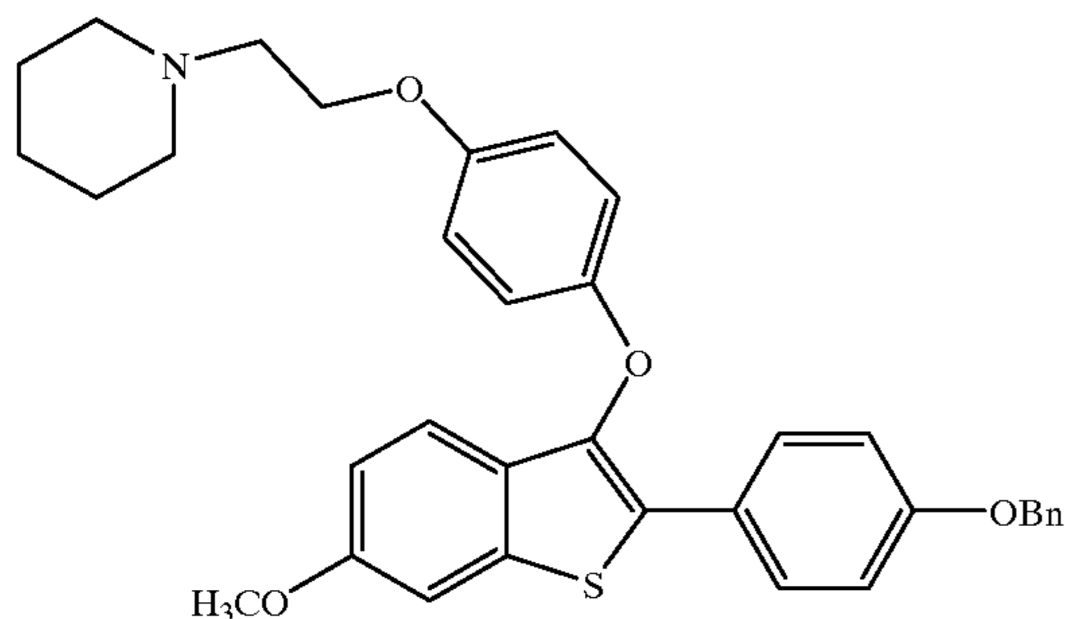
[6-Methoxy-3-(4-[2-(1-piperidinyl)ethoxy]phenoxy)-2-(4-benzyloxyphenyl)]benzo[b]thiophene
