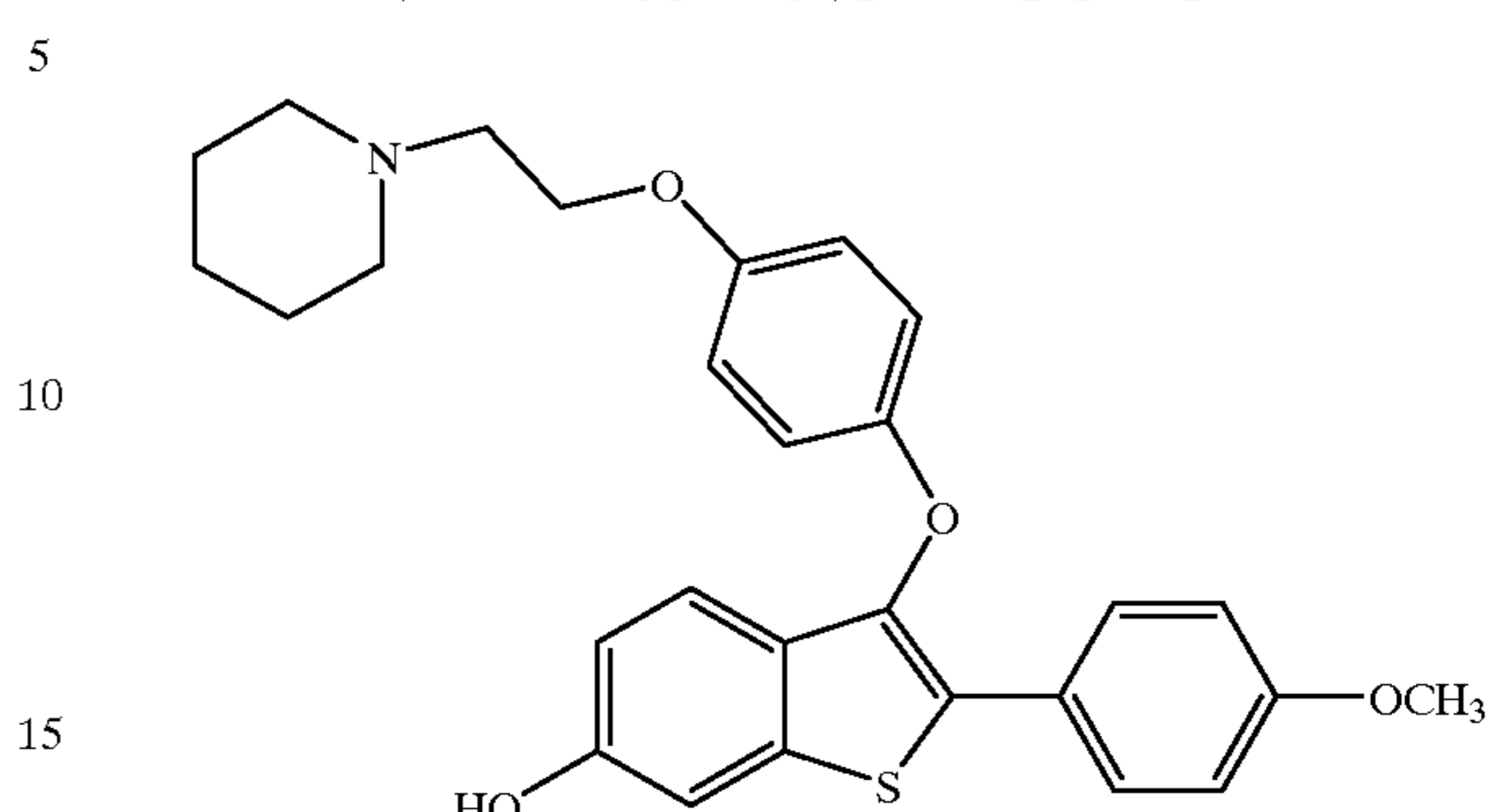
[6-Hydroxy-3-[4-[2-(1-piperidinyl)ethoxy]phenoxy]-2-(4-methoxyphenyl)]benzo[b]thiophene
