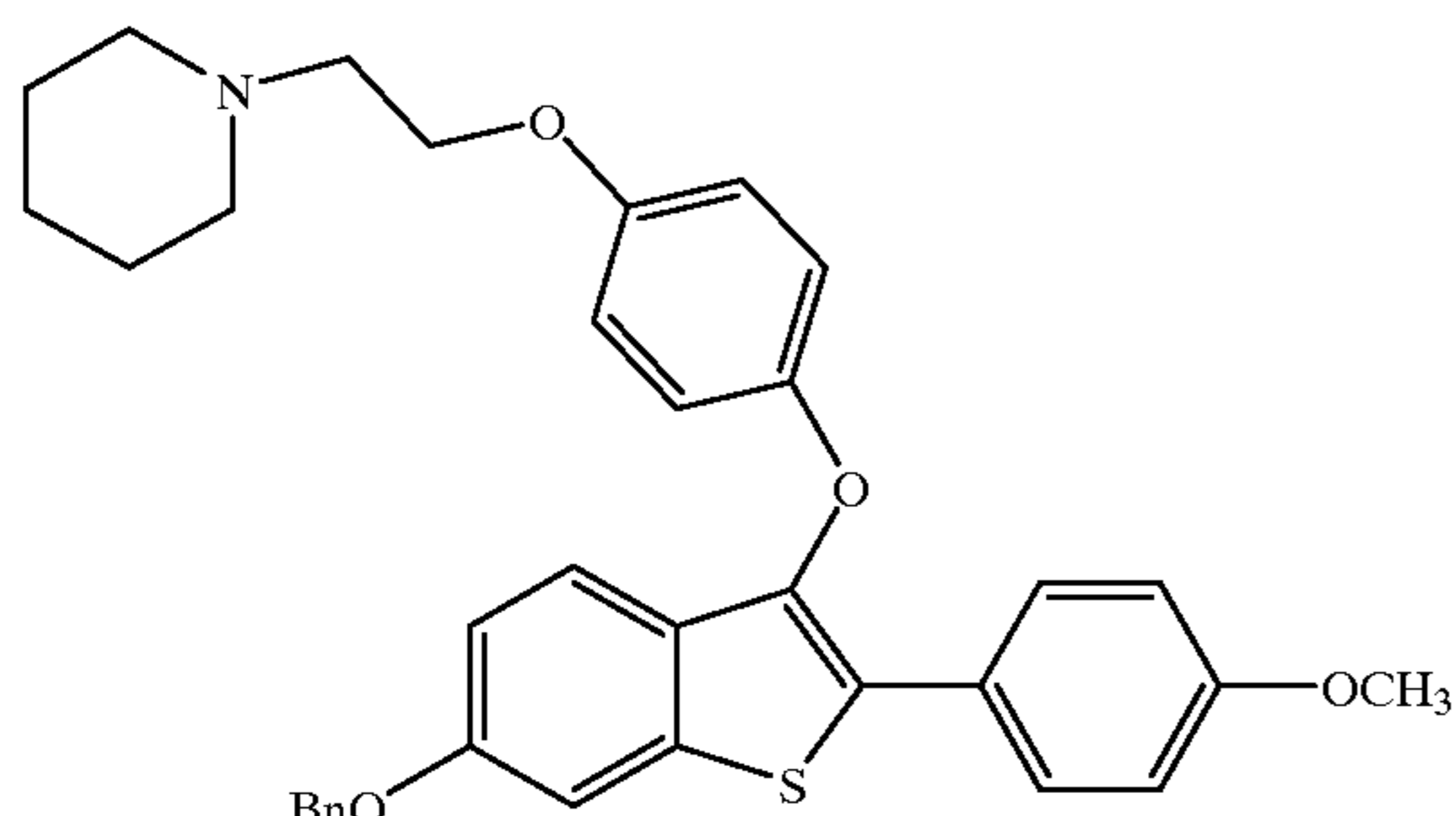
[6-Benzyloxy-3-[4-[2-(1-piperidinyl)ethoxy]phenoxy]-2-(4-methoxyphenyl)]benzo[b]thiophene
