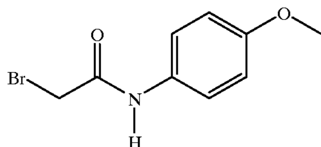
Bromo-N-(4-methoxyphenyl)acetamide
