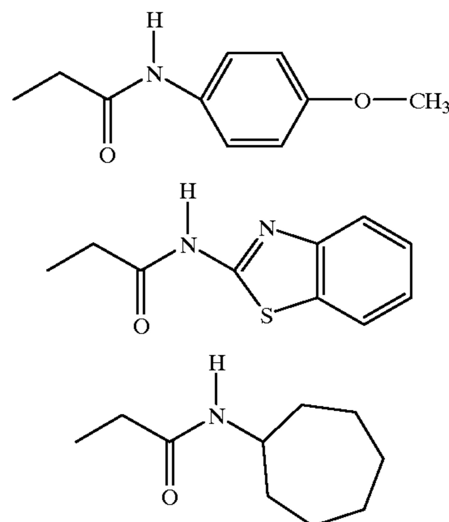
Compounds 155-160
