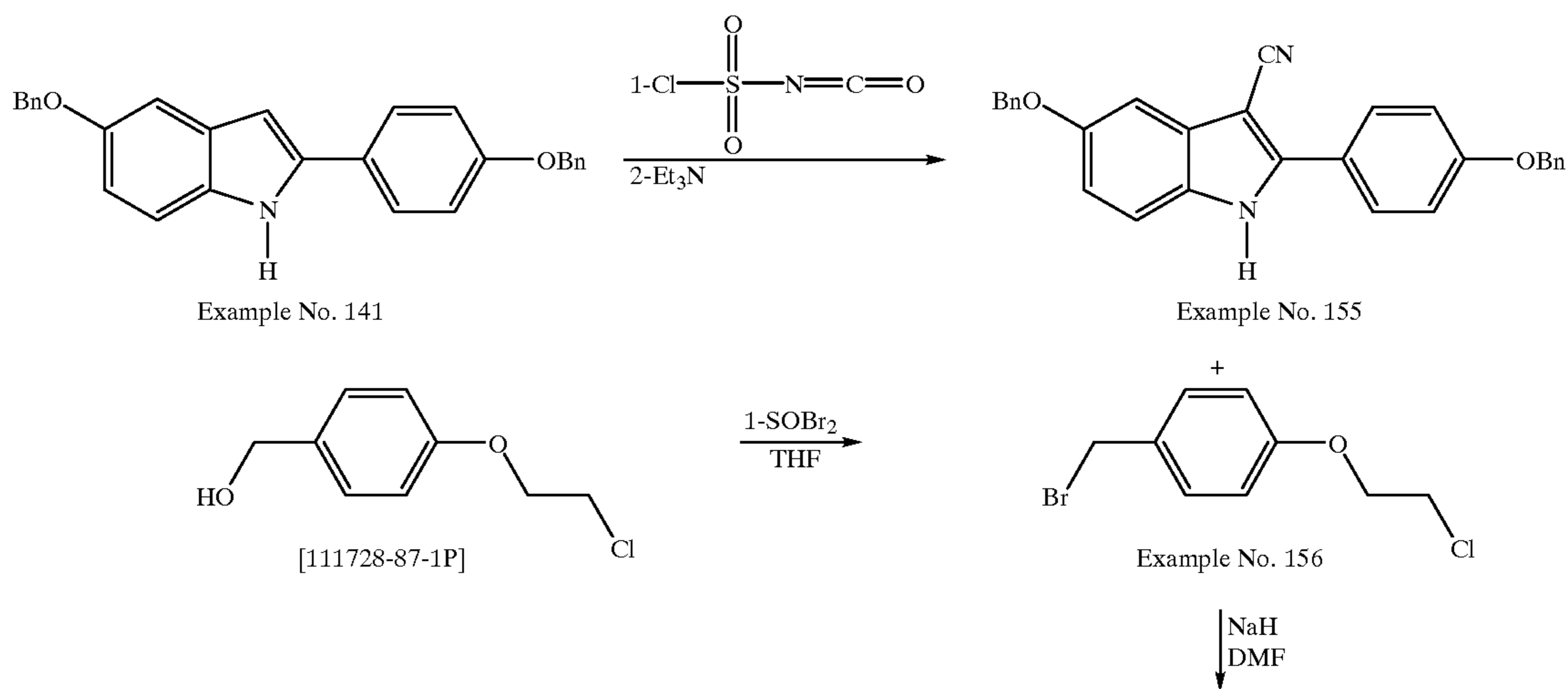
Scheme 7
