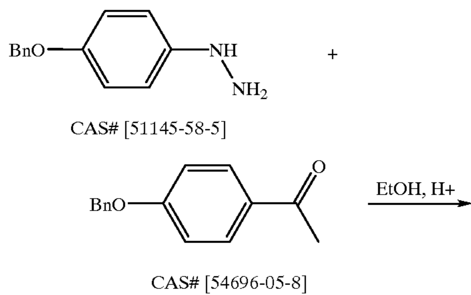
Scheme 5
