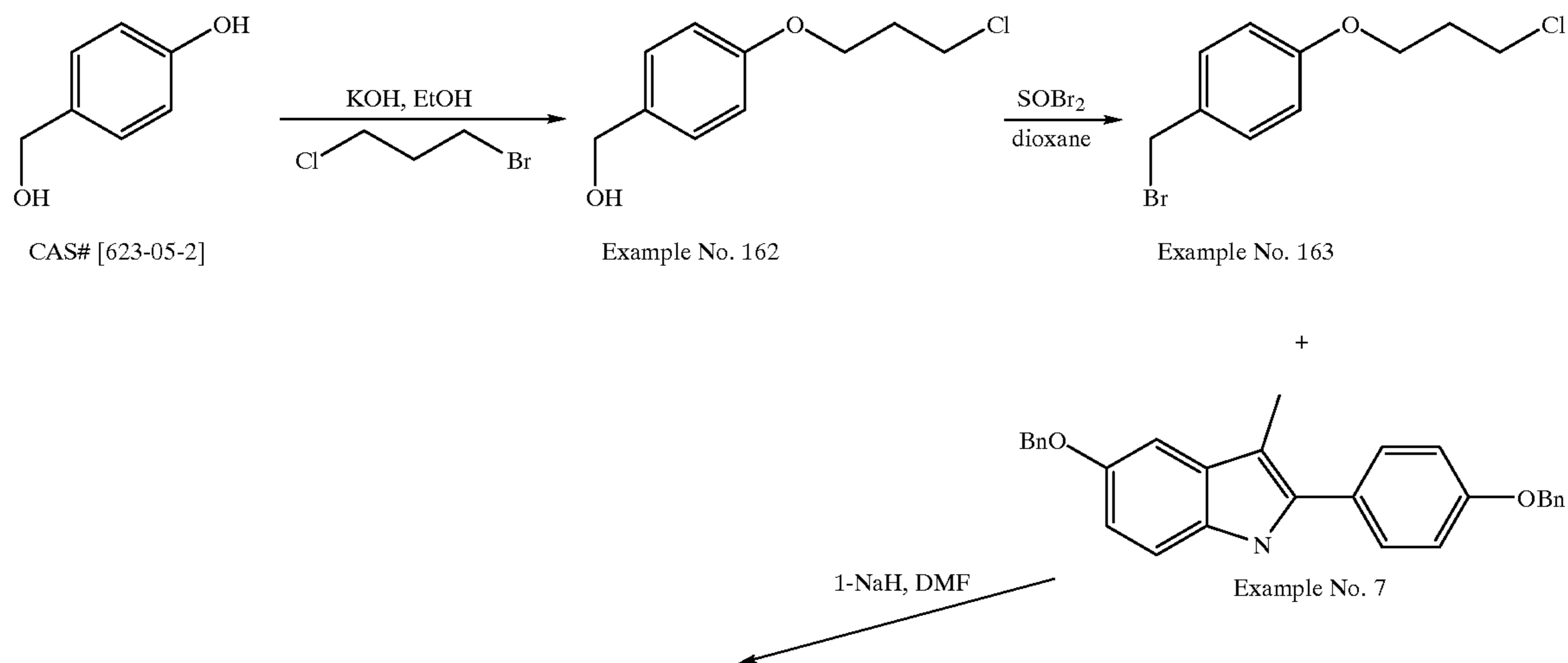
Scheme 4
