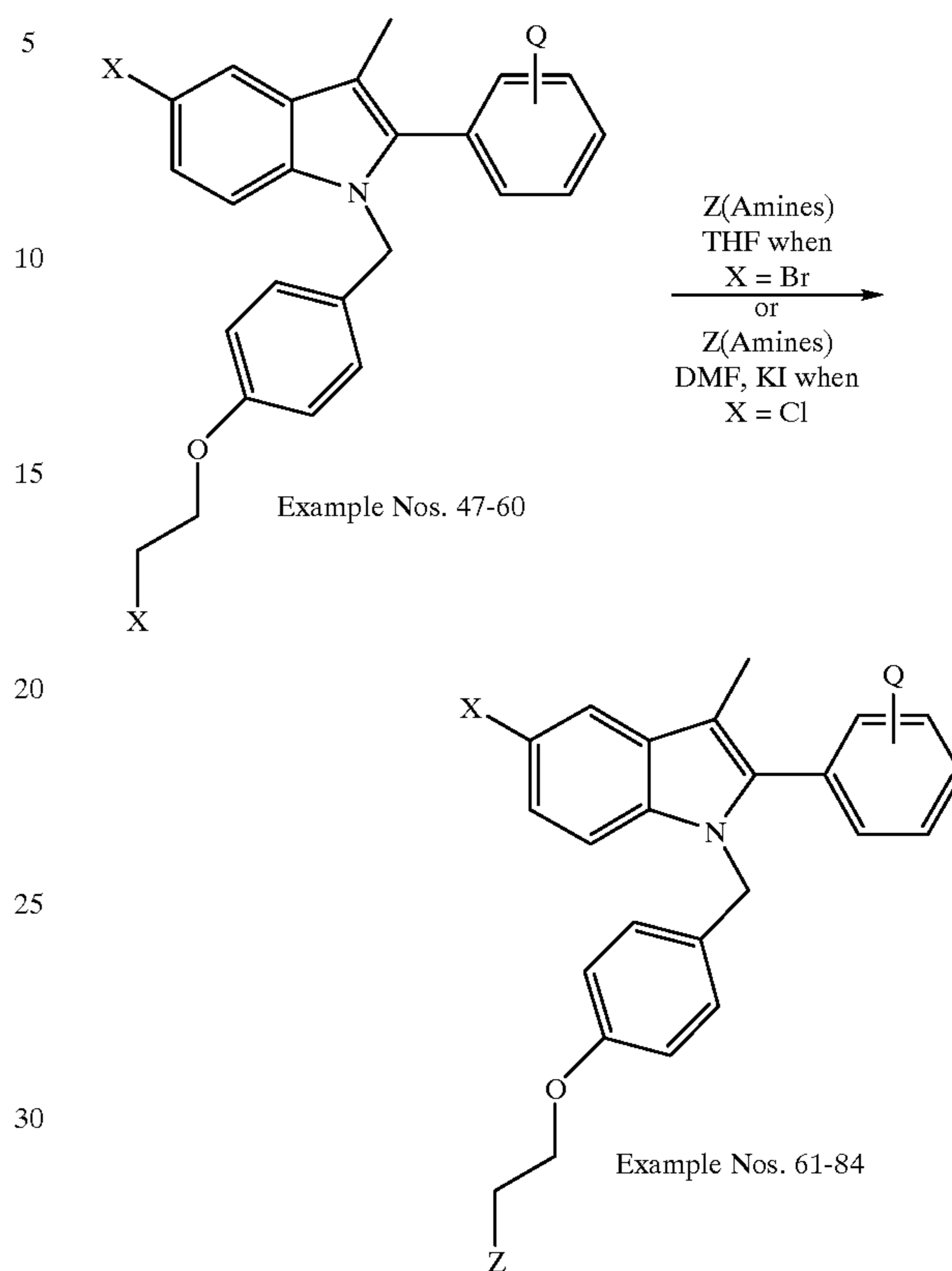
Scheme 13
