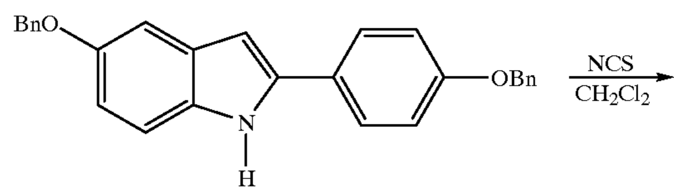
Example No. 141
