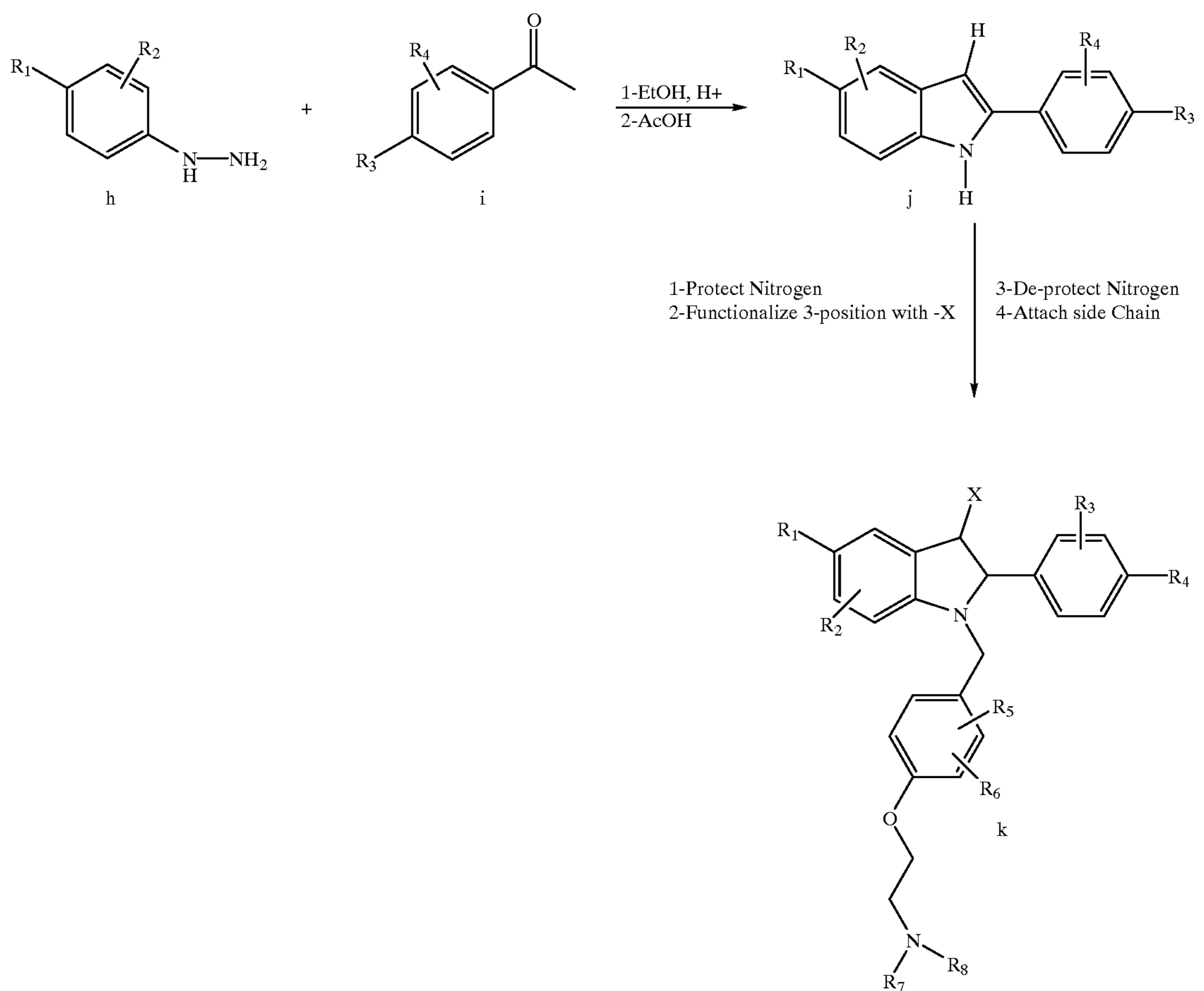
Scheme 2
