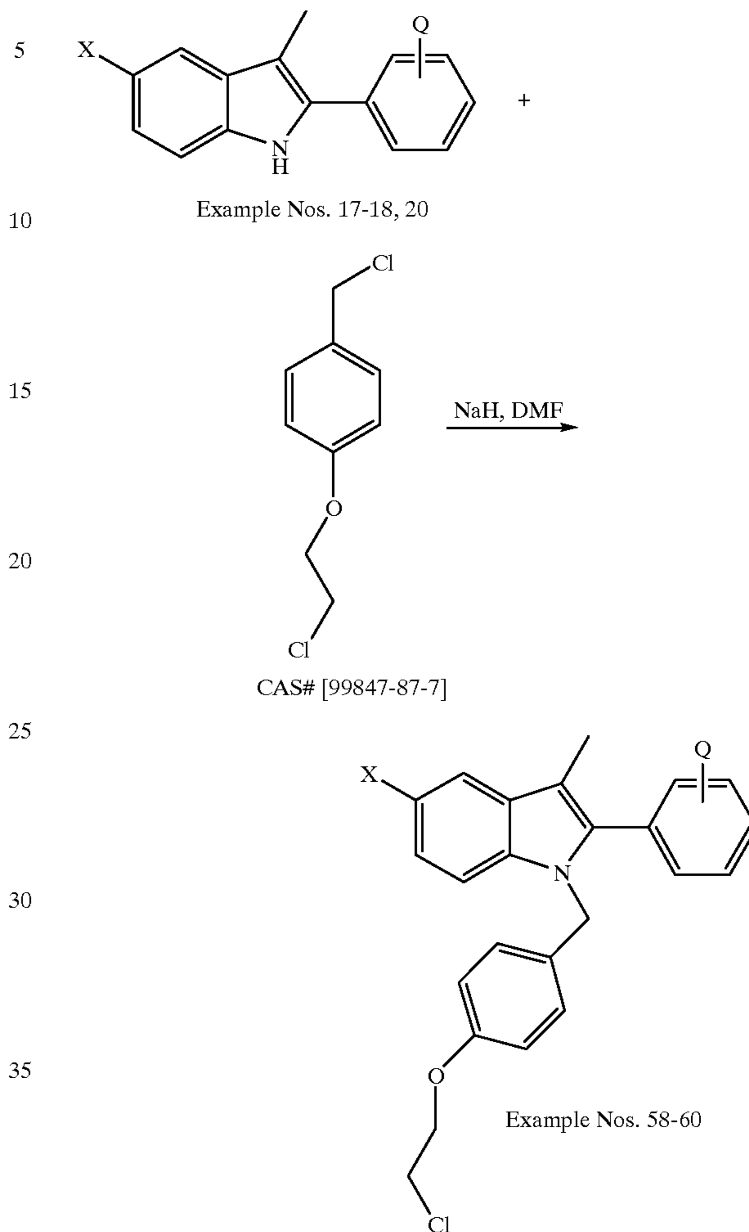
Scheme 12
