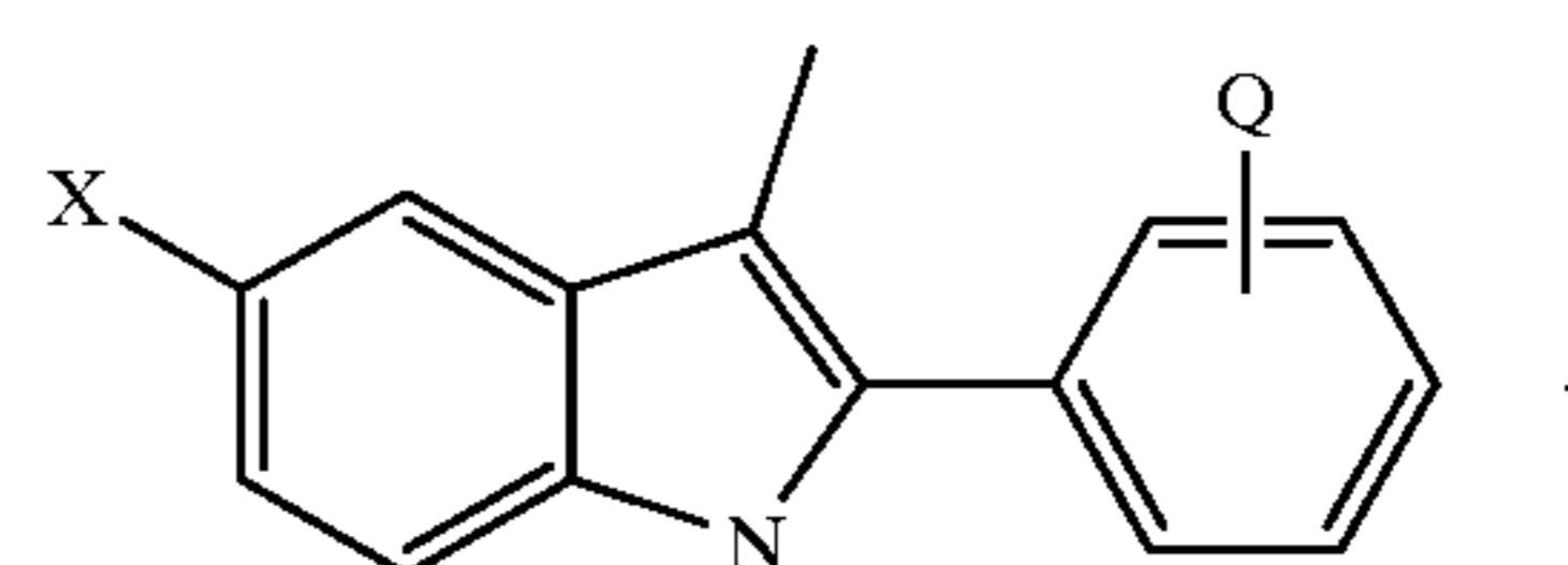
Scheme 9
