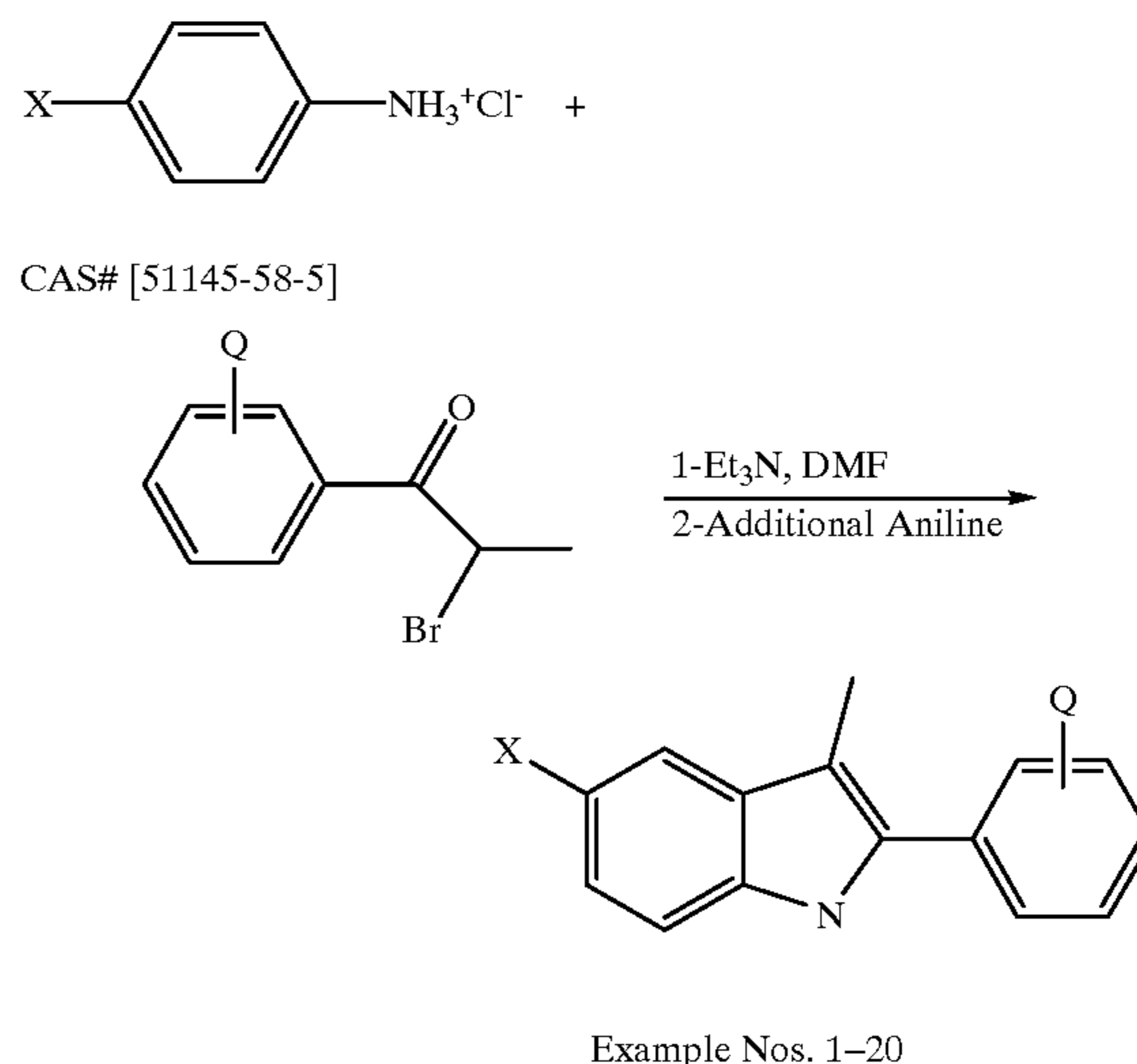
Scheme 8
