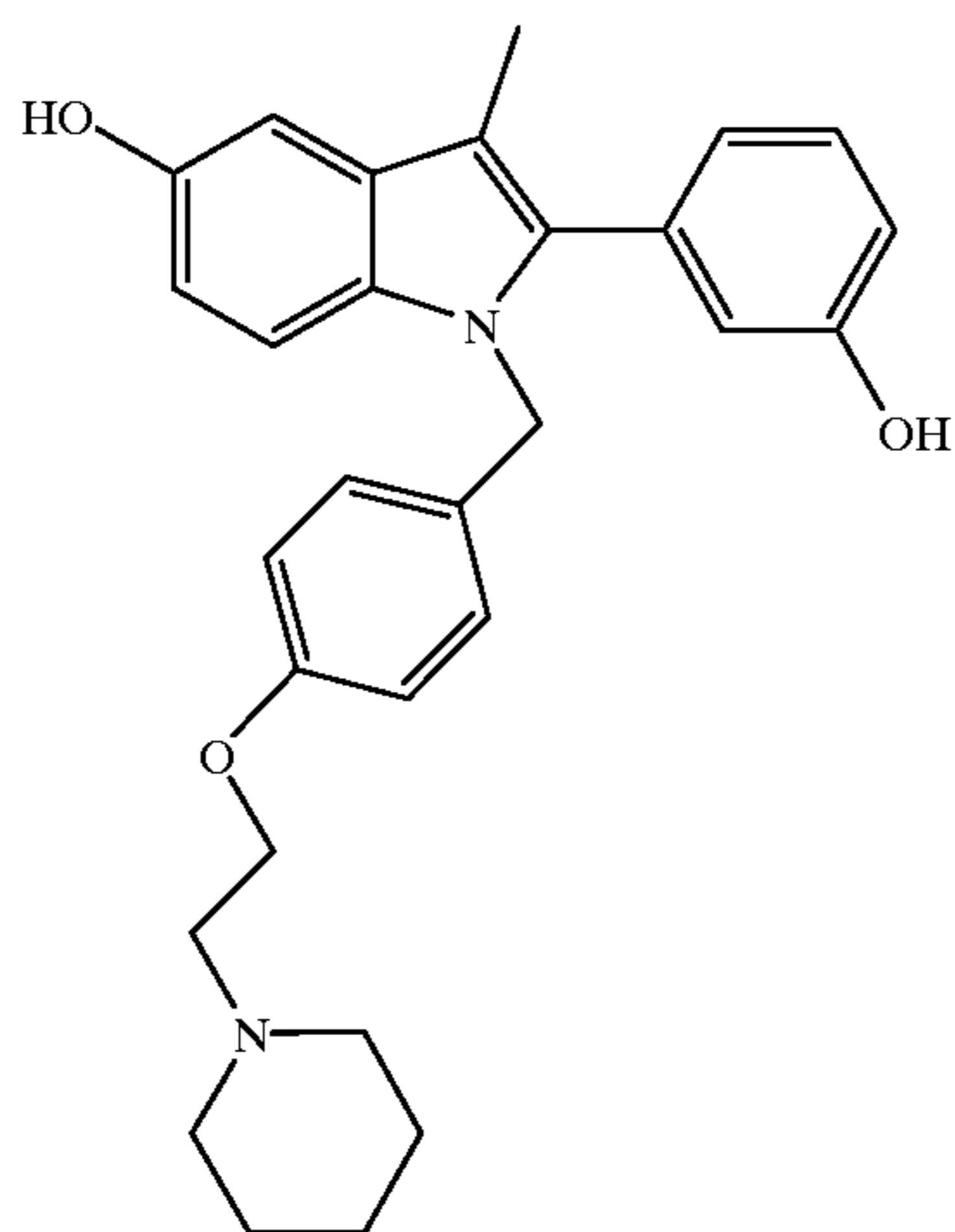
Example No. 127
