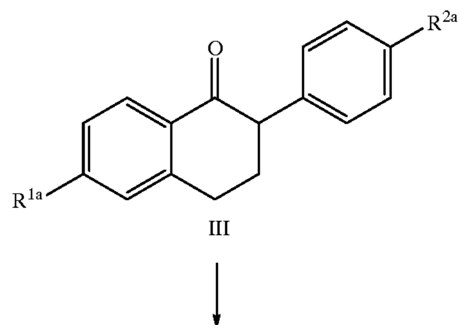
Scheme I
