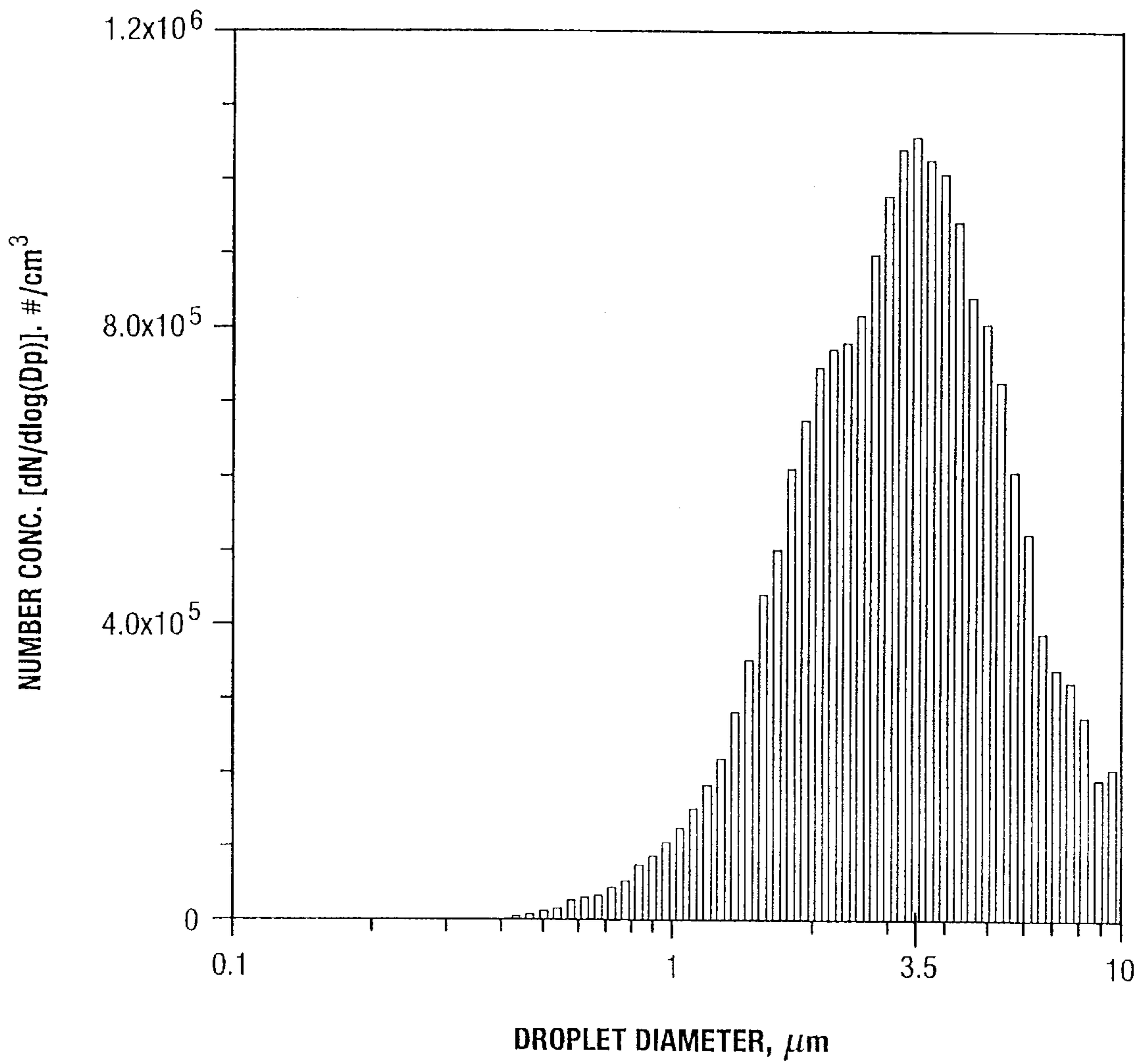
FIG. 19 (PRIOR ART)
