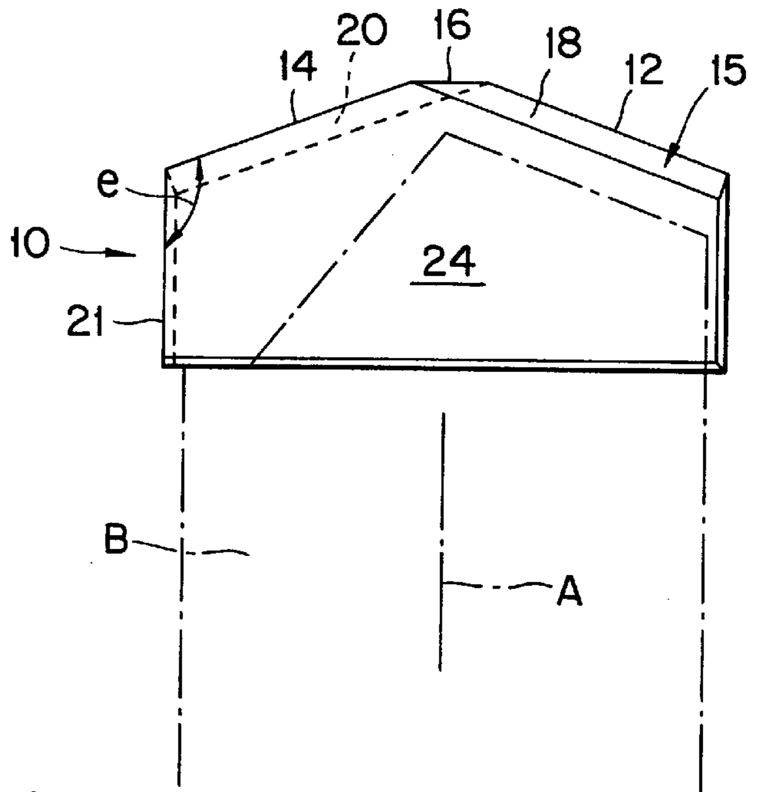
FIG. 2 (PRIOR ART)
