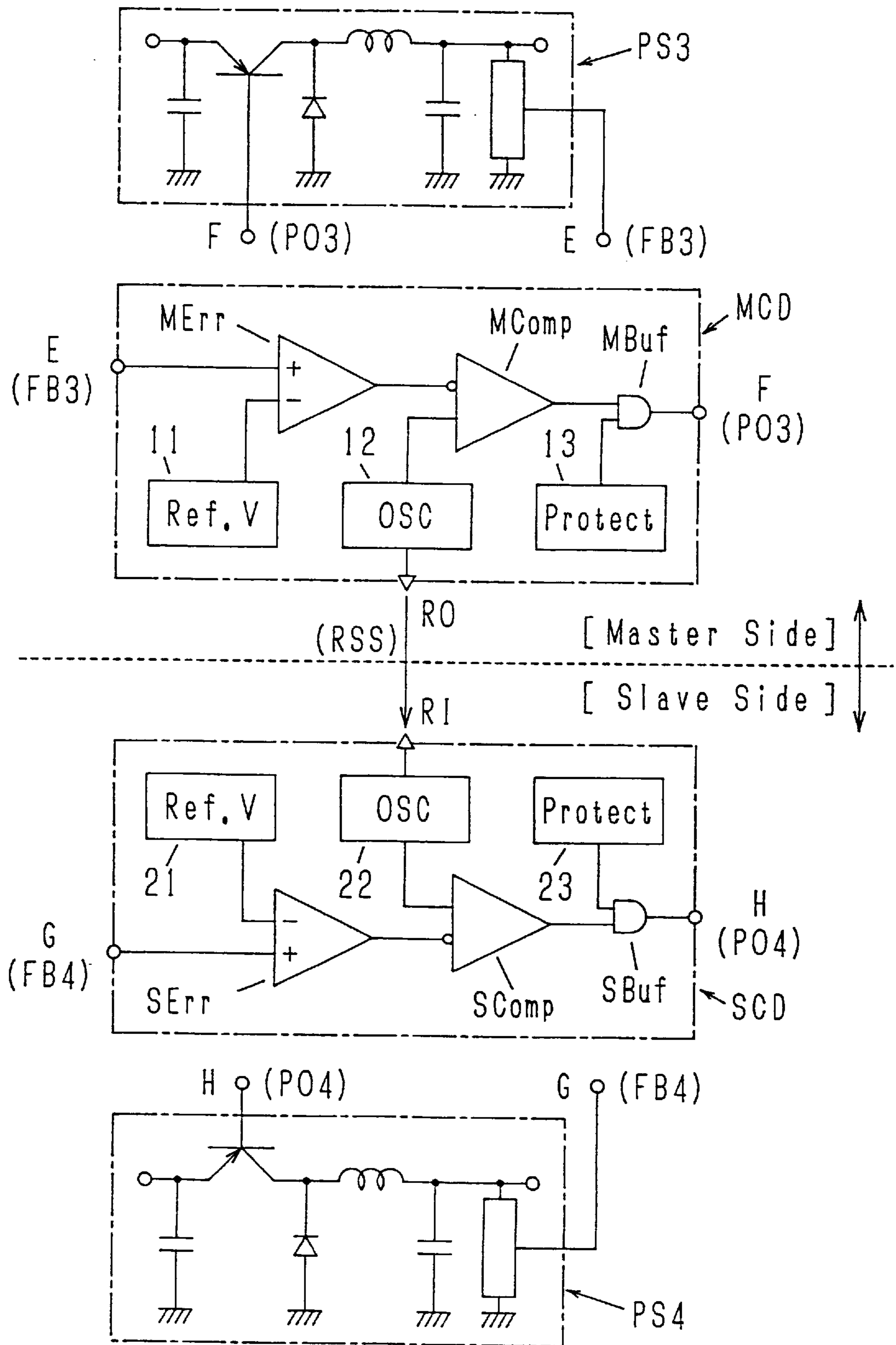
FIG. 2 (PRIOR ART)
