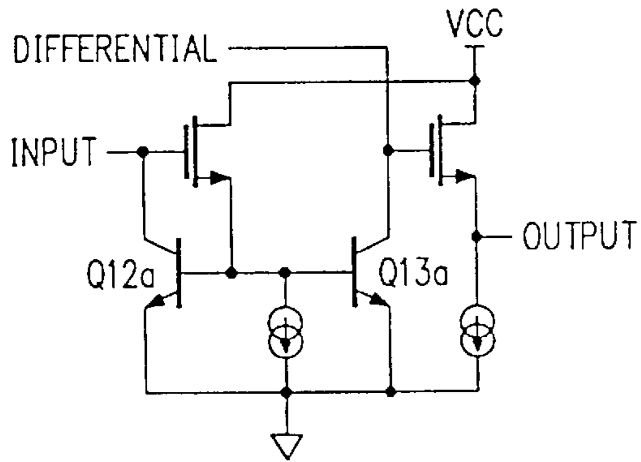
FIG. 34 (PRIOR ART)
