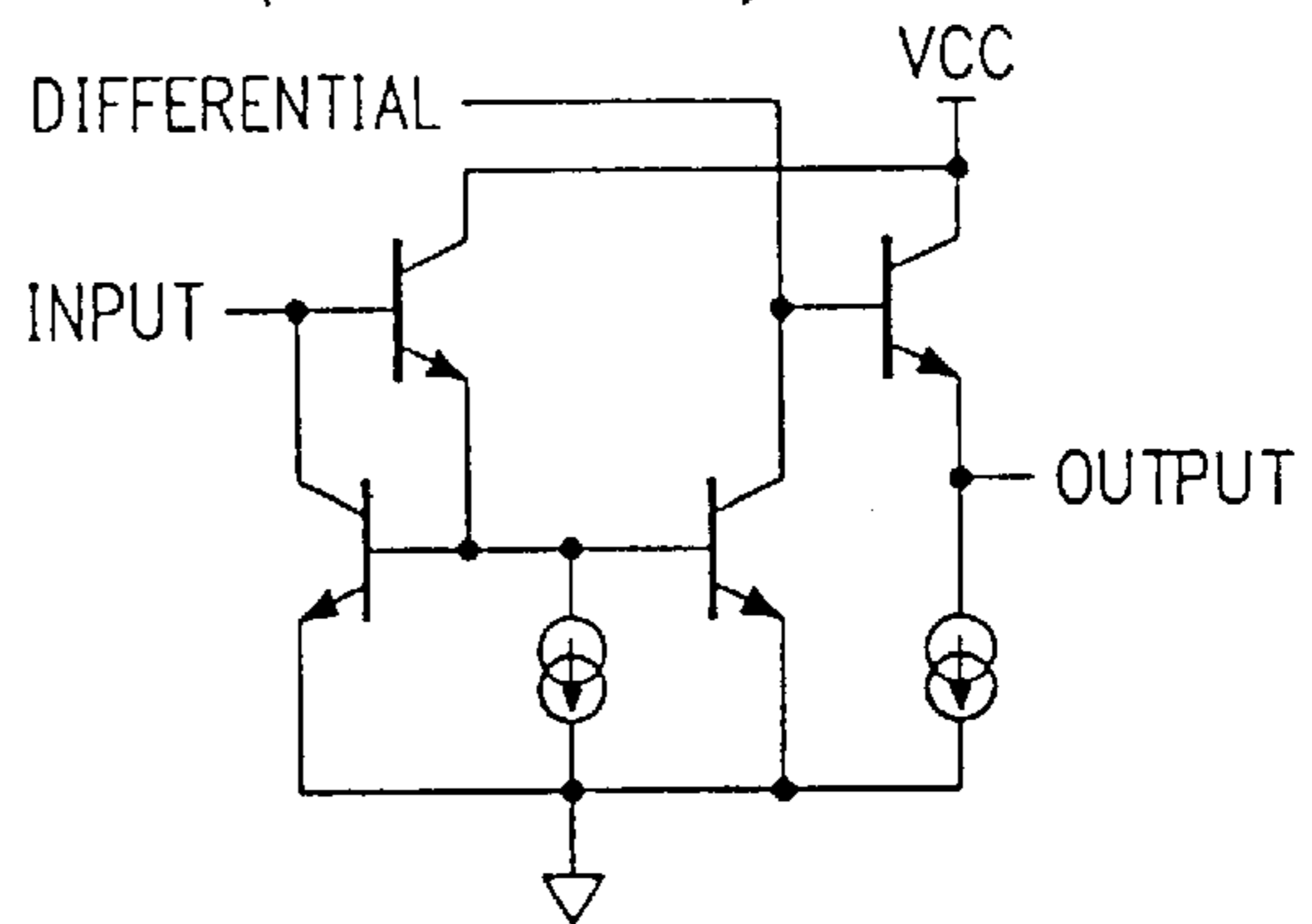
FIG. 35 (PRIOR ART)
