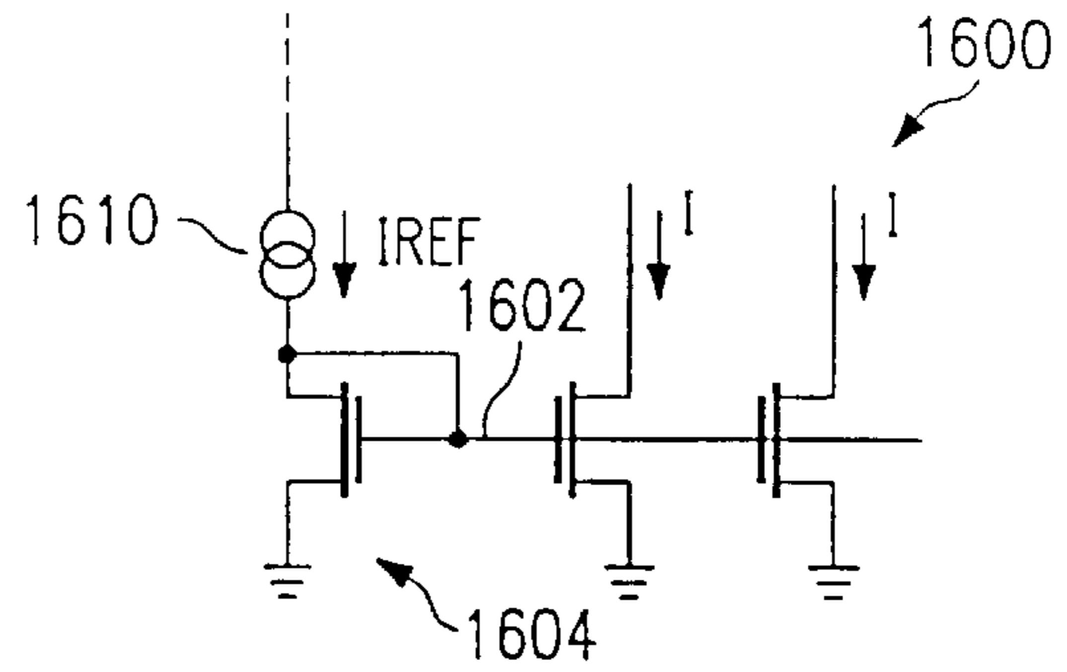
FIG. 16 (PRIOR ART)
