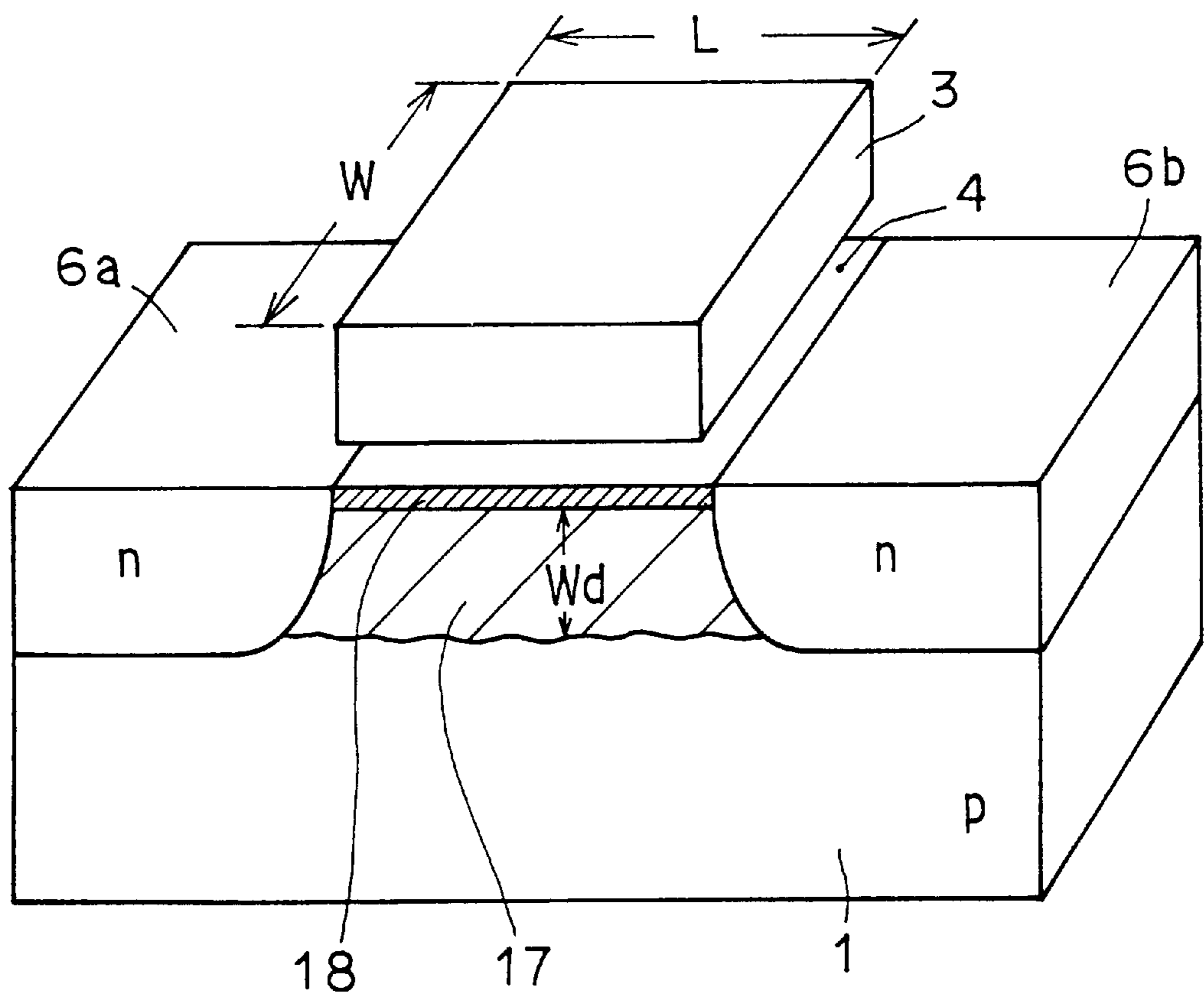
FIG. 101 PRIOR ART
