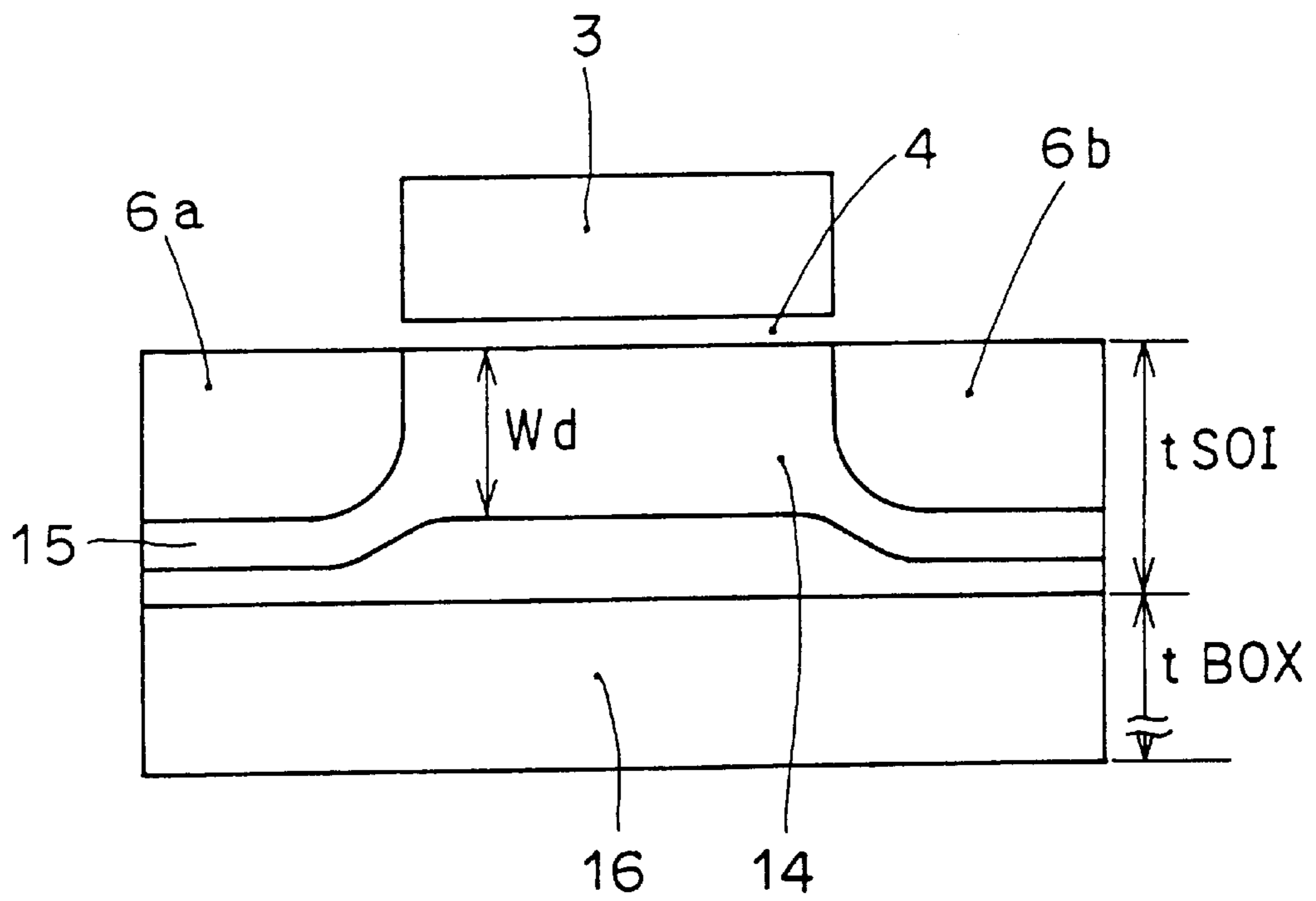
FIG. 104 PRIOR ART
