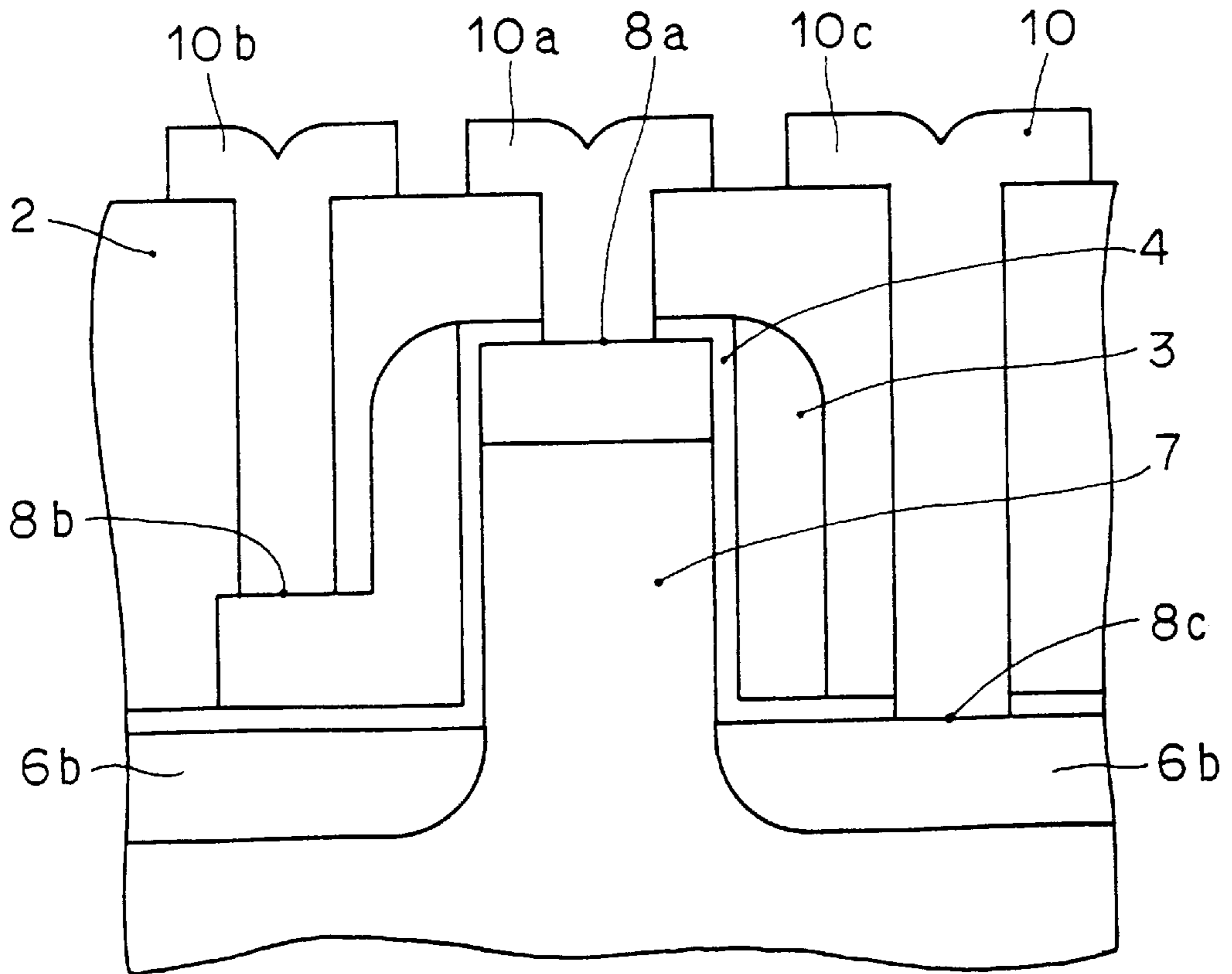
FIG. 110 PRIOR ART
