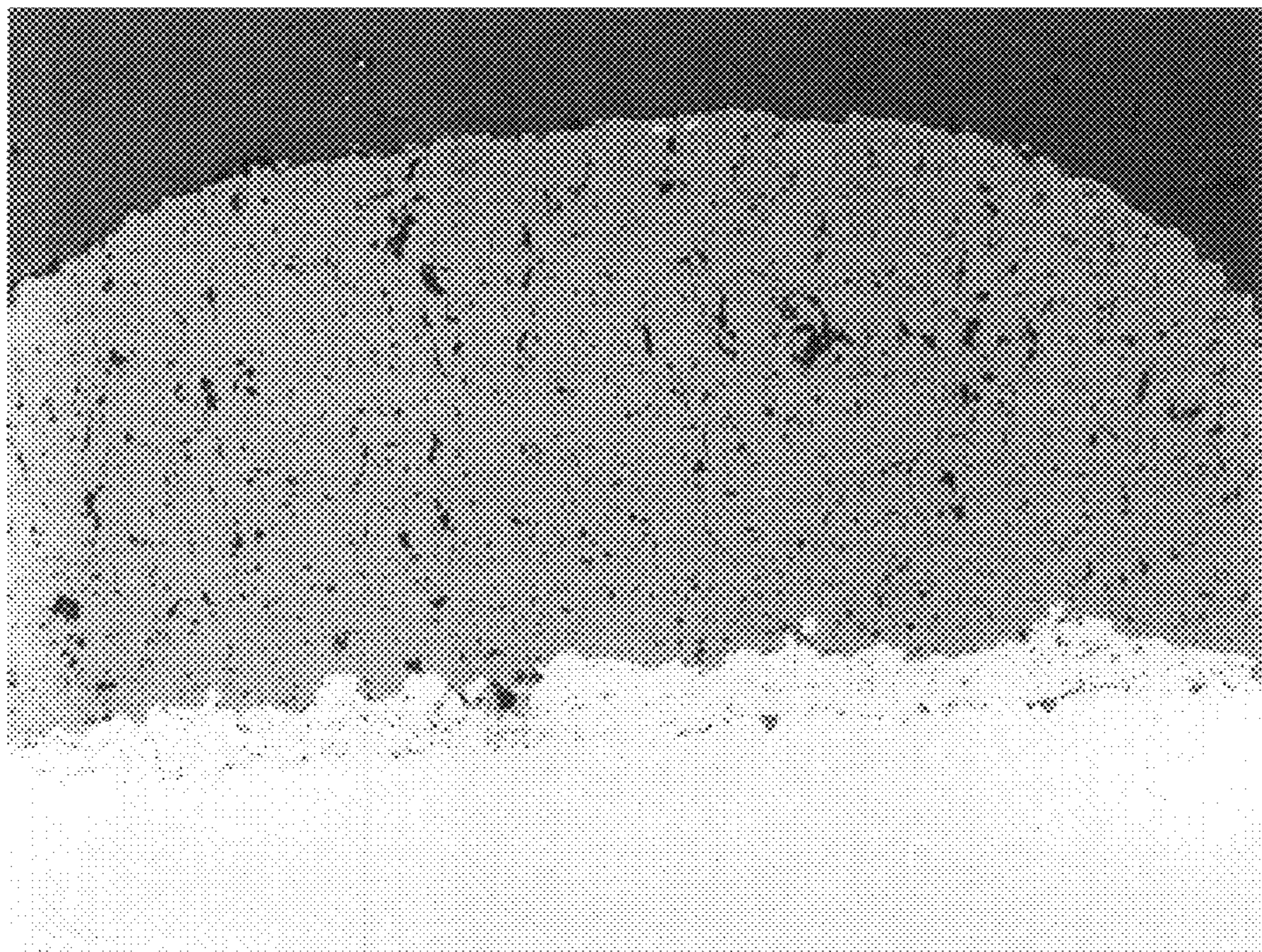
A31(2) X100 Panel: As Sprayed
