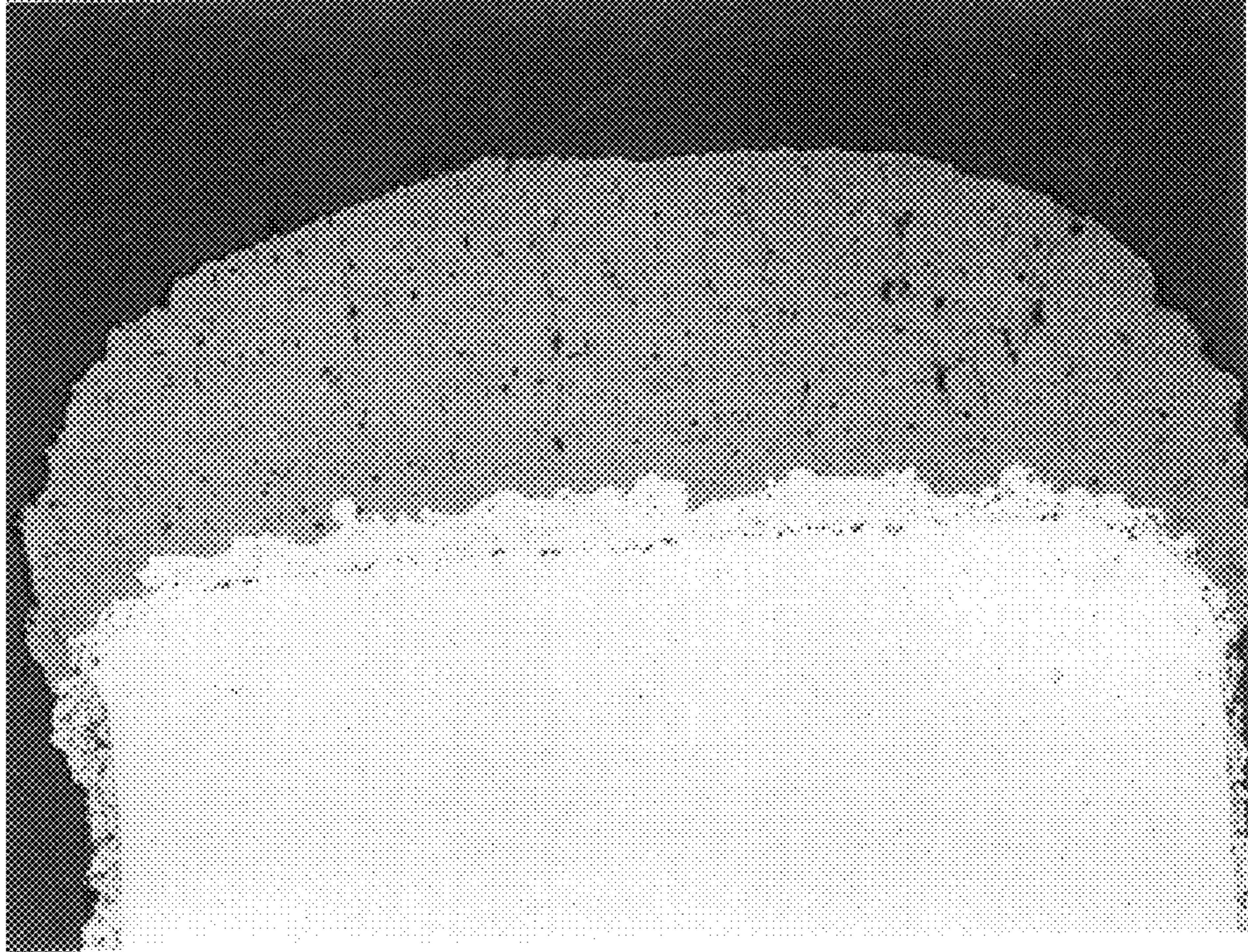
A31(2) X75 Blade: As Sprayed
