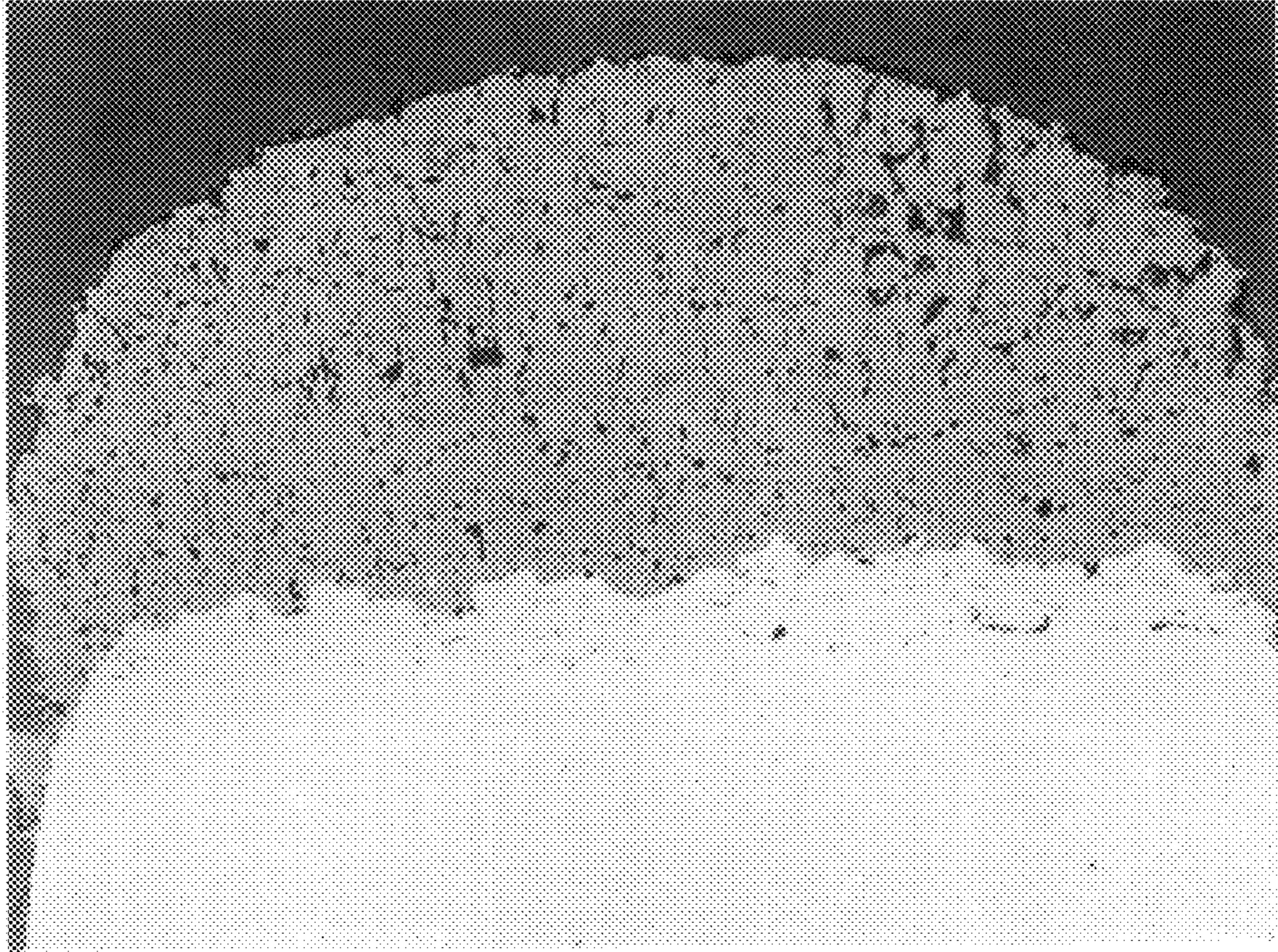
A31(1) X100 Panel: As Sprayed
