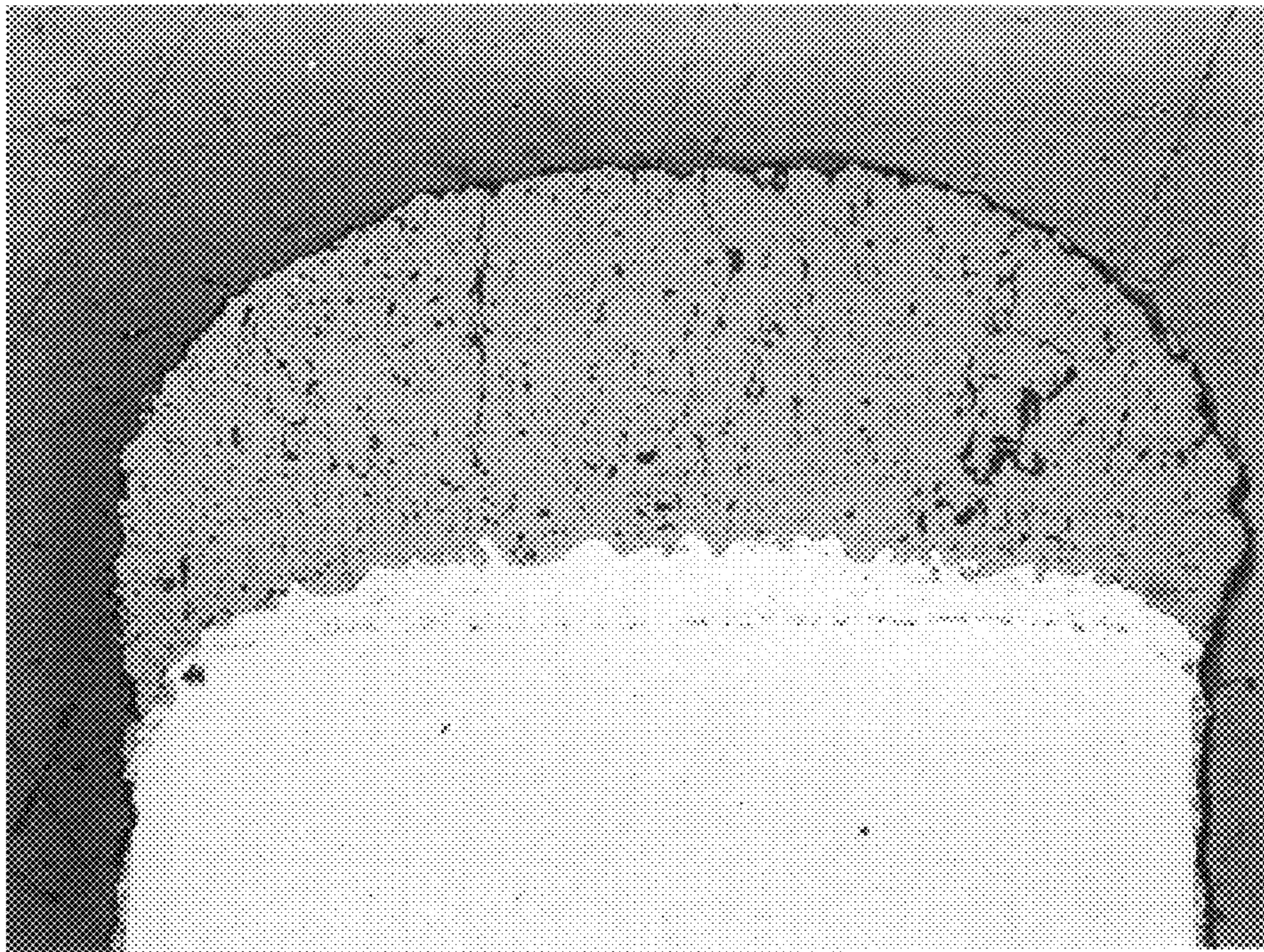
A31(2) X75 Blade: As Tested
