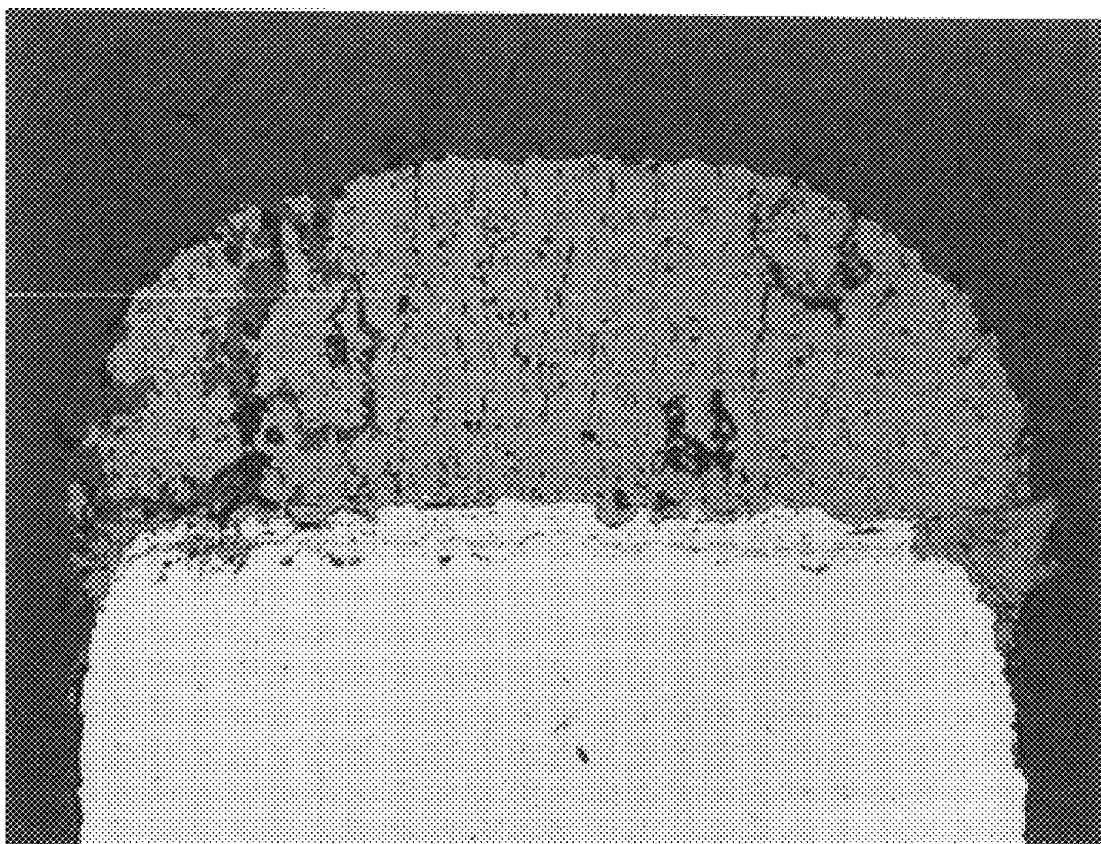
A31(2) X75 Panel: As Tested
