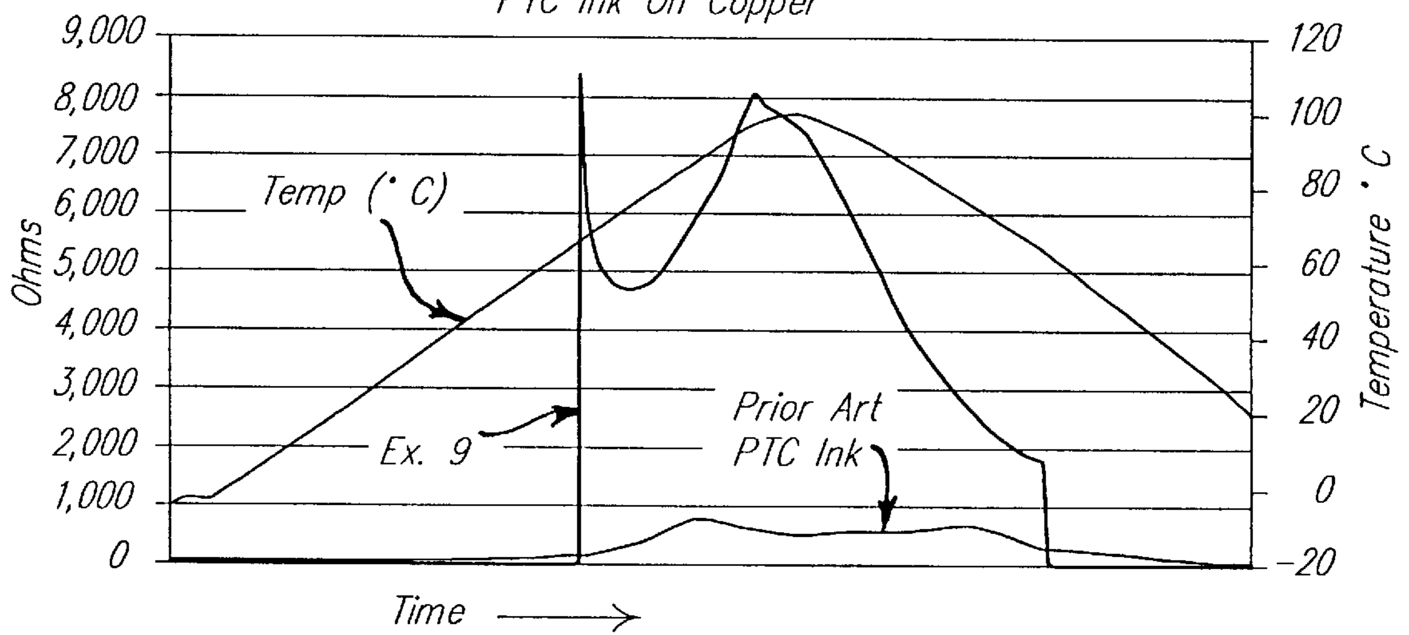
Comparison Of Example 9 Ink And Prior Art Commercial PTC Ink PTC Ink On Copper
