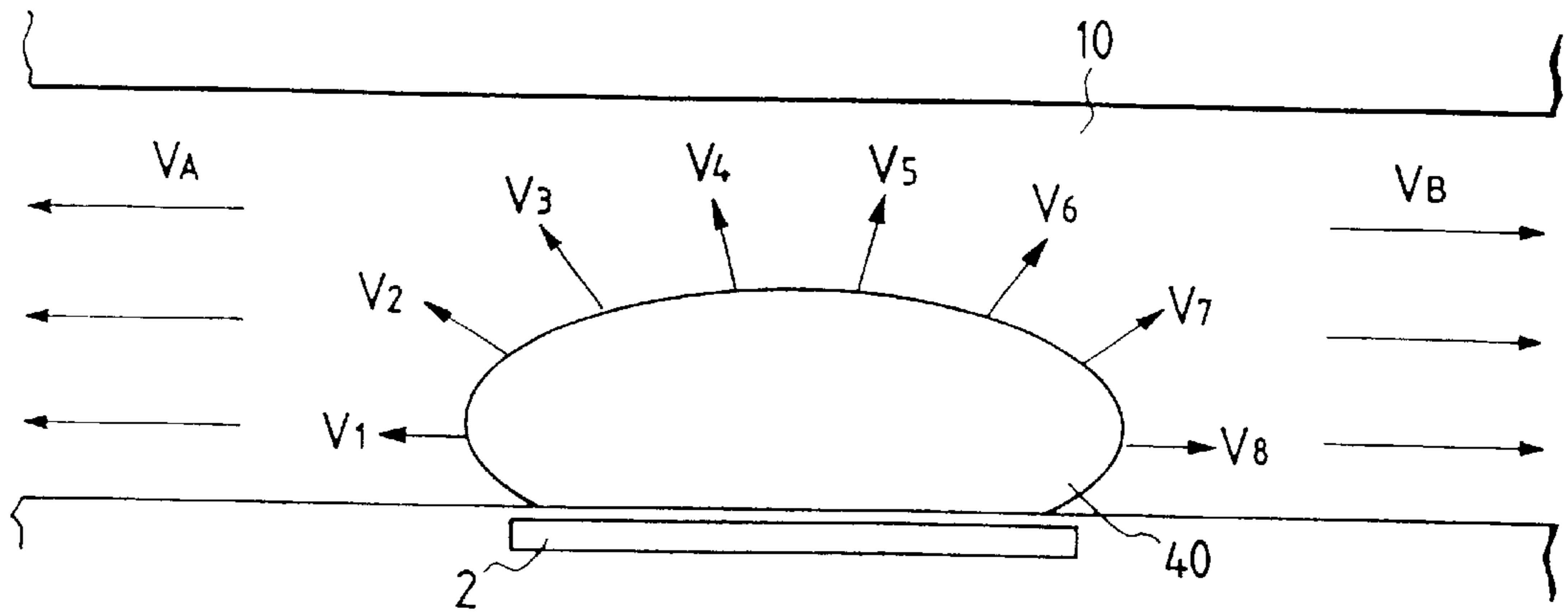
FIG. 3 PRIOR ART
