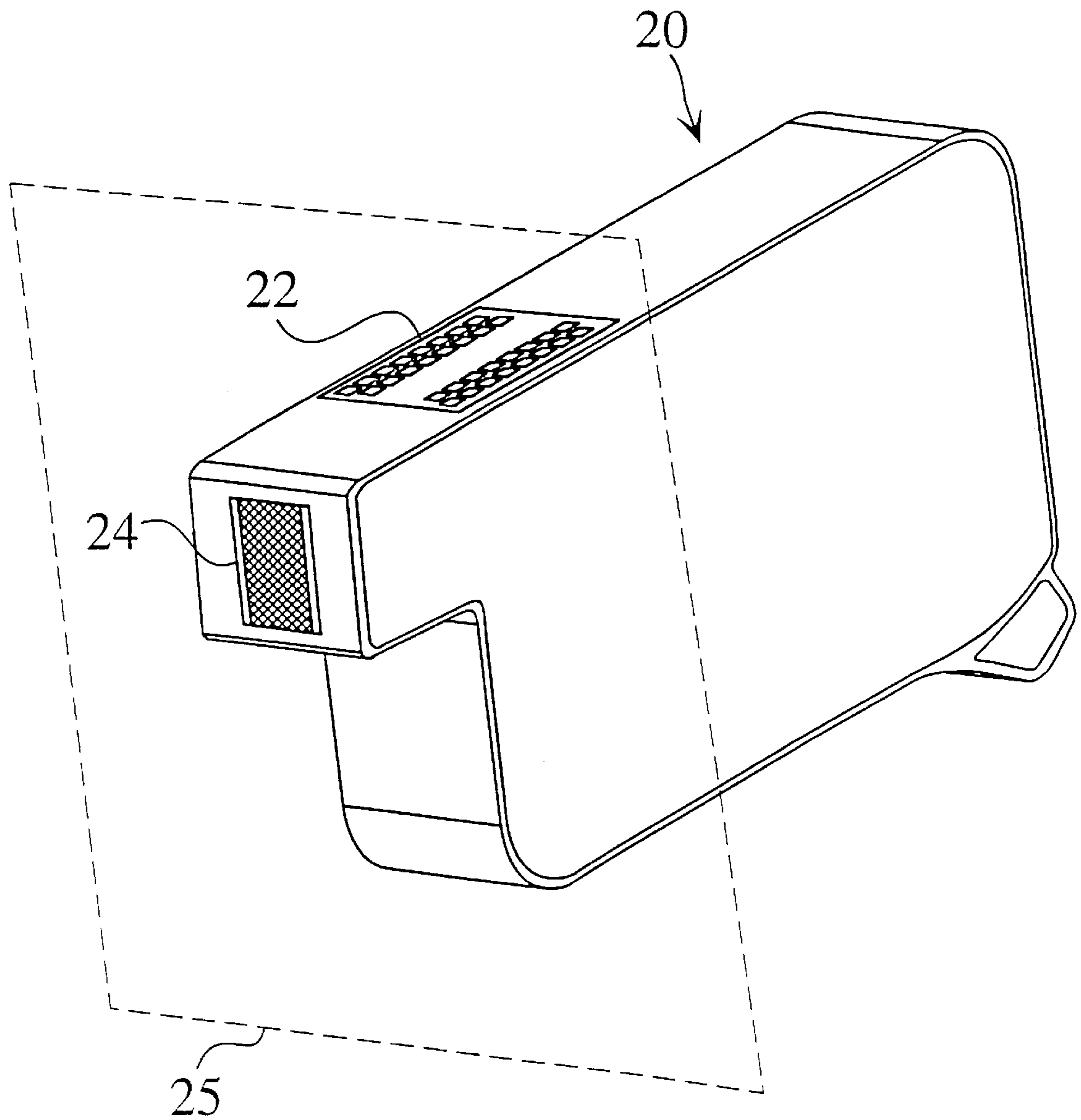
Fig. 2 (PRIOR ART)
