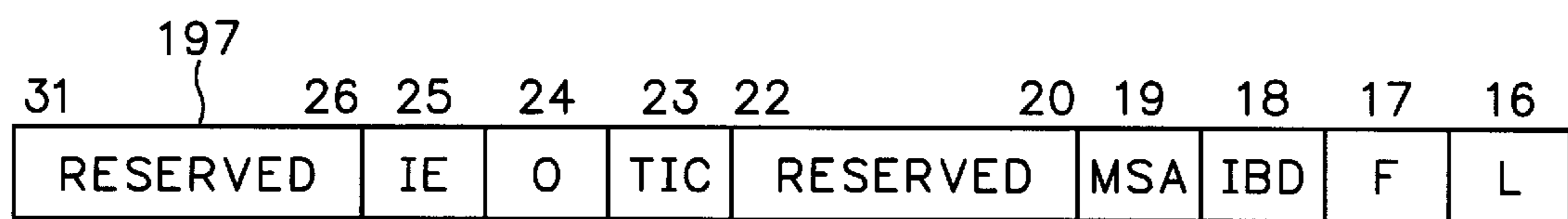
DMA CONTROL & STATUS FIELD OF DESCRIPTOR
