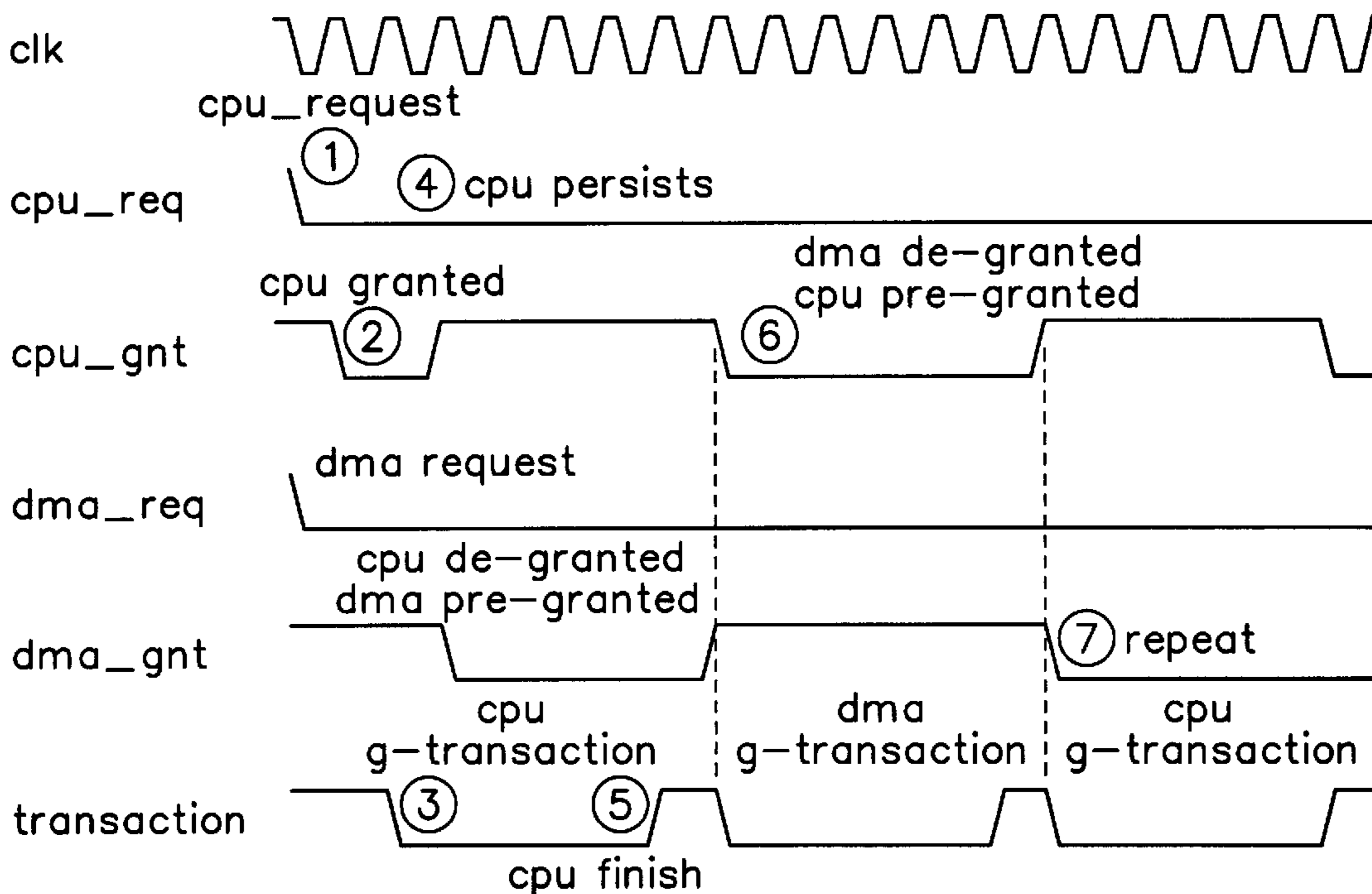
PIPELINE ARBITRATION PROTOCOL EXAMPLE
