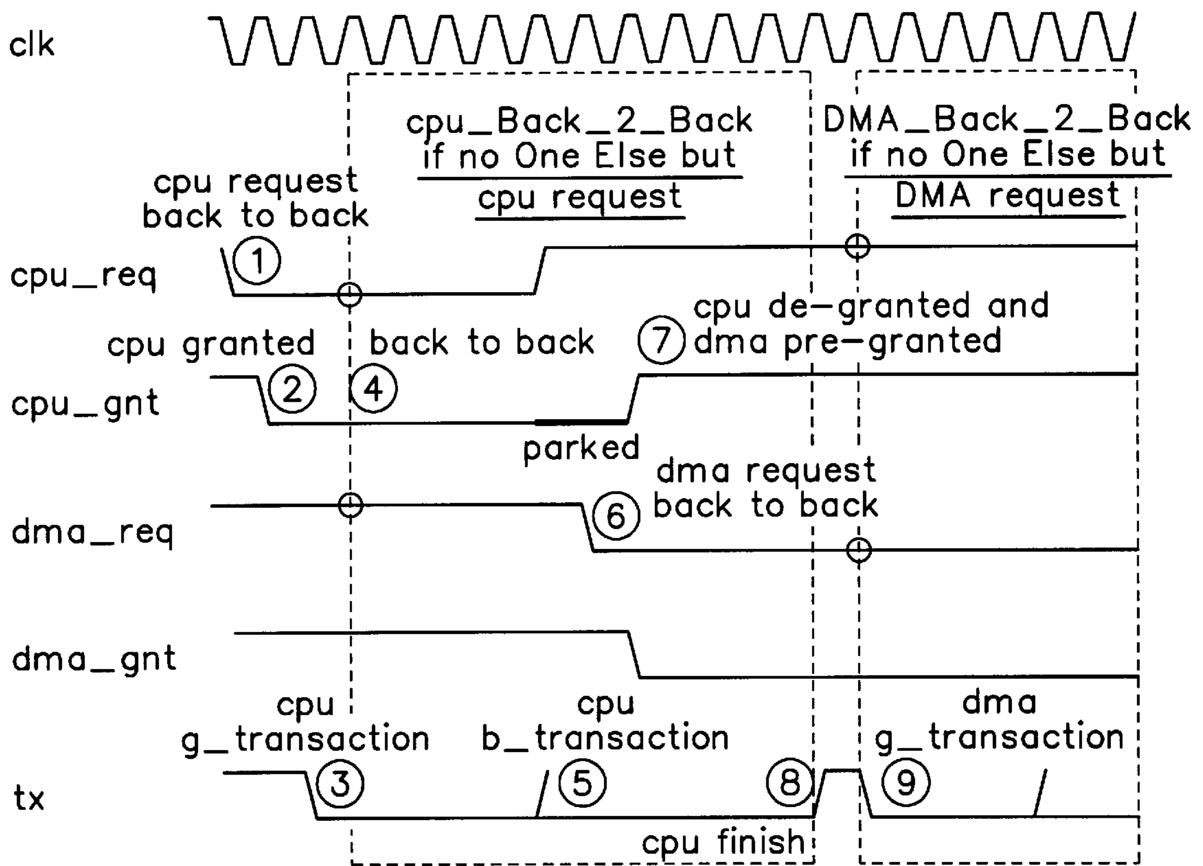
ARBITRATION PROTOCOL EXAMPLE BACK-TO-BACK TRANSACTION
