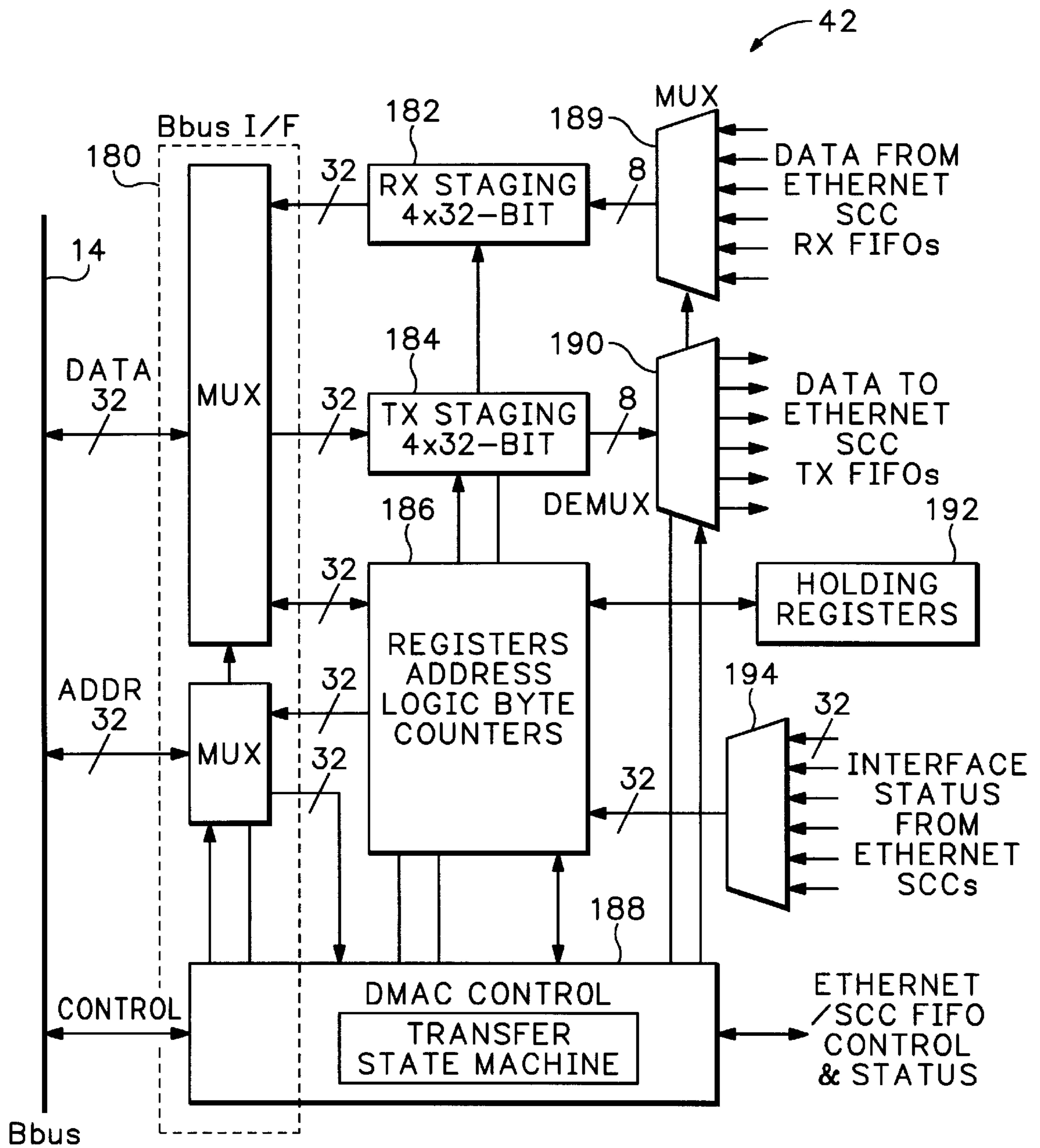
DMAC BLOCK DIAGRAM
