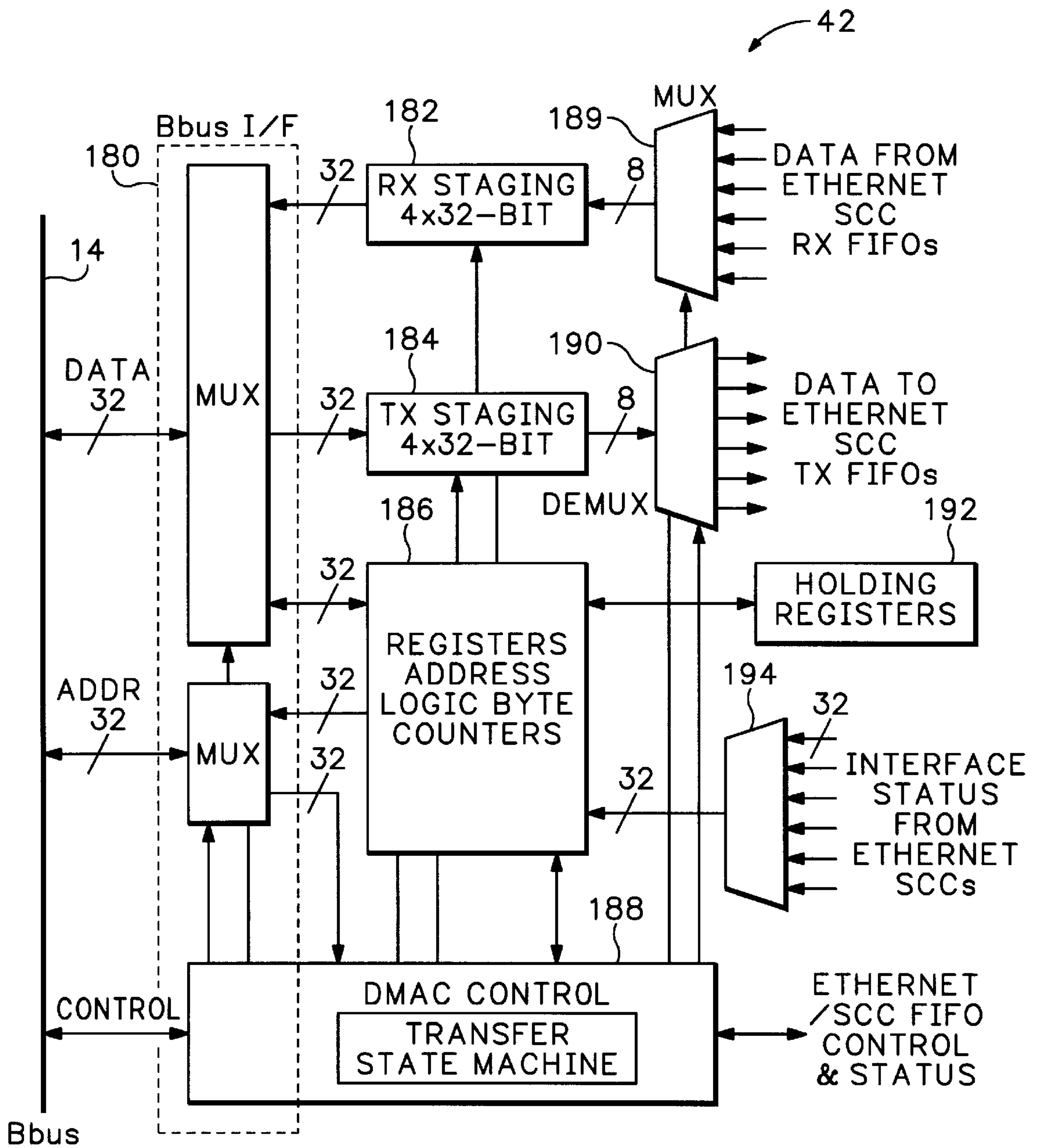
DMAC BLOCK DIAGRAM
