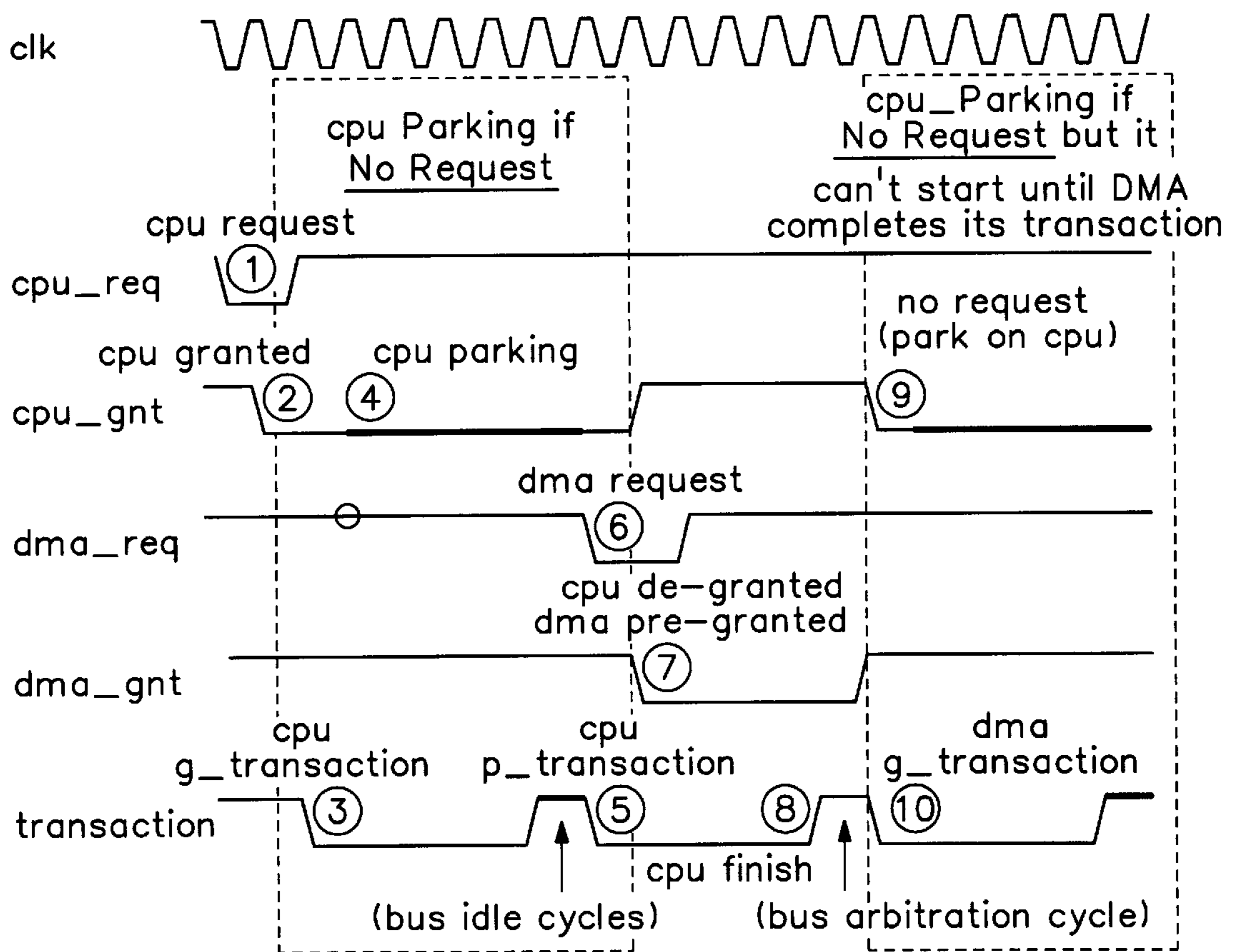
ARBITRATION PROTOCOL EXAMPLE PARKING
