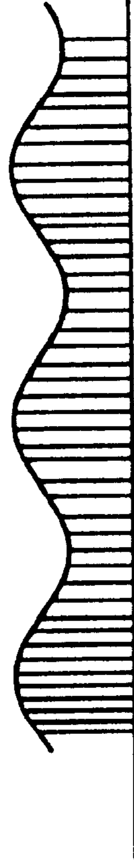
Fig. 120(c) DRIVE CIRCUIT OUTPUT
